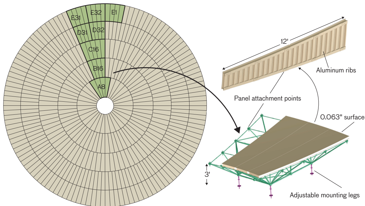
FIGURE 38. The primary reflector with one of each ring type is highlighted. The breakout images show a subframe assembly with mounting hardware and the backside of a surface panel with stiffening ribs.
