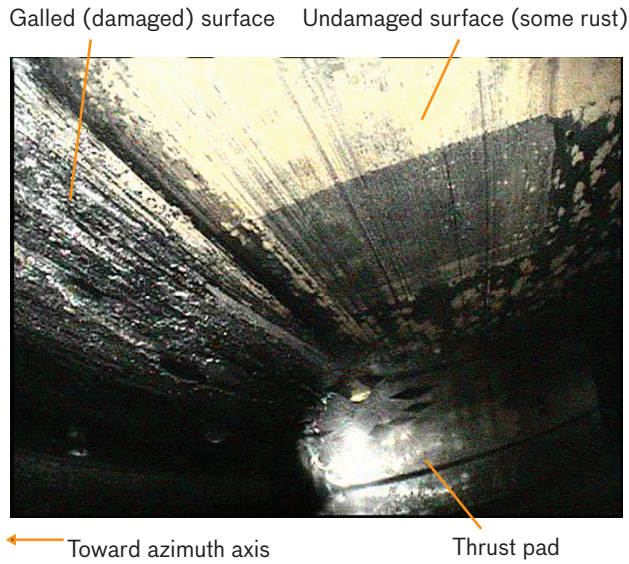
FIGURE 53. A boreoscope image of the thrust-runner surface shows the damaged portion on the left and the smooth portion on the right. The discoloration on the right is due to mild surface rust, likely from the integration period when the bearing was not being used. A thrust pad can be seen in the distance.
