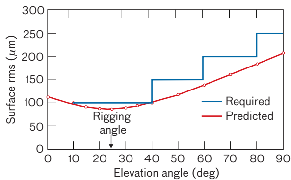
FIGURE A13. Predicted surface rms error when bias-rigged at 25° elevation.
