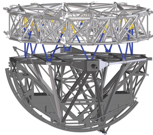
FIGURE 29. The reflector support struts (blue and yellow for the steel and aluminum sections, respectively) join the transition structure to the backstructure while providing isolation from differential thermal expansion.
