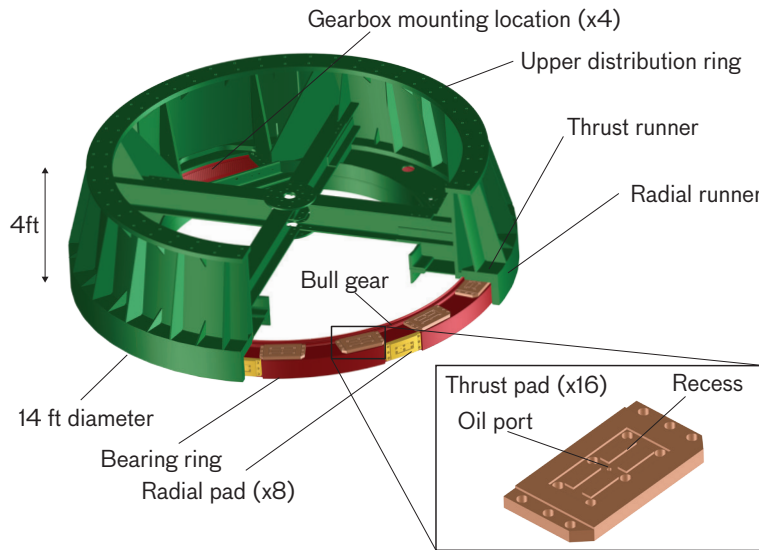
FIGURE 52. A CAD model of the key hydrostatic bearing components shows the thrust pads (bronze) and radial pads (yellow) mounted on the stationary bull gear (red). The pads exert force against the thrust and radial runners, respectively, which are parts of the rotating upper distribution ring (green).
