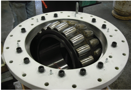
FIGURE 21. One of the elevation axis spherical roller bearings is assembled into its outer race.
