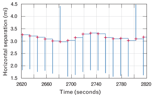
FIGURE 17. Sampled measurements of the separation of the aircraft by Hartford (QHA) radar. The blue lines represent the displayed separation as a function of time. The red plus signs are the sample separation compared to the GPS-provided true separation. The spikes occur as one aircraft position is updated prior to the other. The direction of the spikes depends on the order of the updates.
