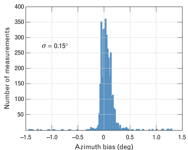
FIGURE 25. Distribution of azimuth bias errors for all sensors.
