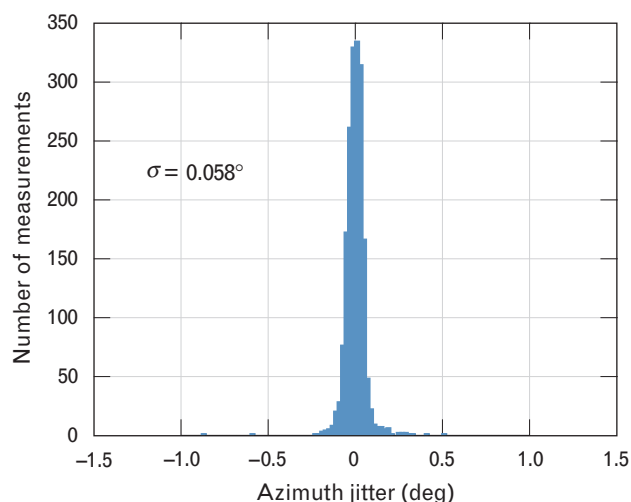
FIGURE 23. Distribution of azimuth jitter errors for the five MSSR sensors.
