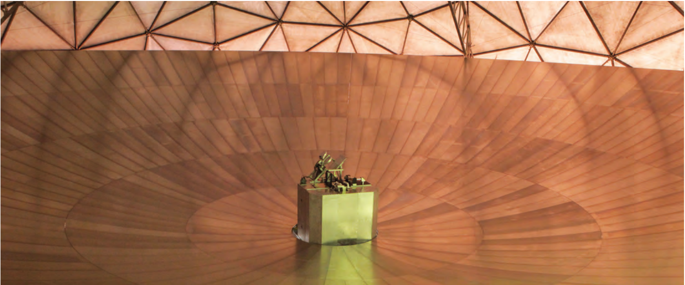
The Haystack Ultrawideband Satellite Imaging Radar (HUSIR) 37-meter-diameter primary reflector surface achieved its final precision alignment goal, allowing final dual-band (X and W) integration and testing to proceed in preparation for transitioning HUSIR to operational use in the U.S. Space Surveillance Network.
