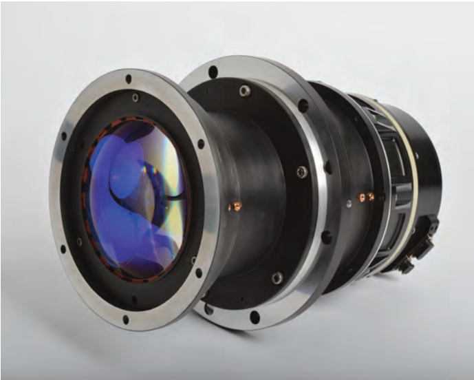
The Transiting Exoplanet Survey Satellite (TESS) system is composed of four optical sensors designed to map out the entire sky in the search for transiting exoplanets. Shown here is one of the prototype telescopes designed, built, and tested to support risk-mitigation efforts for the TESS project selected by NASA for a 2017 mission.
