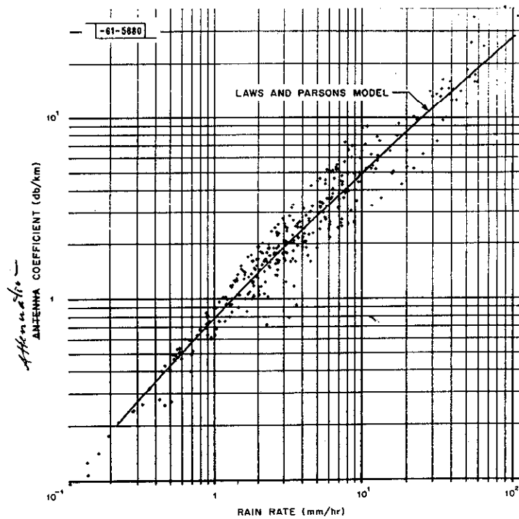
(g) Frequency: 70.0 GHz.
