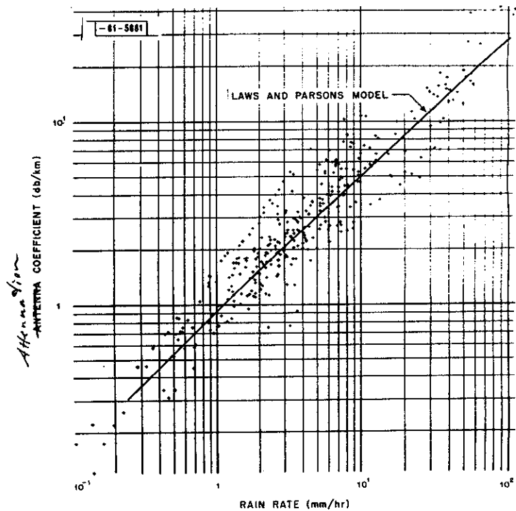
(h) Frequency: 94.0 GHz.
