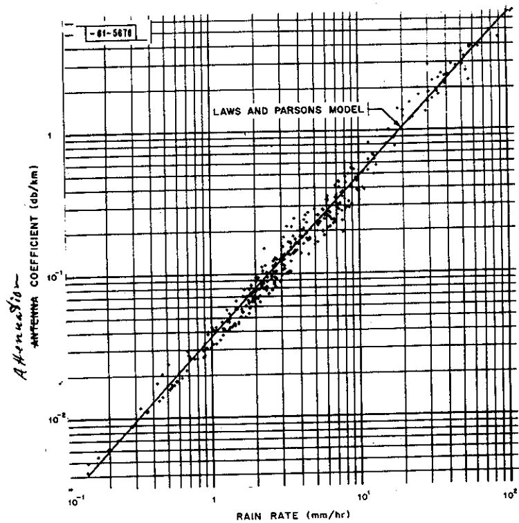
(e) Frequency: 15.5 GHz.
