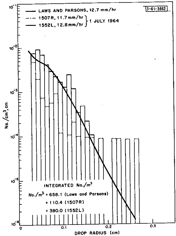
Fig. 2. Comparison of measured and modeled drop distributions, number density (No./cm 3 , cm).
