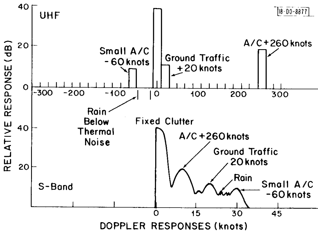
Fig. 3. Doppler domain responses of an S-band and a UHF radar to a typical environment.
