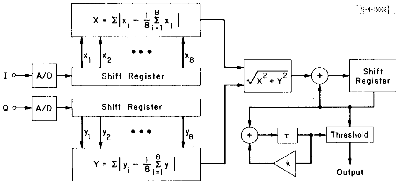
Fig. 11. Digital signal processor.
