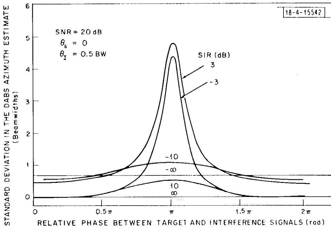
Fig. 4. Variance of the azimuth estimate in the presence of interference.
