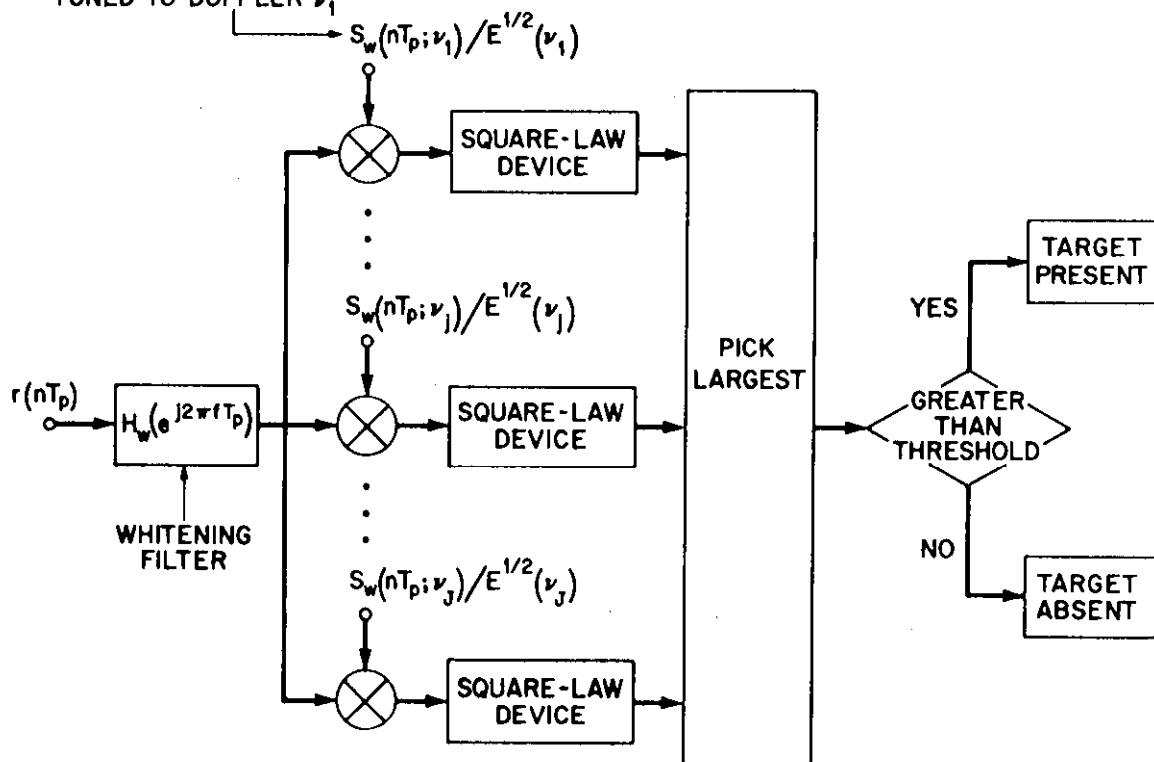
Fig. 3. Block diagram realization of optimum processor using whitening filters.
