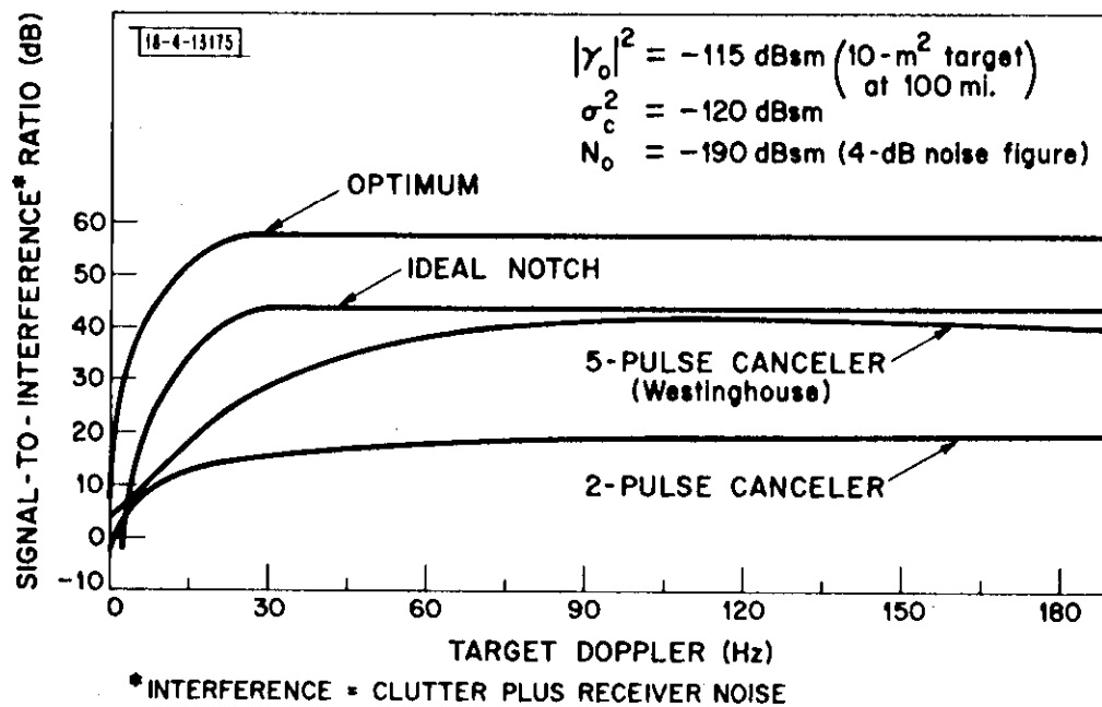
Fig. 7. Signal-to-interference ratios of well known MTI filters.
