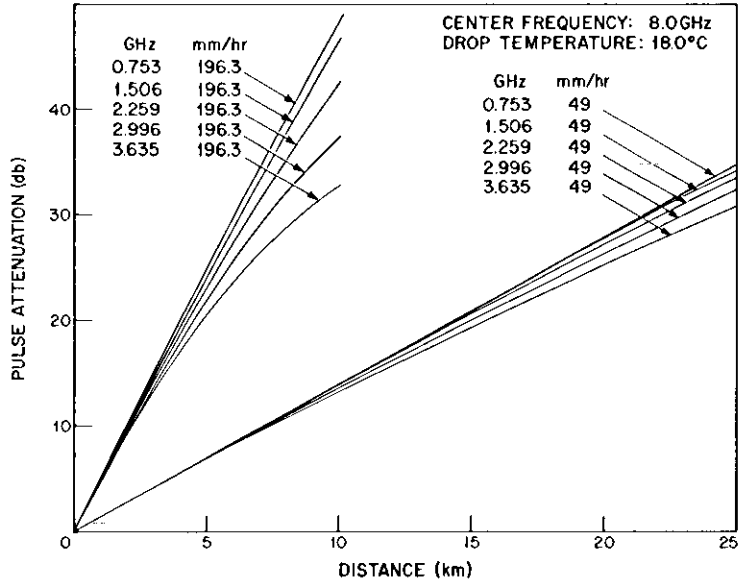
Fig. 9. Pulse attenuation vs. distance.
