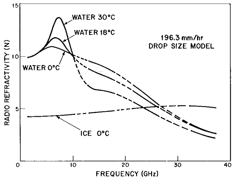
Fig. 11. Radio refractivity vs. frequency.
