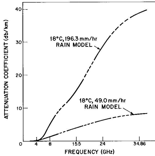
Fig. 3. Attenuation coefficient vs. frequency.
