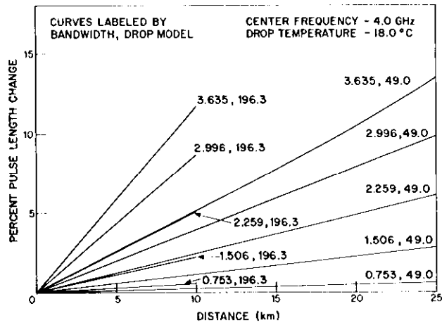
Fig. 5. Percent pulse length change vs. distance.
