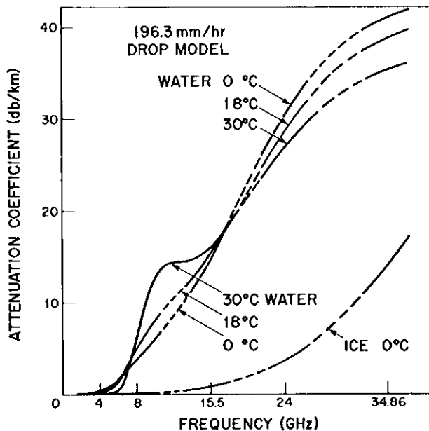
Fig. 12. Attenuation coefficient vs. frequency.
