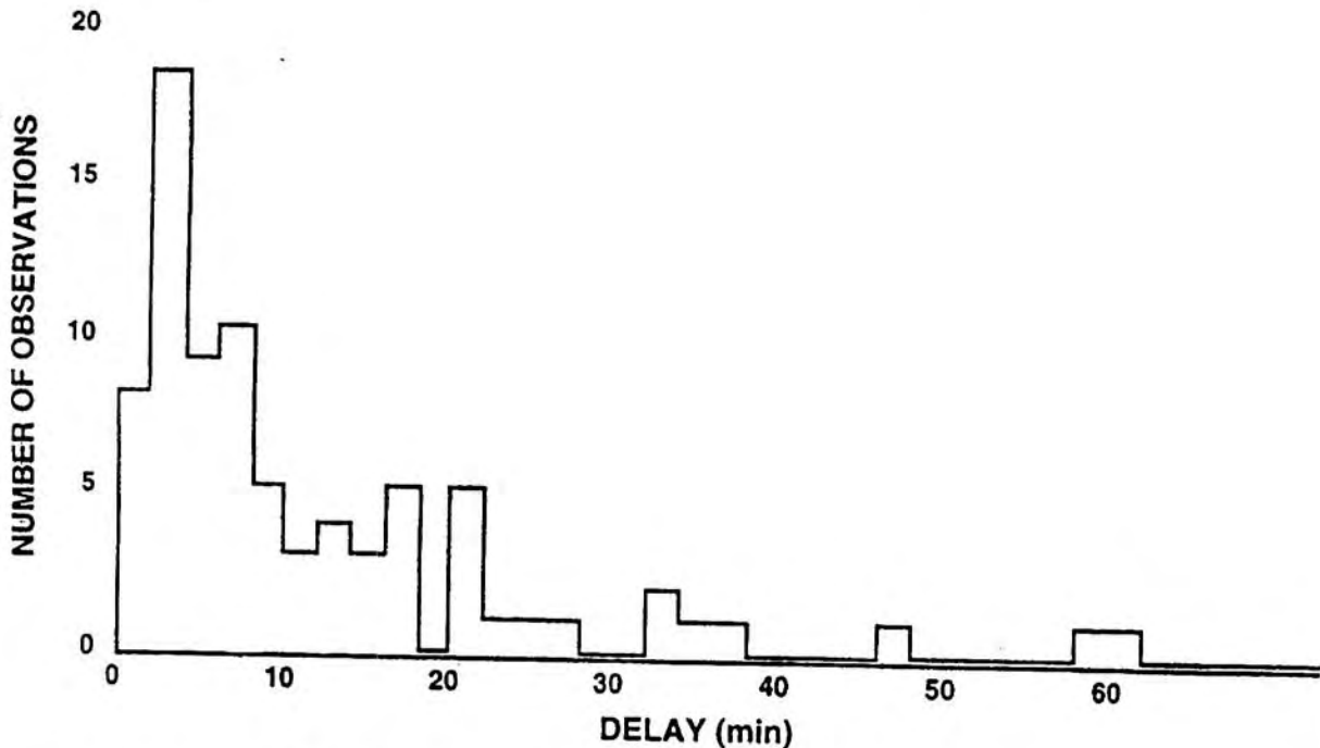
Figure 25. Distribution of delay between first intracloud and first cloud-to-ground flash in Florida thunderstorms.
