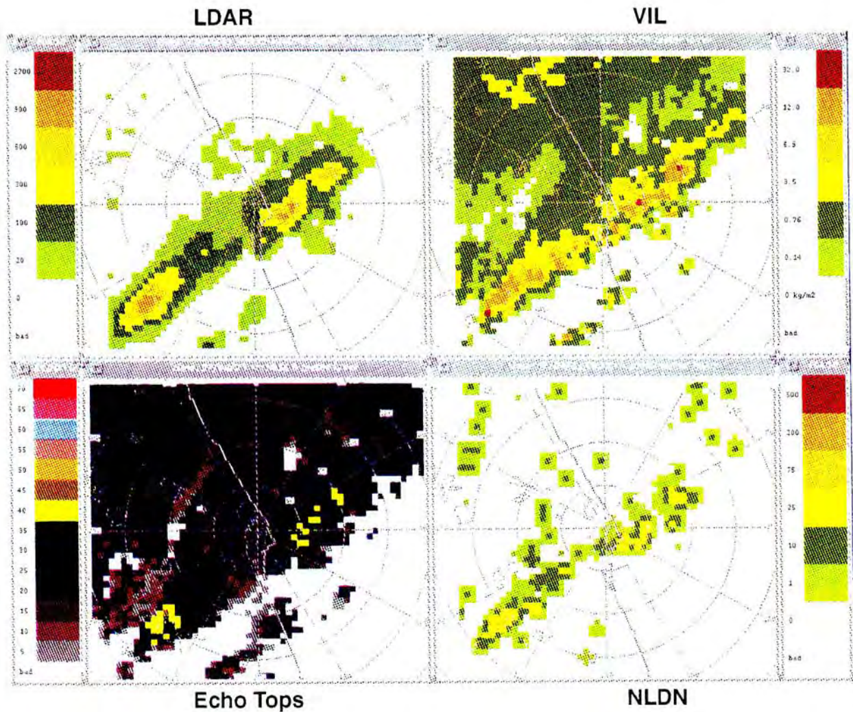
Figure 21. Four-panel plot showing LDAR, VIL and Echo Tops from NEXRAD, and NLDN data at 1638 UT on April 23, 1997. The lightning data has been mapped to two dimensions according to the procedure described in Appendix B. Lightning units are flashes per five-min. \times 48.8 (kernel weighting was not normalized). VIL units are \text{kg/m}^2 , and Echo Tops units are in kft.
