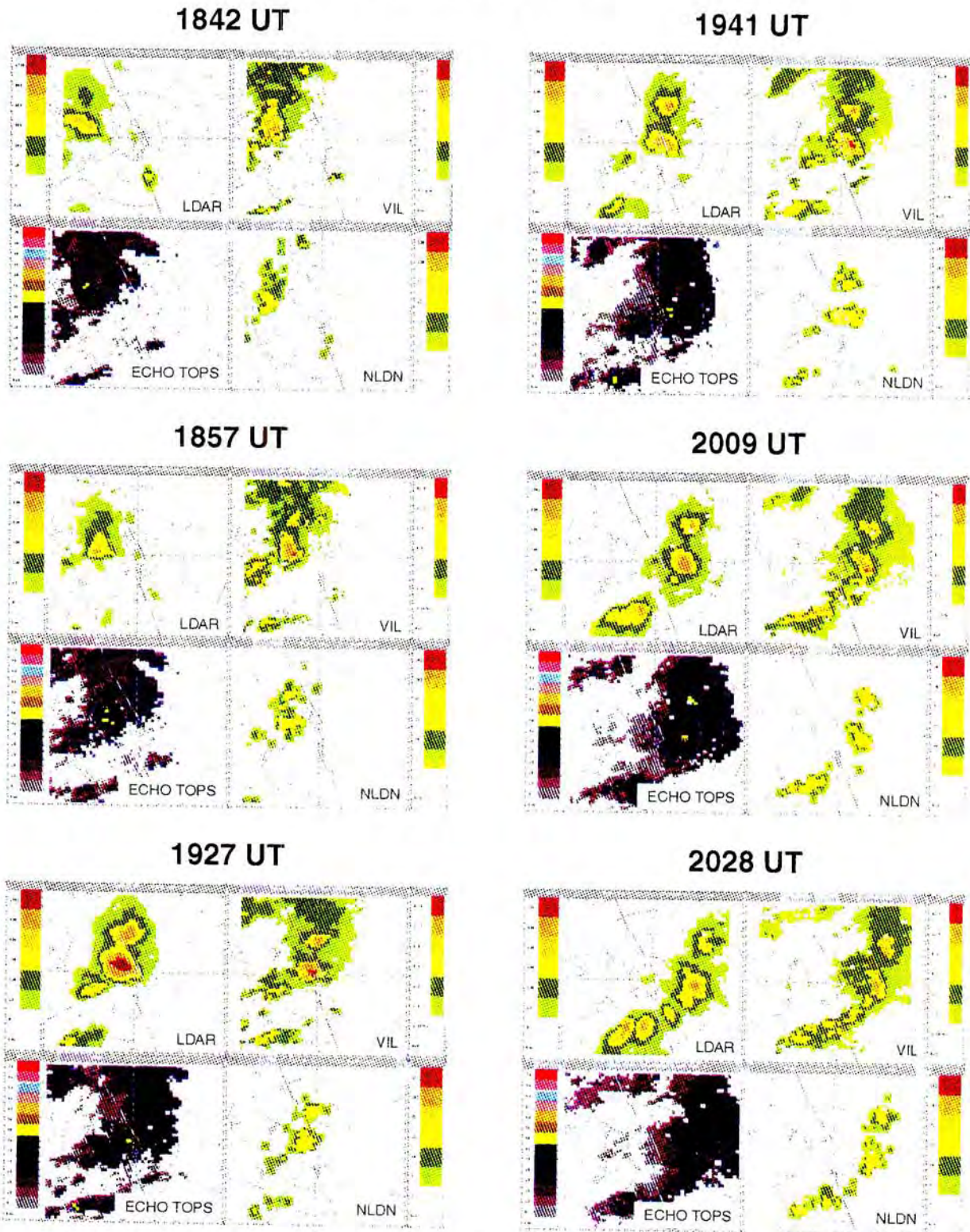
Figure 20. Six of the four-panel plots described in figure 19 are shown for March 29, 1997. Images for every scan in the time interval shown in Table 17 are available from the authors at Lincoln Laboratory.
