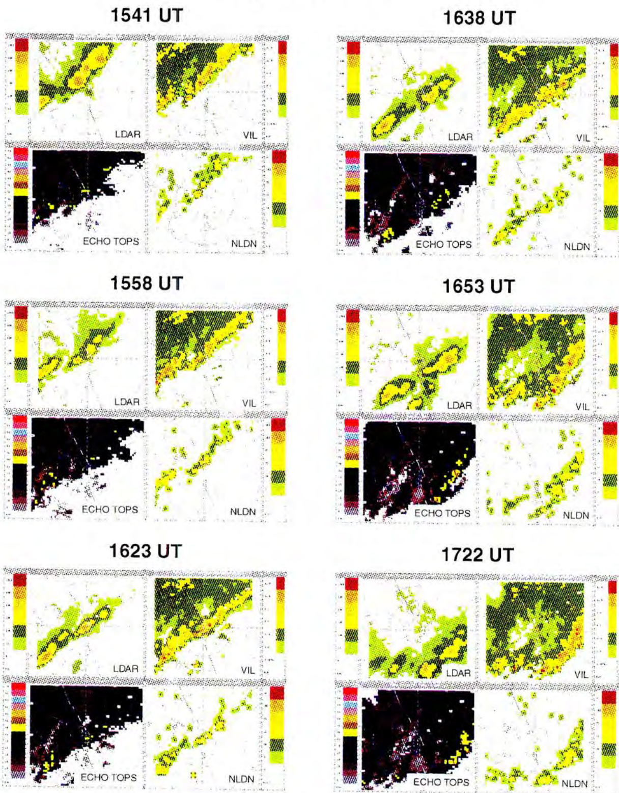
Figure 22. Six of the four-panel plots described in figure 21 are shown for April 23, 1997. Images for every scan in the time interval shown in Table 17 are available from the authors at Lincoln Laboratory.
