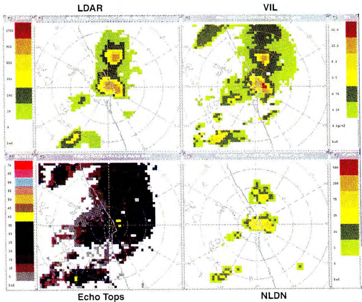
Figure 19. Four-panel plot showing LDAR, VIL and Echo Tops from NEXRAD, and NLDN data at 1941 UT on March 29, 1997. The lightning data has been mapped to two dimensions according to the procedure described in Appendix B. Lightning units are flashes per five-min. \times 48.8 (kernel weighting was not normalized). VIL units are \text{kg/m}^2 , and Echo Tops units are in kft.
