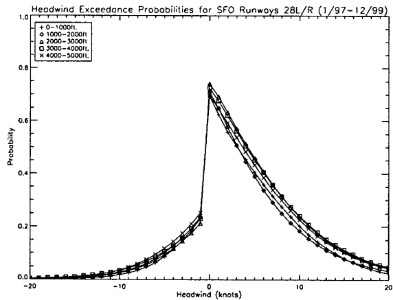
Figure 2. Headwind Exceedance Probabilities for SFO.
