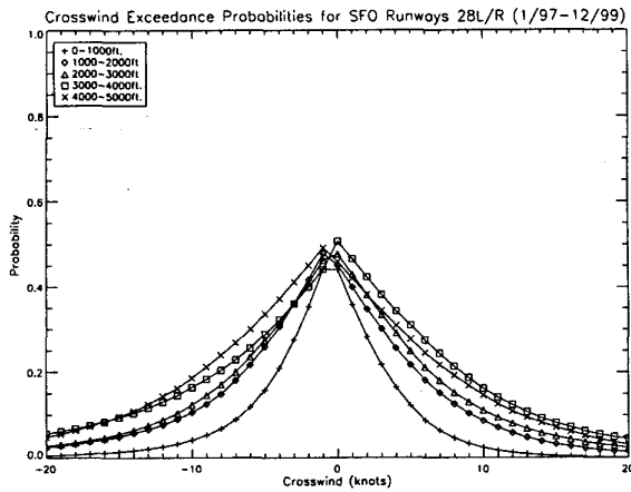
Figure 4. Crosswind Exceedance Probabilities for SFO.
