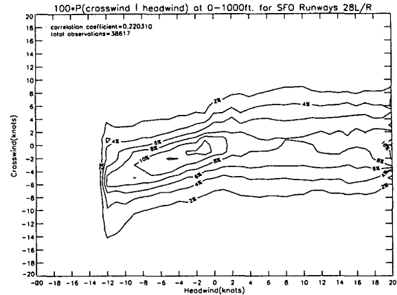
Figure 6. Conditional Crosswind Probabilities for SFO.
