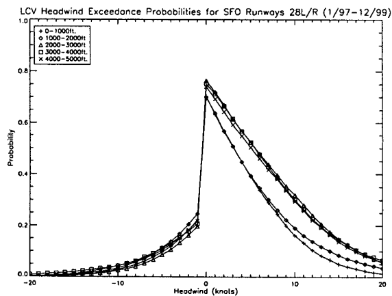
Figure 3. LCV Headwind Exceedance Probabilities for SFO.
