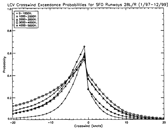
Figure 5. LCV Crosswind Exceedance Probabilities for SFO.
