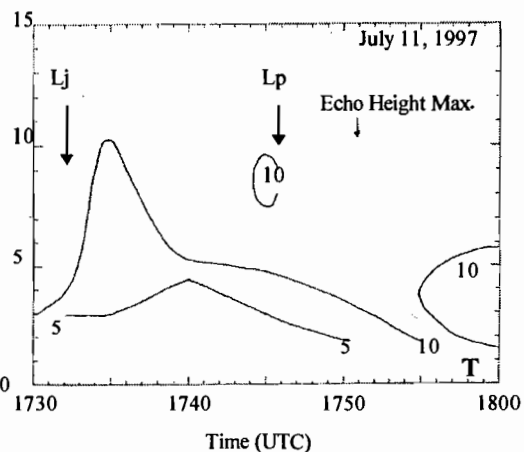
Fig.1. Lightning jump ( L_j ), peak ( L_p ), echo top (5 dBZ), and shear ( \times 10^{-3} ) time-histories of 3 tornadic storms. Tornado reported at time marked by the bold T .
