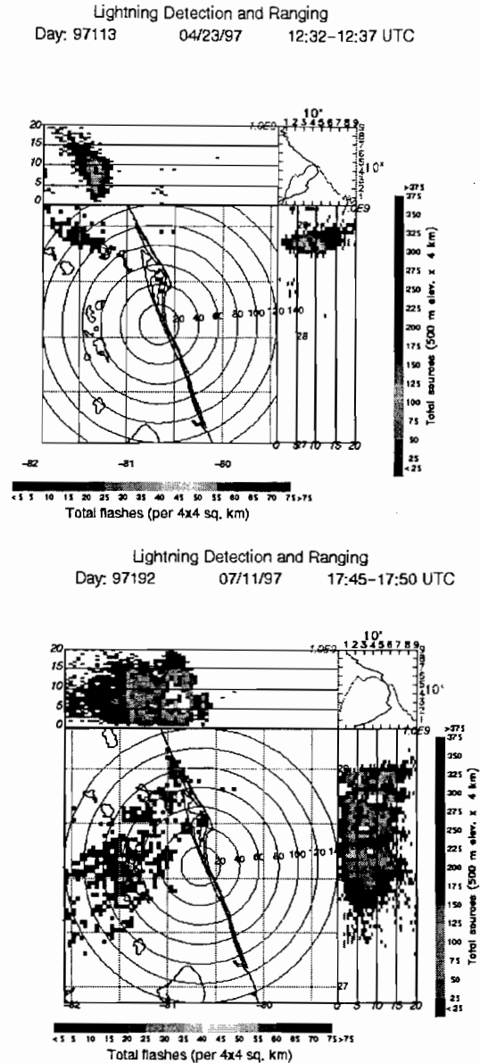
Fig. 2. LDAR flash density (x-y) and source distribution during the period of peak total flash rate on April 23 (top) and July 11 (bottom). The vertical density of sources are shown in a projection in the x-z and y-z planes. Range rings measured from the MLB NEXRAD (KMLB).
