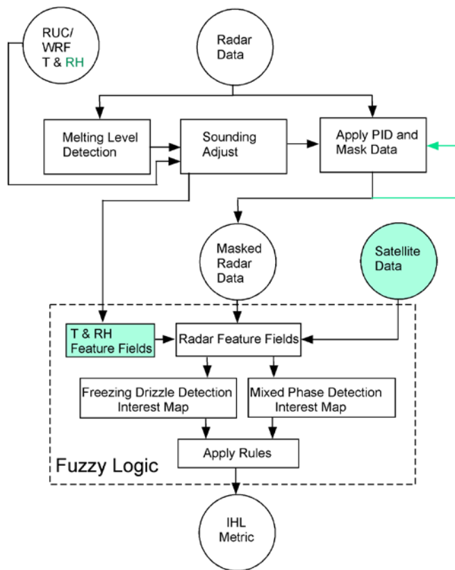
Figure 1: High-level diagram of the IHLA. Green-shaded features are not used in the current IHLA but the architecture allows for these in future versions.
