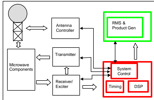
Figure 4. Legacy System Block Diagram
