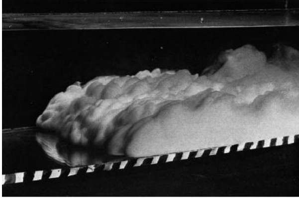
Figure 2. Density current in a transparent tank. The strip at the bottom is marked in intervals of 1 cm. (Simpson, 1969)
