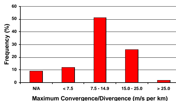
Figure 5. Percentage of analyzed gravity wave cases with maximum values of convergence and divergence. Data in this figure excludes that found along the leading edge of the initial gust front.
