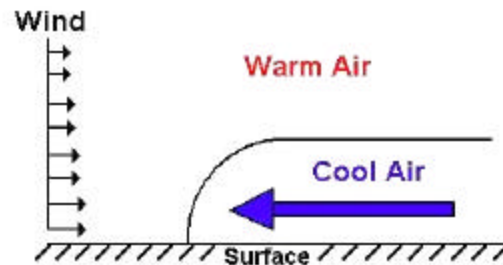
Figure 1. An idealized thunderstorm outflow encountering vertical shear in the environmental winds.
