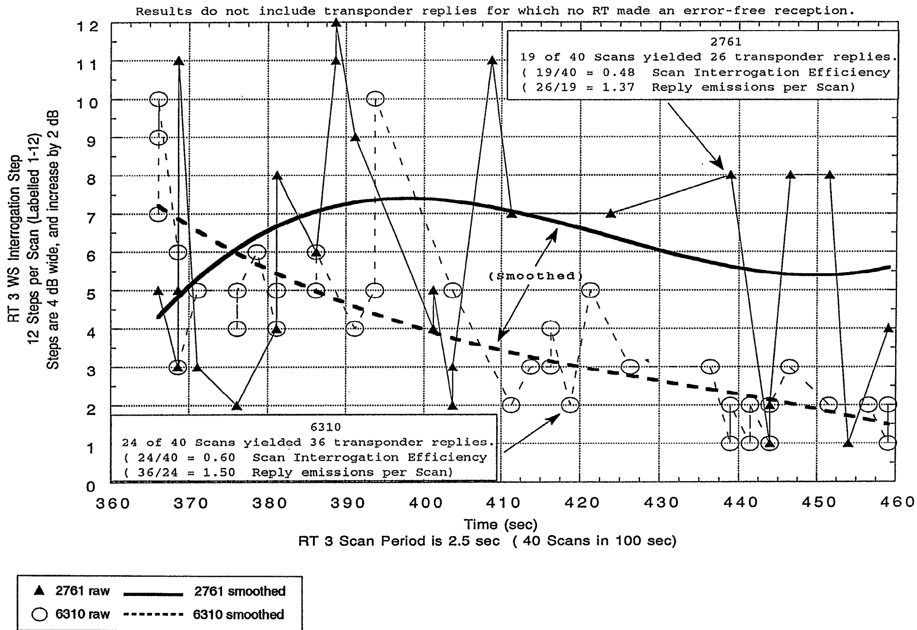
Figure 5-12. Partitioning by 4 dB Whisper Shout Sequence, Region RT.
