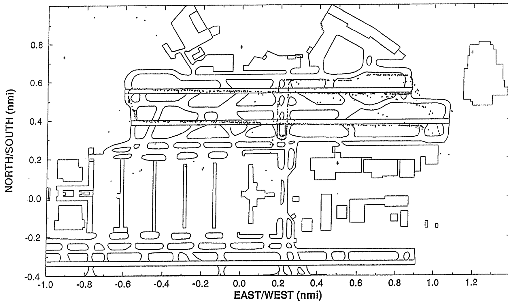
Figure C-2. Short squitter multilateration on SSV test target, by MIT Lincoln Laboratory playback (using unrefined survey). RT's are Delta, Ford, and Region.
