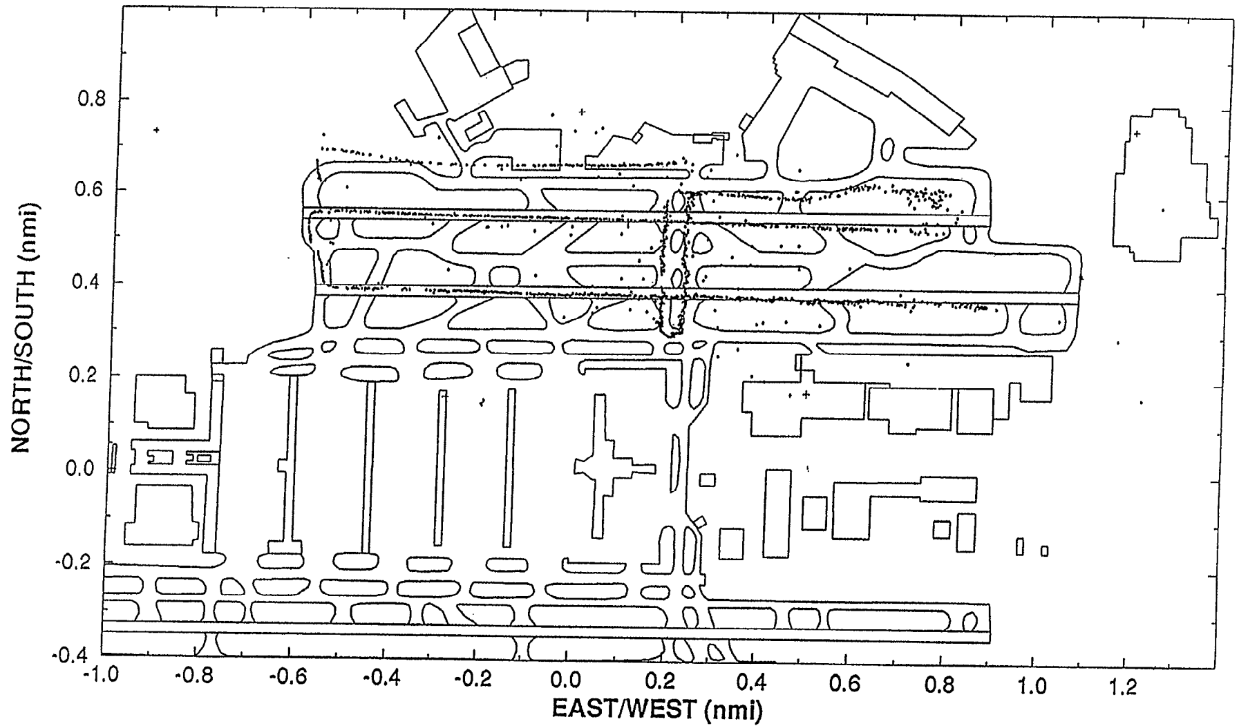
Figure C-10. Short squitter multilateration on SSV test target, by MIT Lincoln Laboratory playback (using unrefined survey). RT's are Stouffers, Region, and Terminal C.
