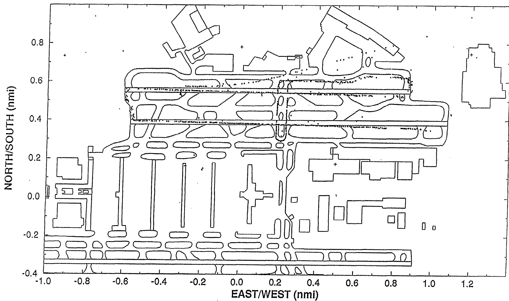
Figure C-5. Short squitter multilateration on SSV test target, by MIT Lincoln Laboratory playback (using unrefined survey). RT's are Delta, Stouffers, and Terminal C.
