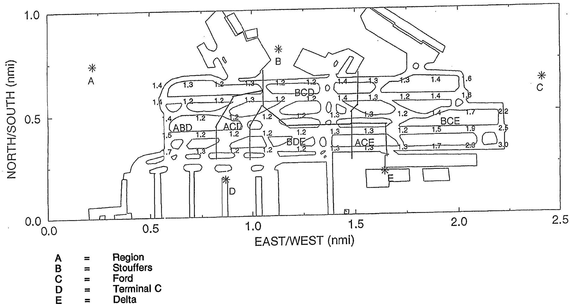
Figure B-1. Minimum GDOPs and associated RT triads.
