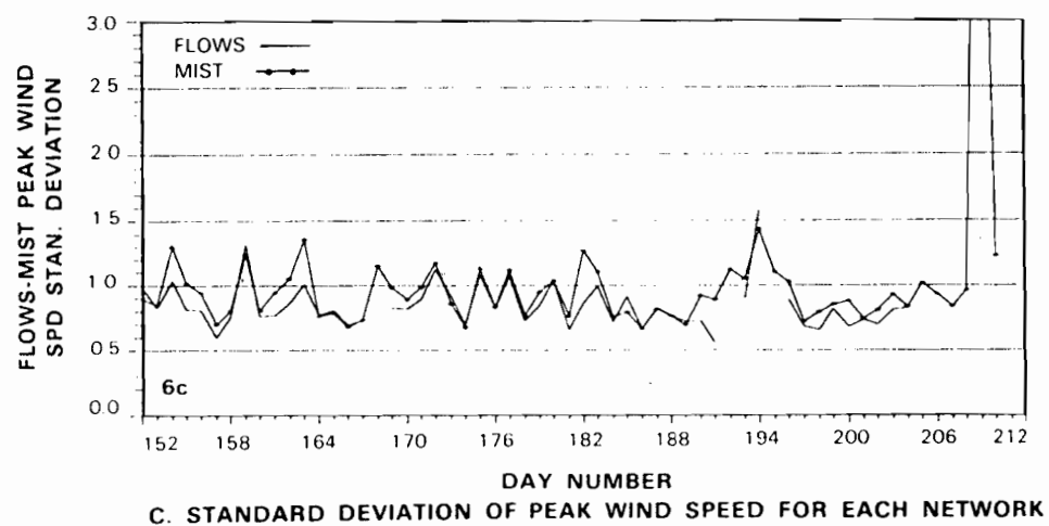
Figure 6. Peak wind speed comparison data for FLOWS and MIST networks.
