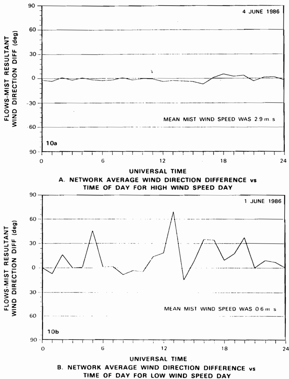
Figure 10. Difference between FLOWS and MIST network average wind direction vs. time of day (GMT) for a high wind speed day and a low wind speed day.
