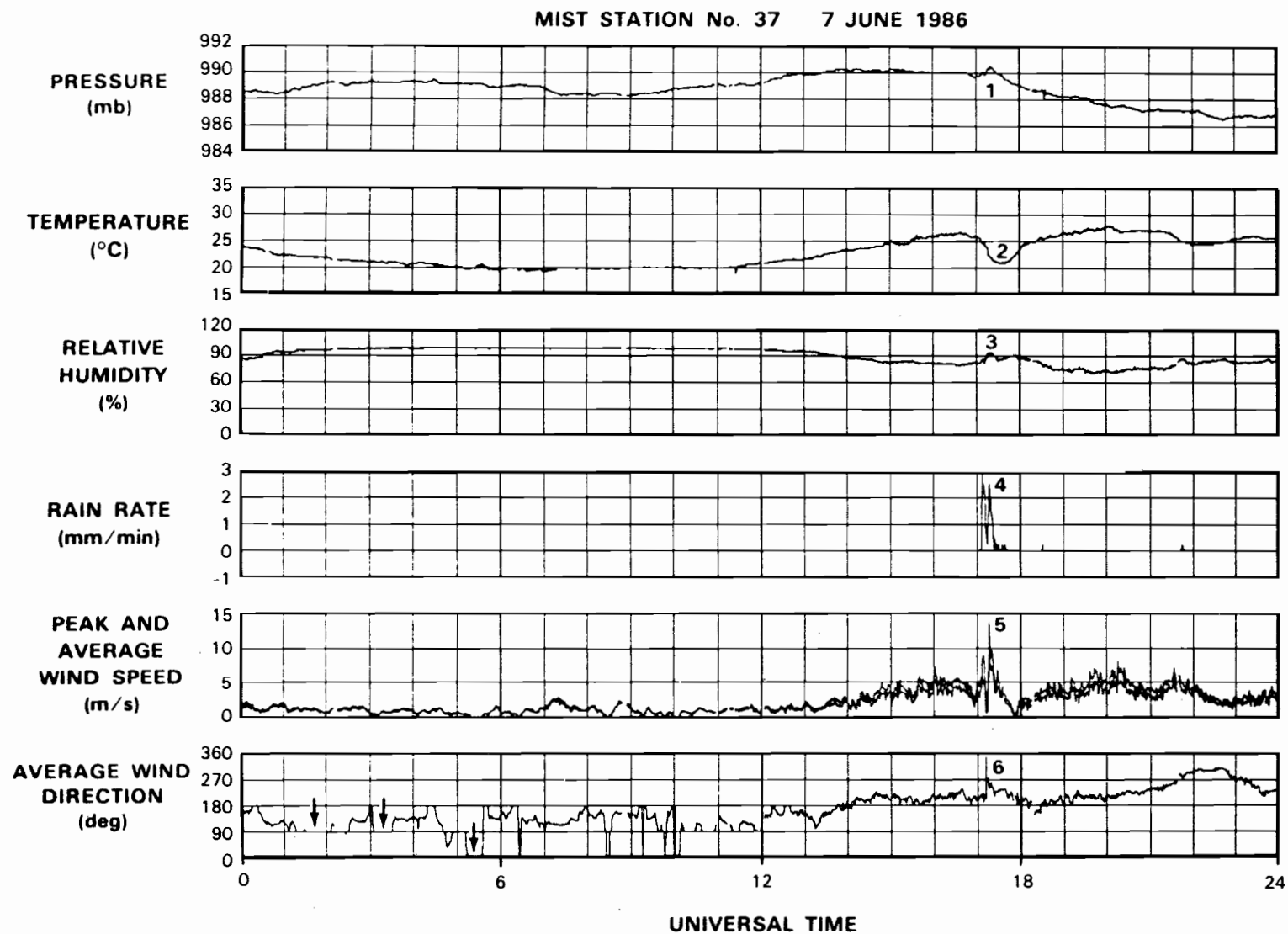
Figure 19. Comparison of 24-hour time series plots of data on 7 June 1986 (sheet 2 of 2).
