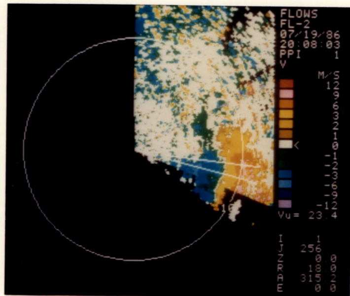
Figure III-7. Sector scan at 0.0^\circ elevation of reflectivity and radial velocity fields in a microburst near Huntsville, AL. The overlay indicates the range extent and azimuth interval between which the ASR velocity reports in Figure III-9 were simulated.
