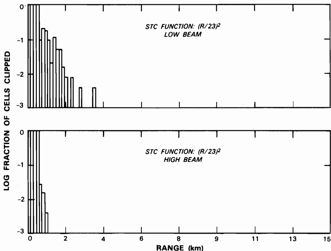
Figure IV-6a. Probability of receiver clipping (ensembled over azimuth) versus range for the ASR-8 at Memphis. As discussed in the text, an (R/23\text{km})^2 STC function is assumed.
