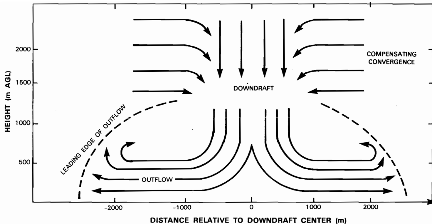
Figure I-1. Vertical cross section of microburst wind structure.
