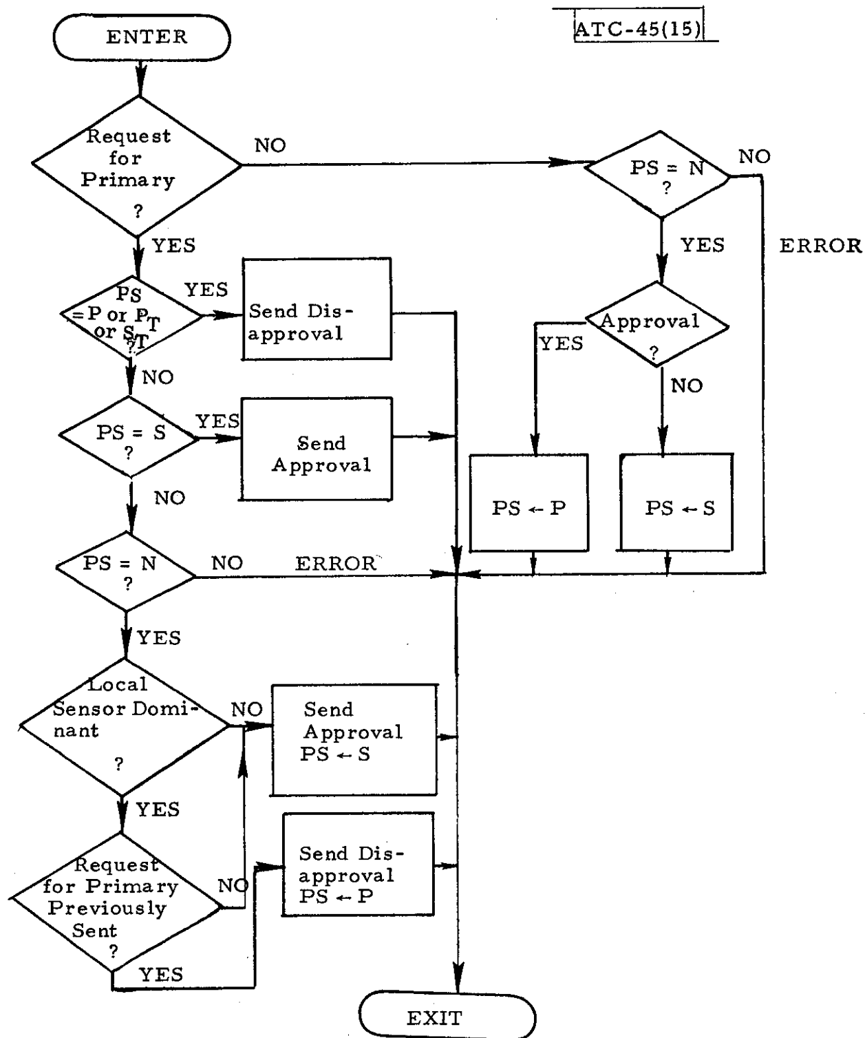
Fig. 15. Processing the transition zone coordination message.
