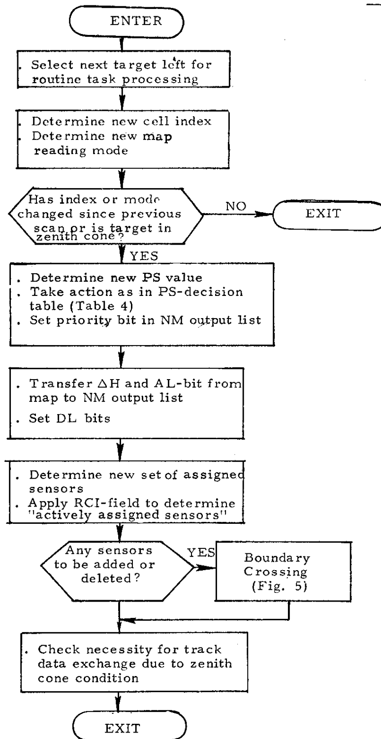
Fig. 3. Checks for boundary crossings and related tasks.
