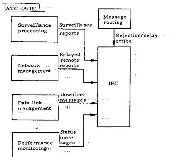
Fig. 18. Message flow - local sensor functions to IPC.
