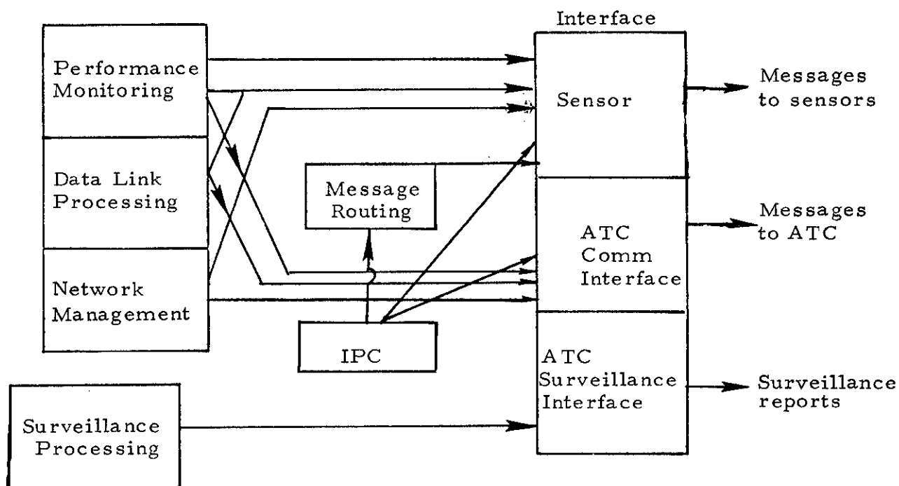
Fig. 16a. Message flow to local sensor functions.
