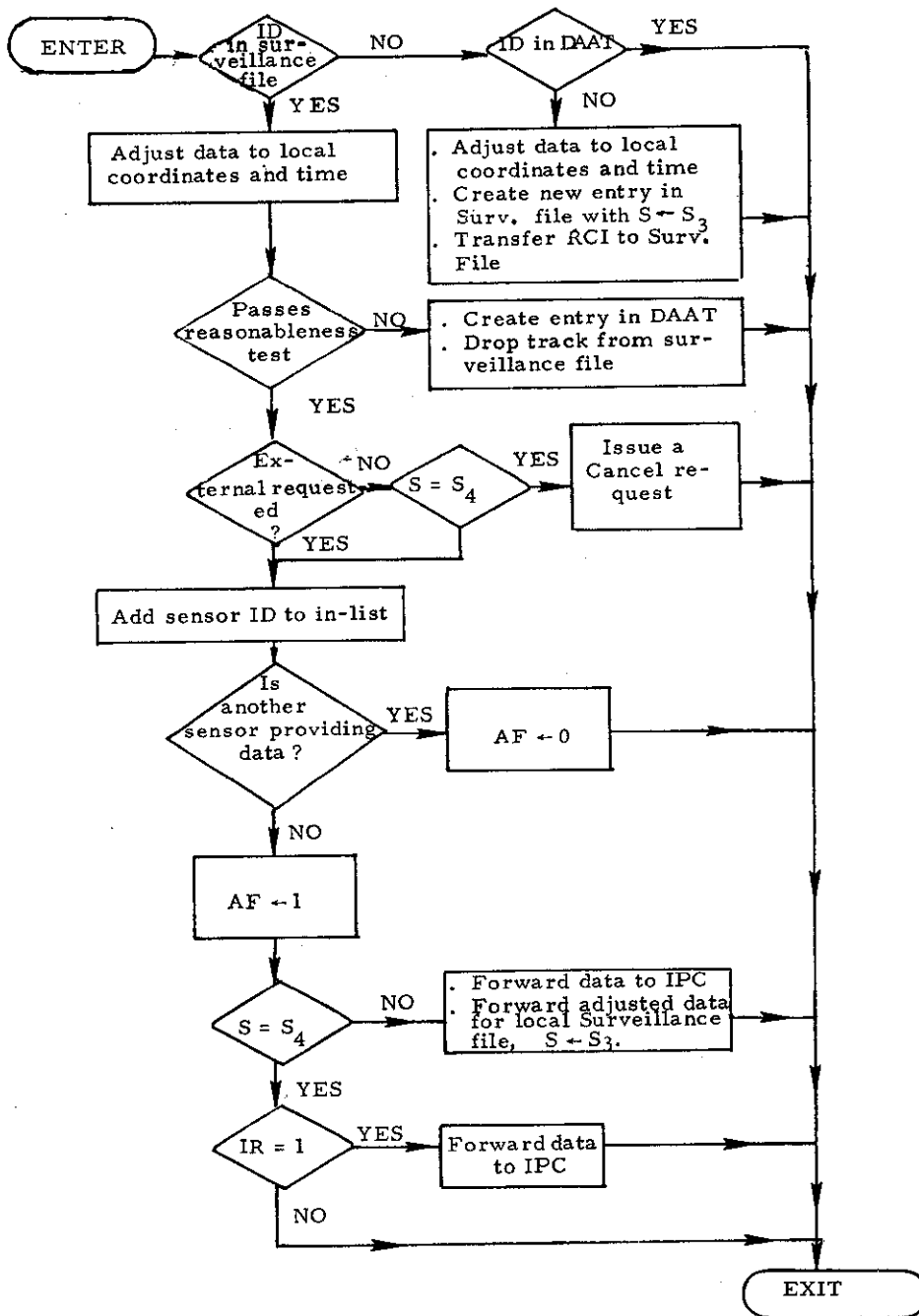
Fig. 12. Processing a data start message.
