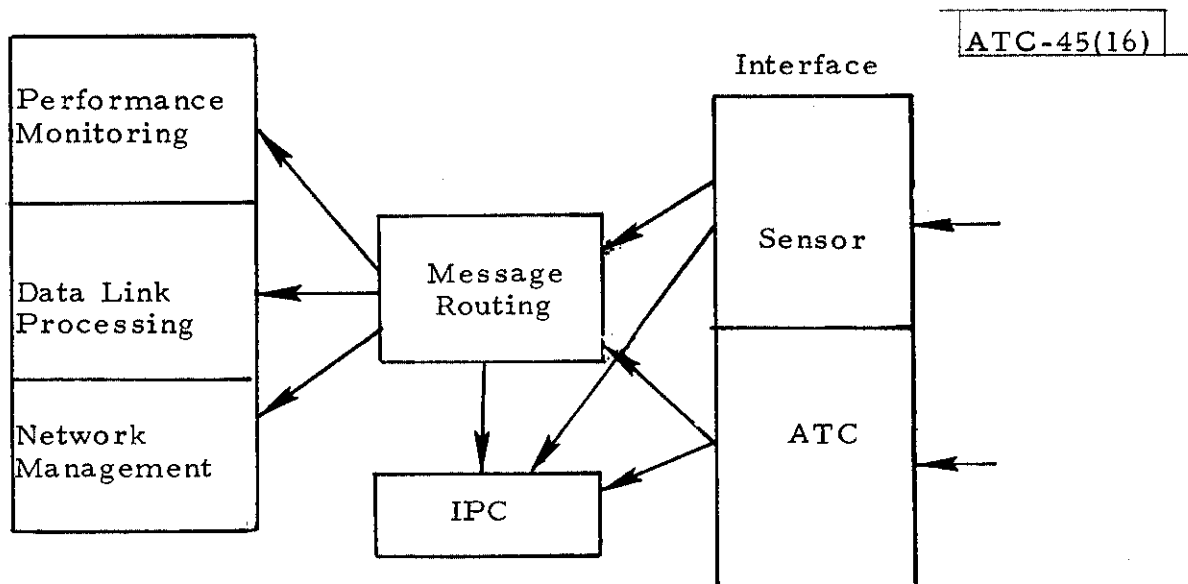
Fig. 16a. Message flow to local sensor functions.
