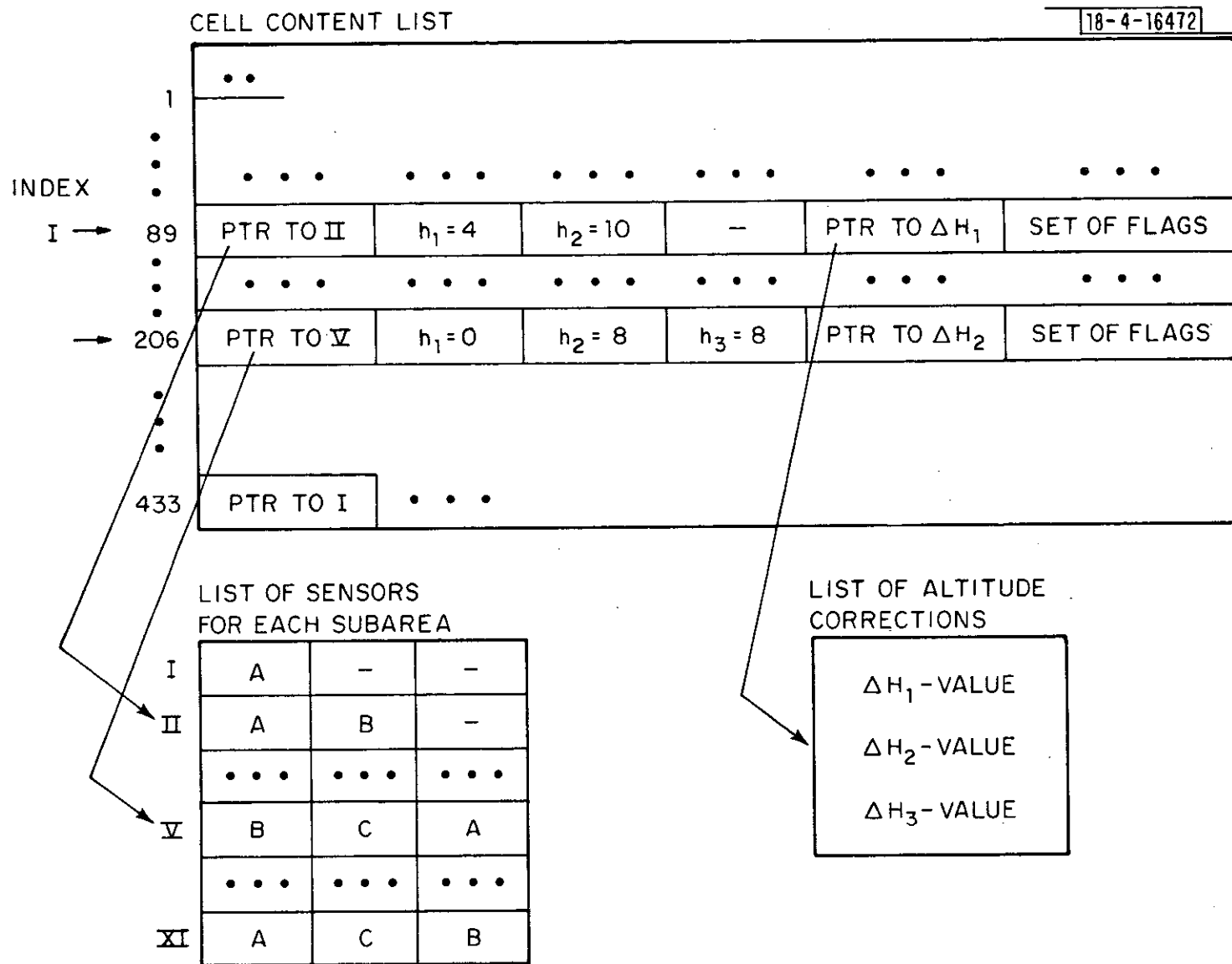
Fig. A.9 File structure for coverage map.
