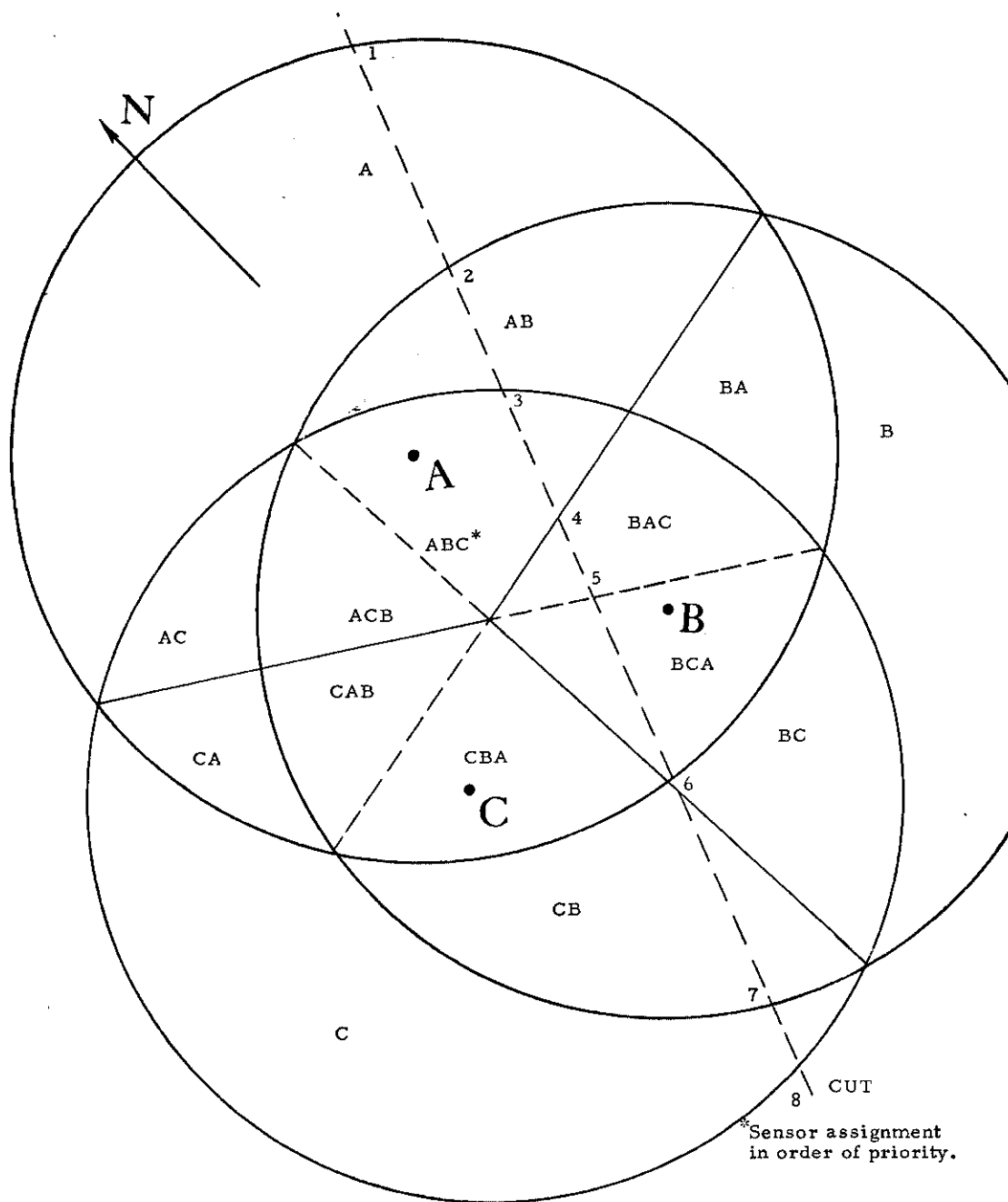
Fig. A. 1. Theoretical sensor assignment in the horizontal plane.
