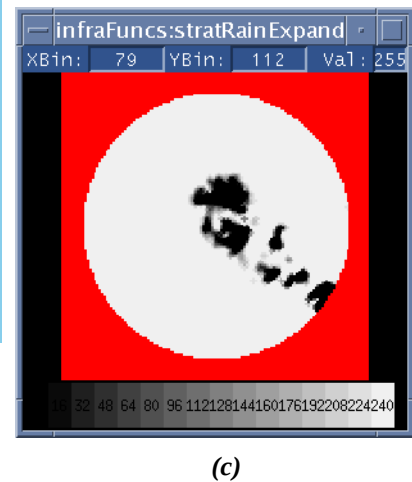
Figure 12. Example computation of "expanded" stratiform rain interest image. The scoring function (a) is applied to the reflectivity image (b) using a 3x3 ellipsoidal kernel. The resulting interest image is shown in (c). Lower X-axis of scoring function is the integer-scaled pixel value. Upper X-axis is reflectivity in dBZ. Data are from 5/24/99 at Albuquerque, NM.
