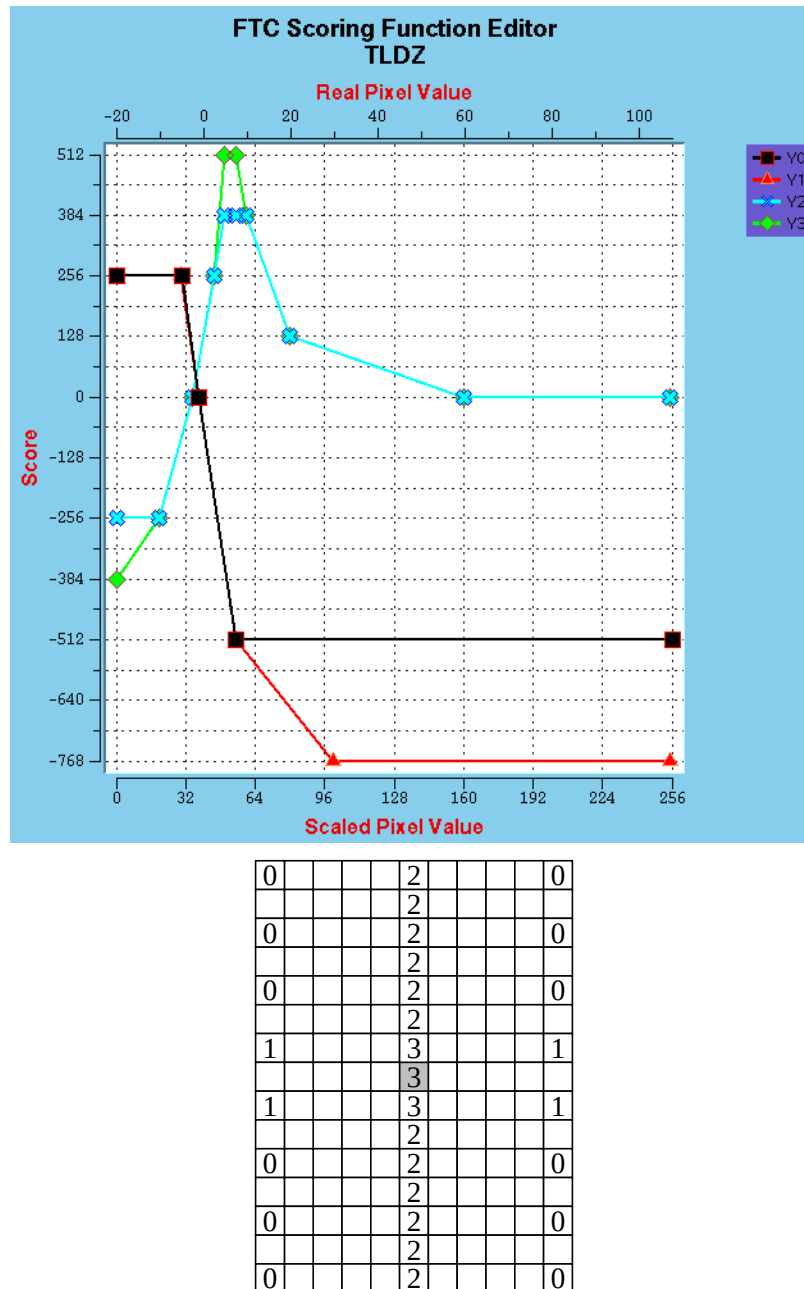
Figure 24. Scoring functions and template for the TLDZ reflectivity thin line detector. Lower X-axis of scoring function is the integer-scaled pixel value. Upper X-axis is reflectivity in dBZ.
