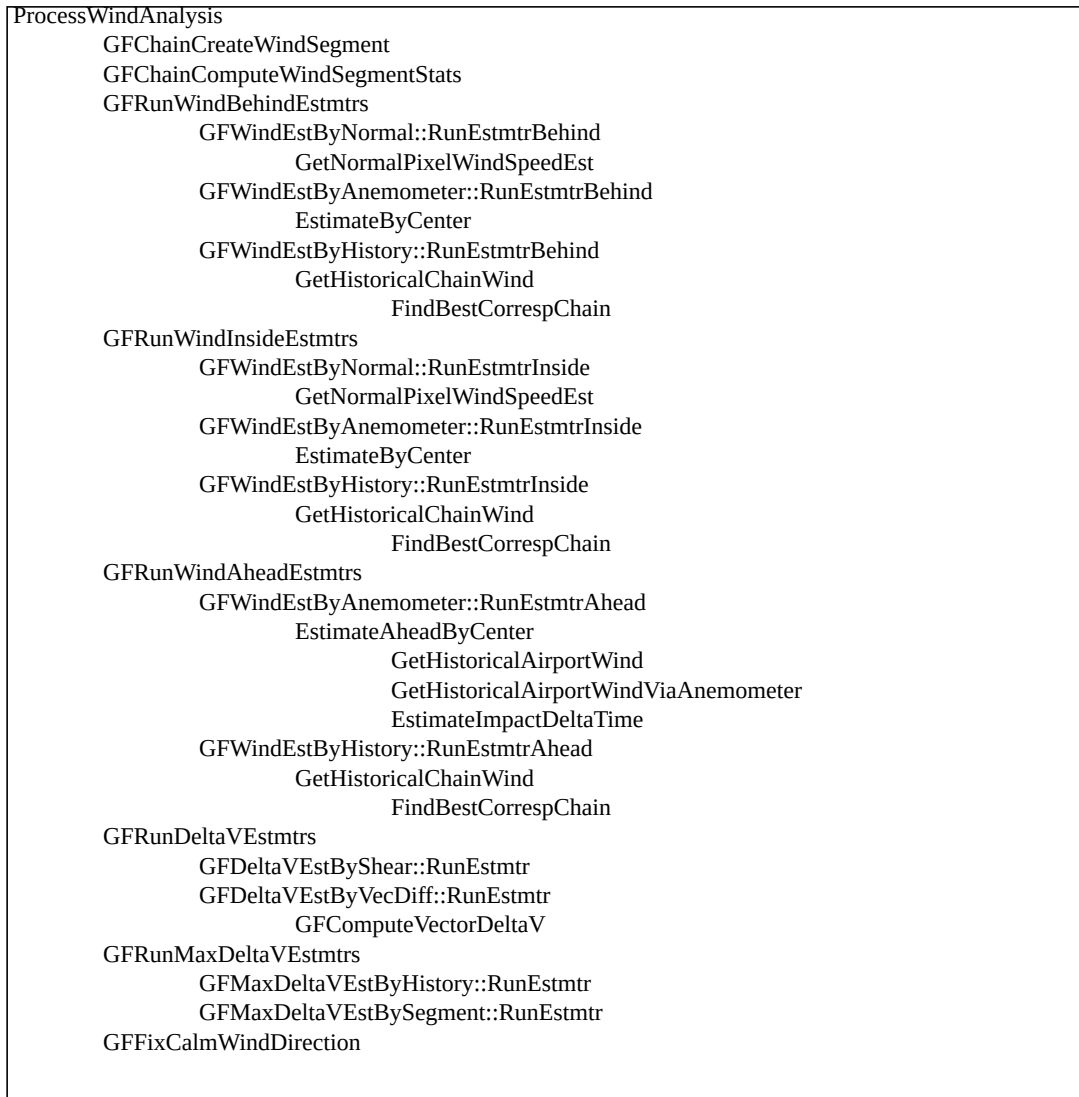
Figure 48. Function call tree for the MIGFA wind analysis stage (see text for description).
