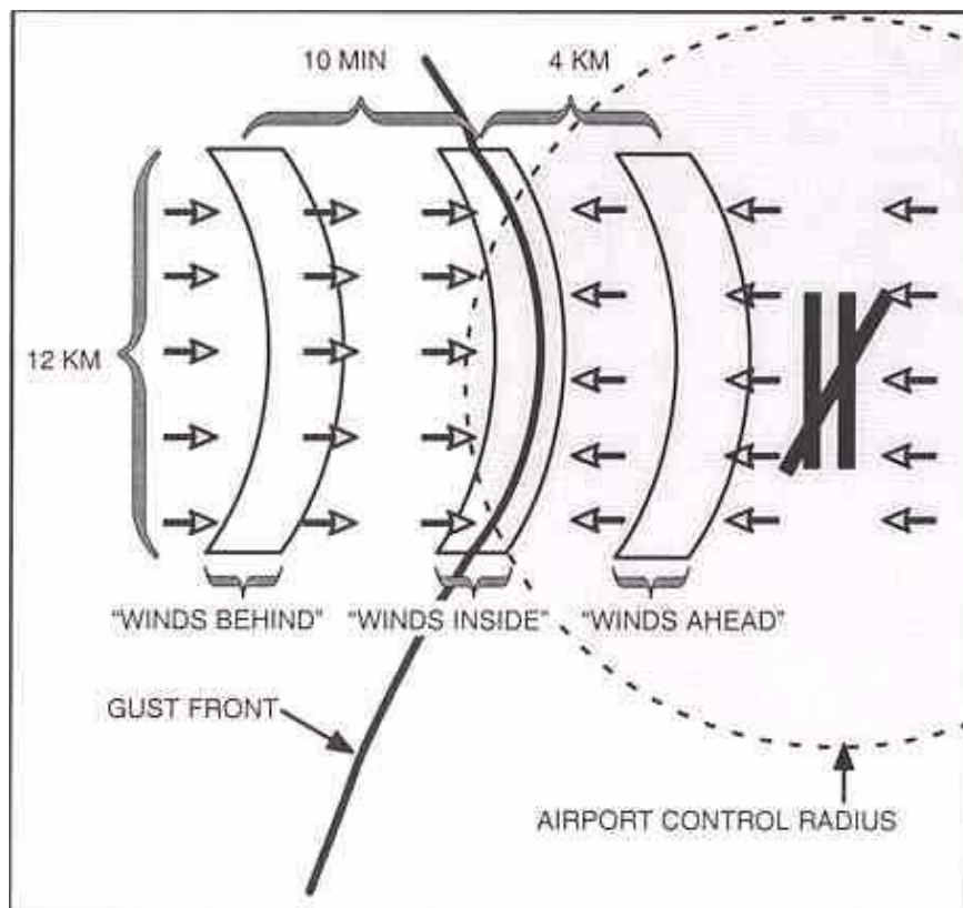
Figure 49. Wind analysis regions for MIGFA gust front wind shift and wind shear estimation. For WSP, the "winds behind" region is defined to be 0 minutes behind the front, so the "winds behind" region for WSP MIGFA is the same as the "winds inside" region.
