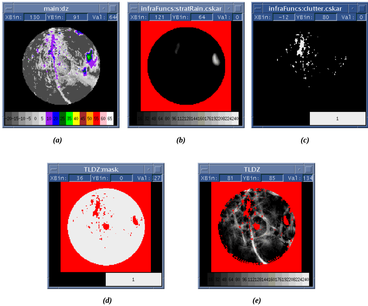
Figure 25. Summary of processing stages of TLDZ reflectivity thin line detector. A gust front thin line echo can be seen as a N-S oriented line of 0-10 dBZ echoes just west of the radar in the input dual-beam reflectivity (a). The corresponding stratiform rain interest image is shown in (b). This stratiform rain image is used together with the corresponding binary clutter mask image (c) and 2-km site mask (not shown) to form the detection mask shown in (d). The resulting TLDZ interest image is shown in (e). Data are from 7/13/99 at Austin, TX
