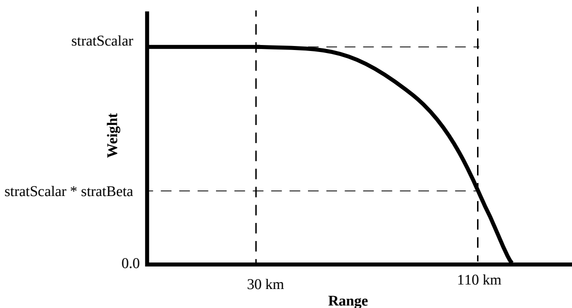
Figure 20. Illustration of stratiform rain and storm cell pixel weighting for precipitation coverage computation.
