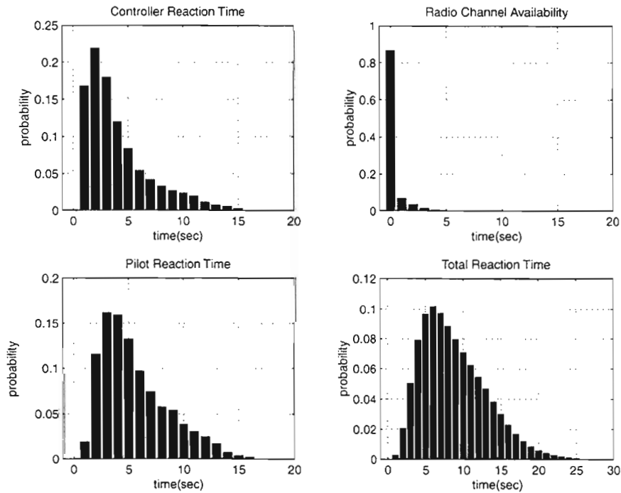
Figure 58. Probability density functions for reaction times for tower cab alerting systems.
