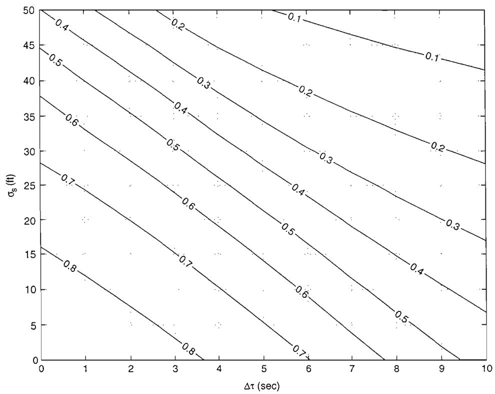
Figure 23. Save probability surface for taxi, 10 kts, direct cockpit alert with B-747 on runway.
