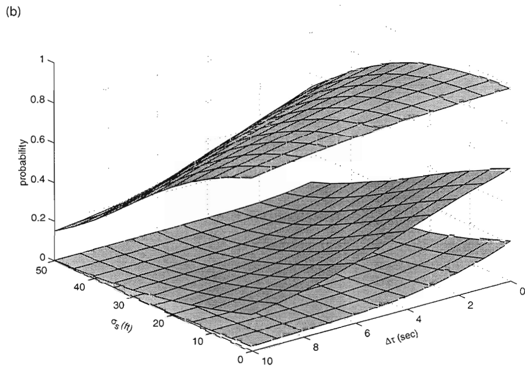
Figure 14. Two different axes views of save probability plots for a taxi speed of 5, 10, and 15 kts, B-747 on runway.
