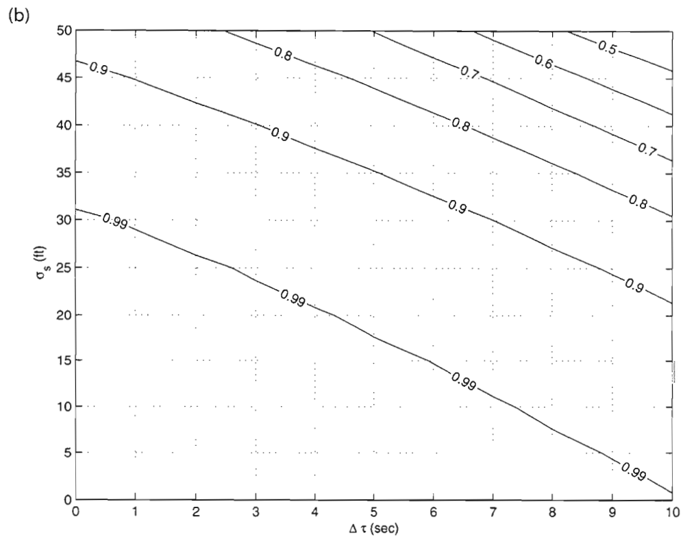
Figure 22. Save probability surface for taxi, 5 kts, direct clock alert with B-747 on runway.
