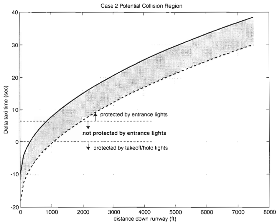
Figure 50. Effective surveillance parameters and protected portion of the Case 2 potential collision region.
