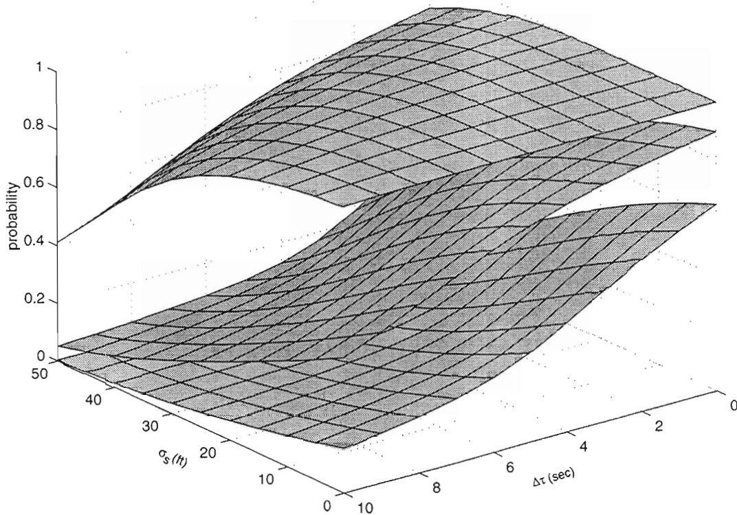
Figure 25. Save probability surface for taxi, 5, 10, and 15 kts, direct cockpit alert with B-747 on runway.
