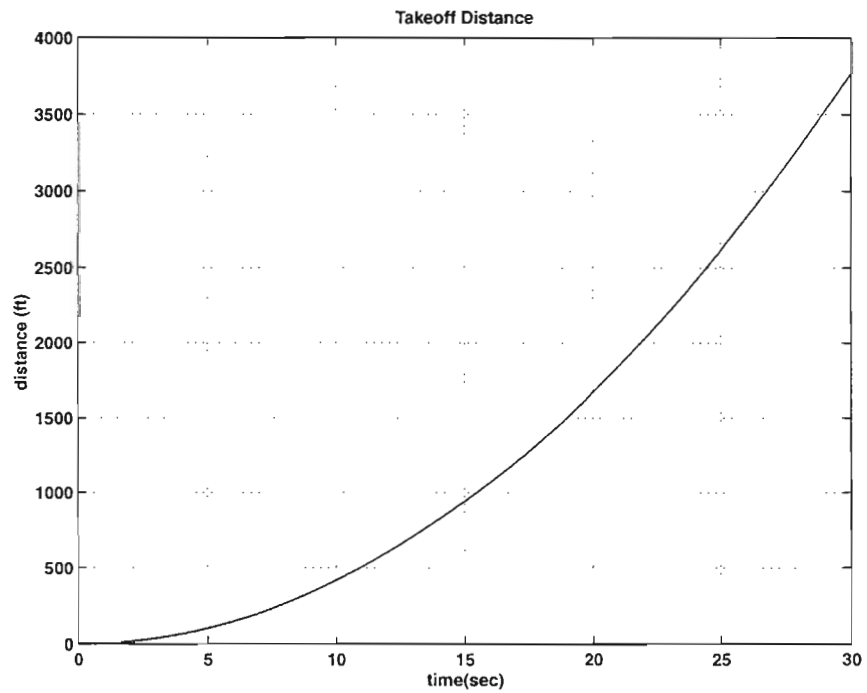
Figure 30. Nominal takeoff aircraft takeoff distance.
