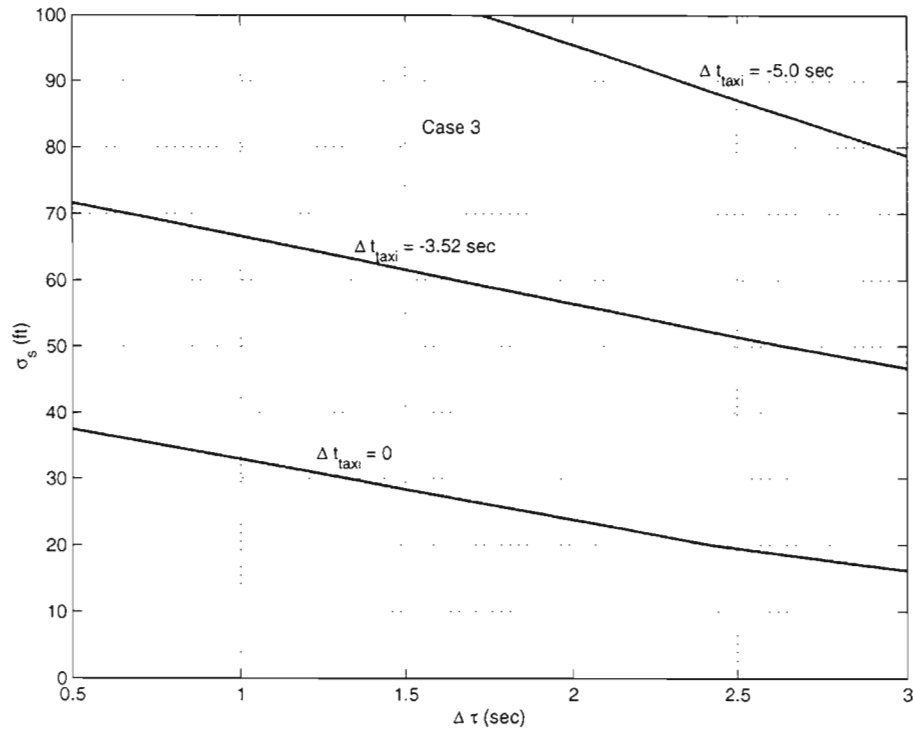
Figure 64. Surveillance requirements for rejected takeoff for Case 3.
