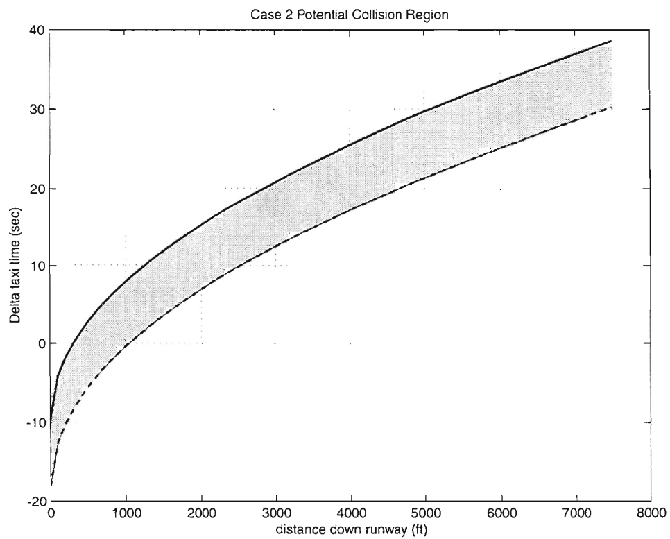
Figure 49. Potential collision region for Case 2 incursion.
