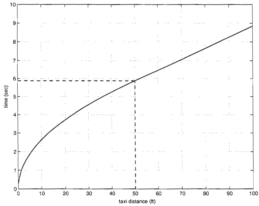
Figure 18. Taxi time profile for nominal taxi.
