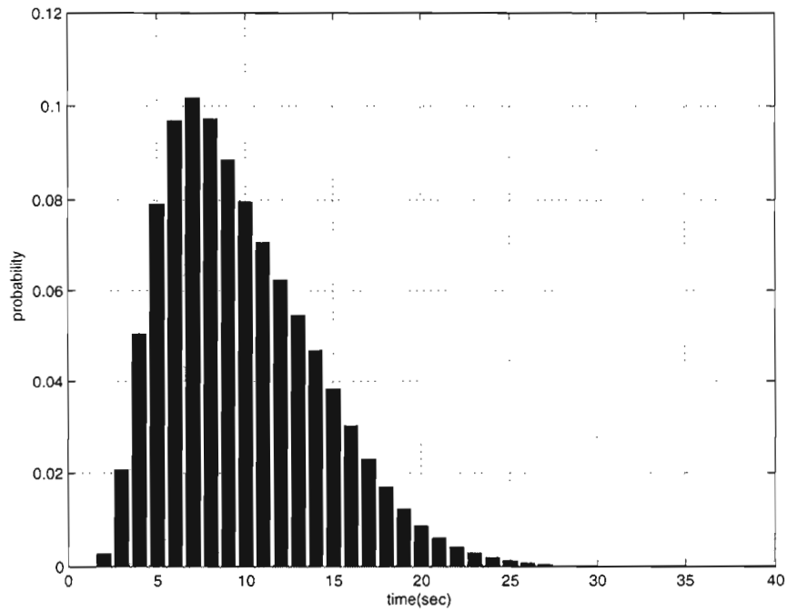
Figure 5. Total reaction time pdf.
