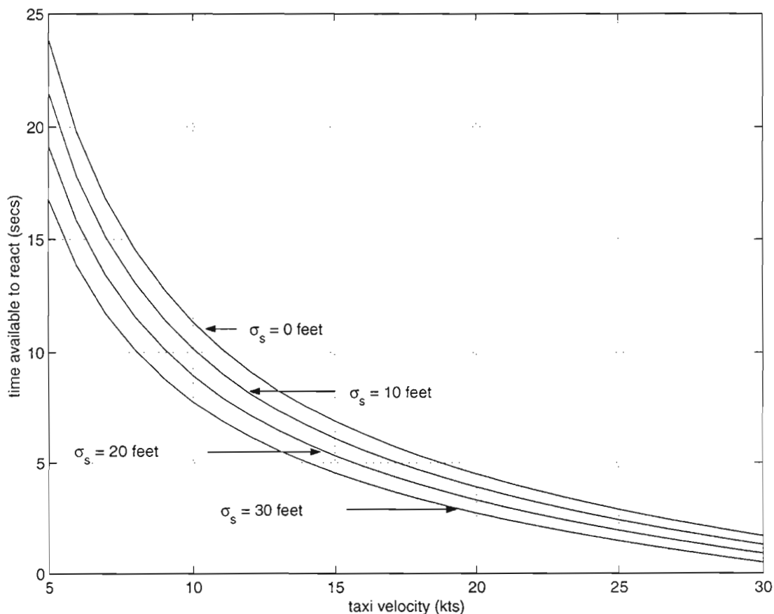
Figure A-1 Time available to react to a taxi aircraft incursion as a function of taxi velocity and surveillance position accuracy.
