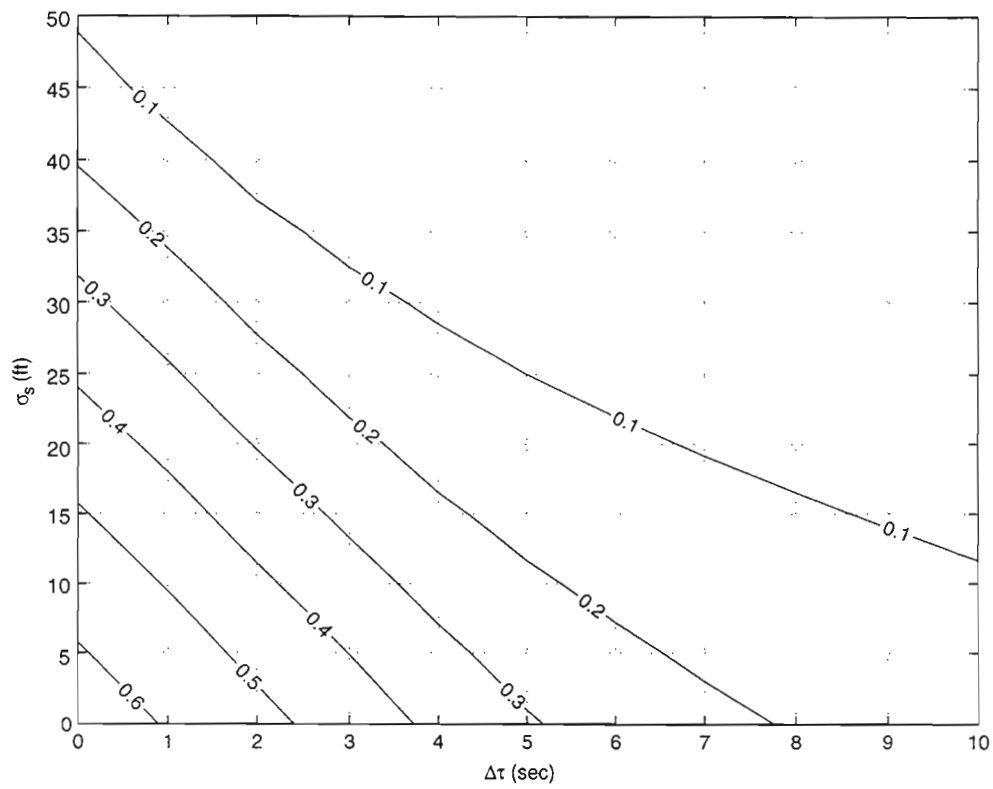
Figure 24. Save probability surface for taxi, 15 kts, direct cockpit alert with B-747 on runway.
