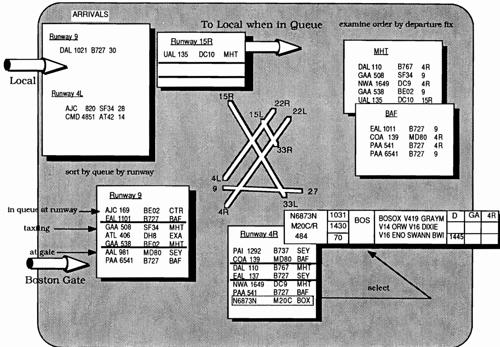
Figure 9d. ASMS Ground Control Screen
