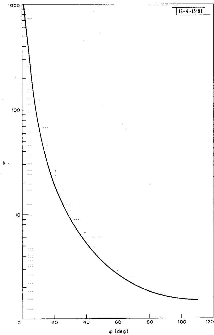
Fig. 1.1. A lower bound to the geometric dilution factor, k , with four satellites within a cone of half angle \phi .
