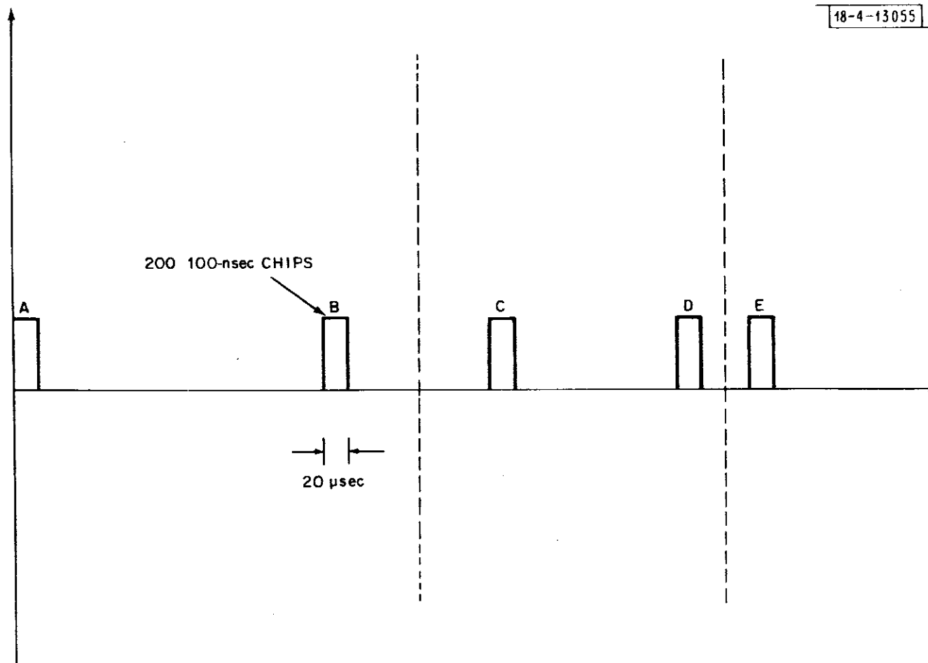
Fig. 2.1. A typical FSRR signature.
