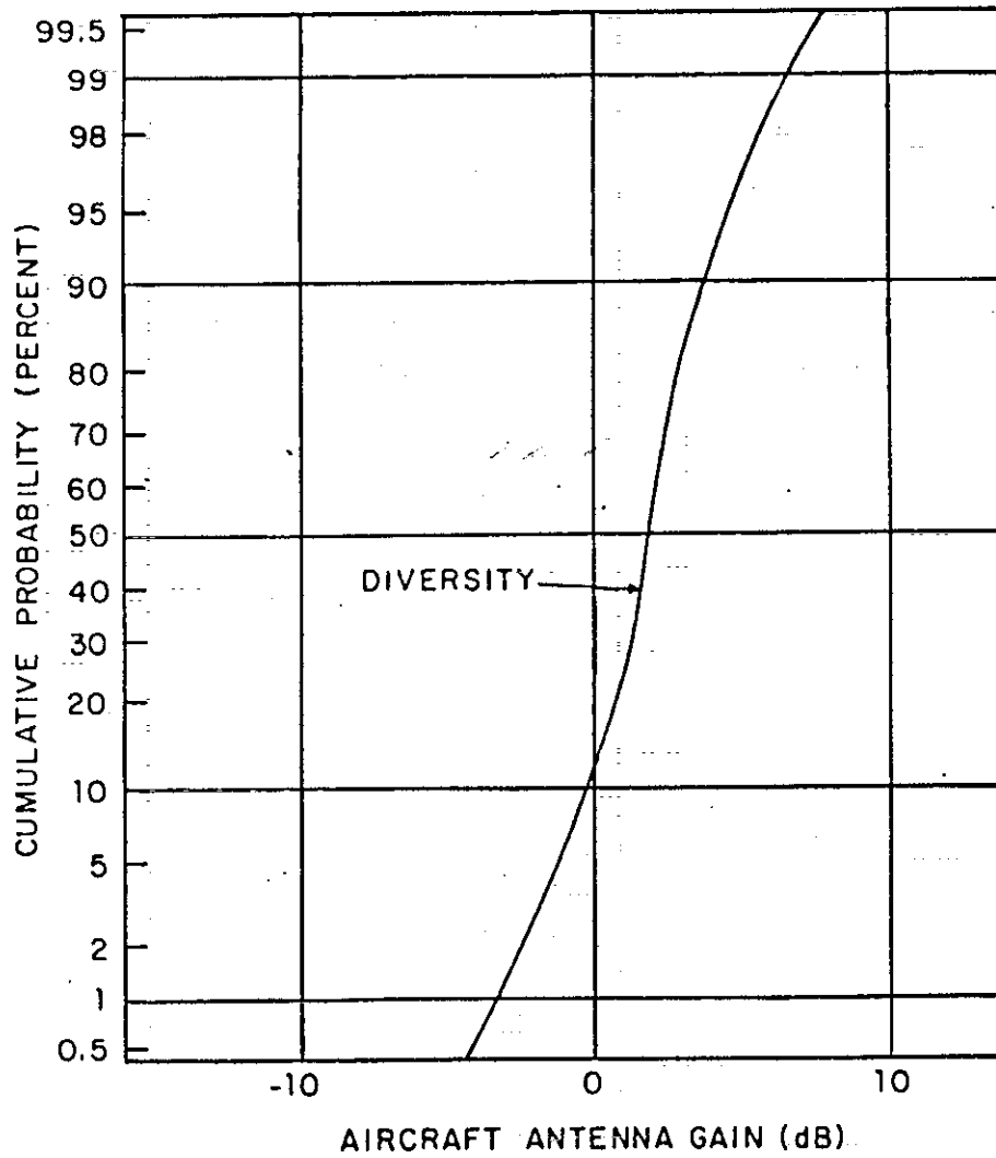
Fig. 8. Aircraft antenna summary statistics.
