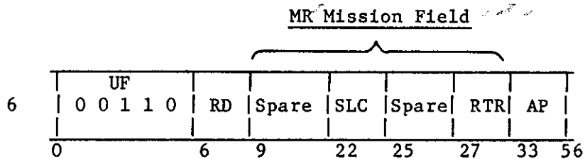
(b) RBX Reply Format
