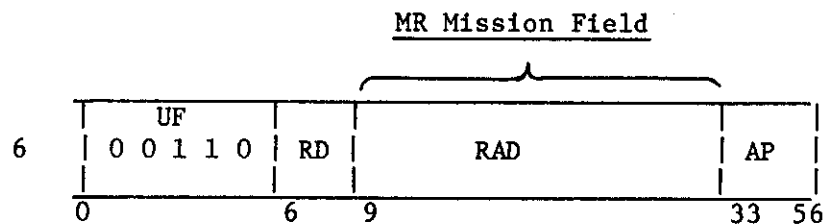
(a) RBX Squitter Format
