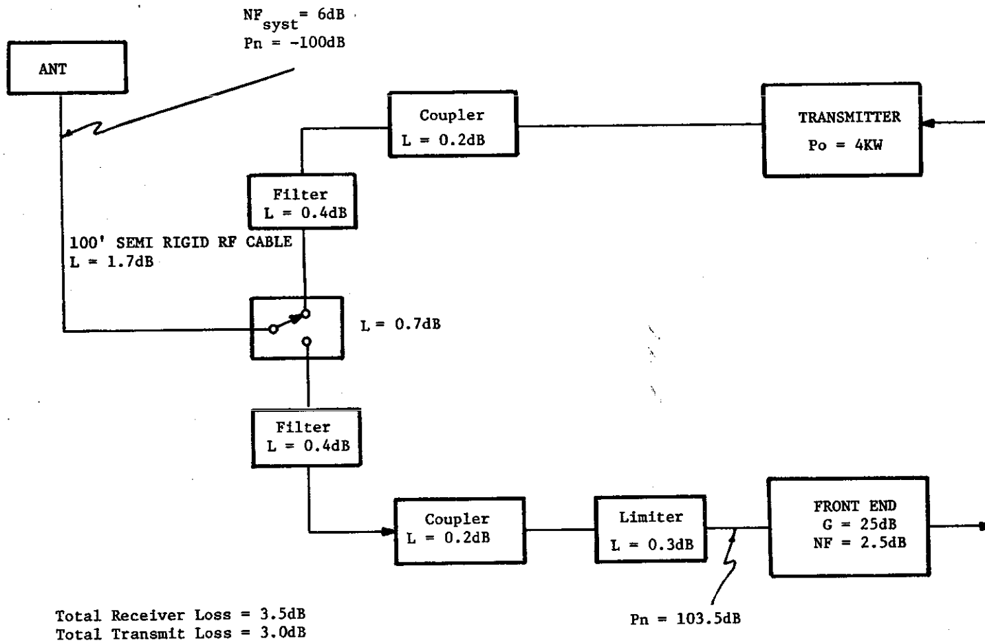
Fig. 5. Example of an RBX front end.
