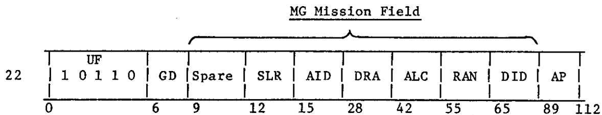
(c) BCAS Interrogation Format
