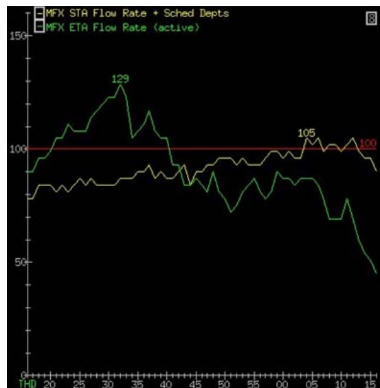
Figure 2-3. TMA load graph for ATL, showing projected ETA and STA flow rates for the next hour. The airport acceptance rate for this period is shown by the red line.
