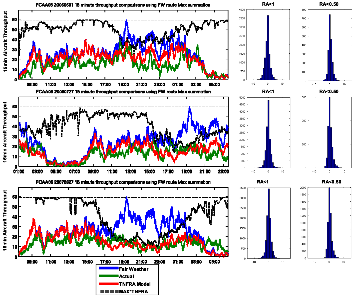
Figure 3-5. AFP throughput estimates compared to the actual 15 minute throughput across FCAA05 for the three high impact weather events: 01 June 2006, 27 July 2006, and 27 June 2007. The green line represents the actual 15 minute AFP filtered throughput that occurred on each of the three weather impacted days. The blue line represents the AFP filtered fair weather throughput estimate derived by summing the 15 minute route maximum of the three fair weather days centered at each one minute time step. The red line in the time series represents the TNFRA reduction of the fair weather estimate and is the model for assessing weather impact. The thick black dotted line is the TNFRA reduction relative to the single value maximum observed fair weather throughput (thin dashed line) and is meant to represent a measure of potential achievable capacity given weather impacts in the AFP domain. The histogram bin amplitudes represent the number of times the difference between a route's actual throughput and the route availability estimate is observed. The positive side of the histogram indicates that the route availability overestimated the weather impact on a route's throughput at any given time; the negative side of the histogram indicates the underestimate. The first column of histograms (left side) shows the occurrence distribution of these differences over all instances where route availability indicates weather impact ( RA < 1.0 ). The second column of histograms (far right) compares the differences of a smaller set of instances with greater weather impact ( RA < 0.50 ).
