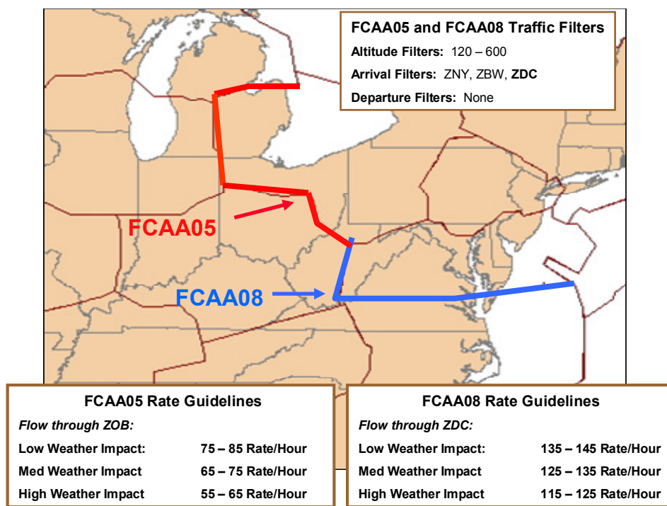
Figure 1-1. Location, traffic filters, and rate guidelines for AFP FCAA05 and FCAA08.
