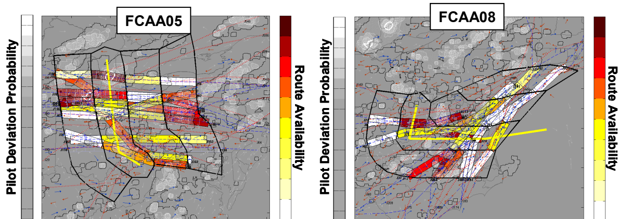
Figure 3-4. FCAA05 and FCAA08 AFP route availability at 1900 UTC on 27 June 2007. Low impacted routes are colored in white, deepening from yellow to shades of red for highly impacted routes. A muted grayscale overlay of WAFs for flight altitude of 35 kft (low WAF pilot deviation probabilities in gray, high deviation probabilities in white) and the 100% WAF contour (thick solid white contour) are also shown.
