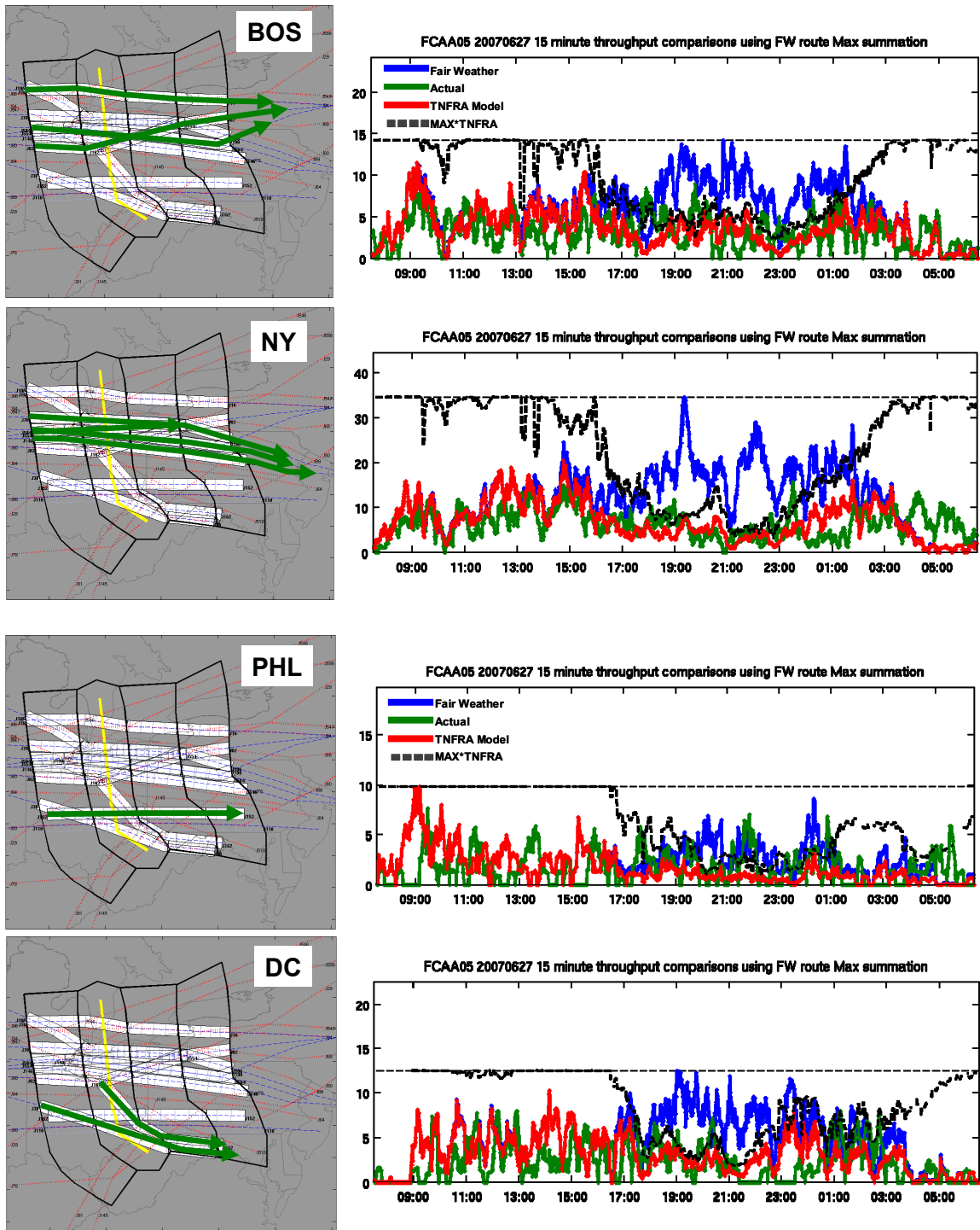
Figure 3-7. Tactical FCAA05 AFP throughput assessment, with route availability and usage (estimated vs. actual) deconstructed for individual traffic flows to Boston, metro-NY (EWR, LGA, and JFK), Philadelphia, and metro-DC (IAD, DCA, and BWI) airports. Throughput time series results (right-side) are presented as in Figure 3-6.
