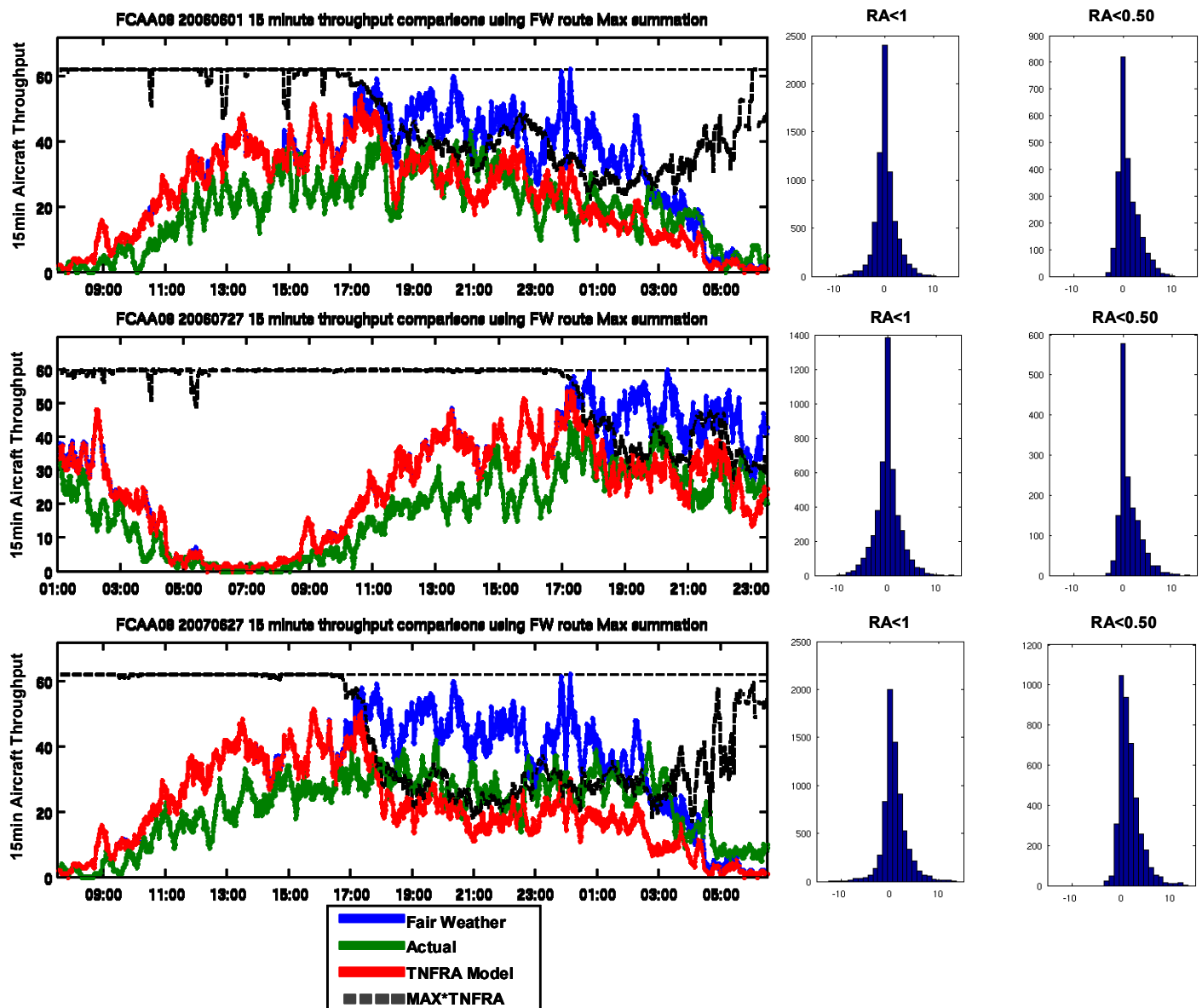
Figure 3-6. As in Figure 3-5, except for FCAA08.
