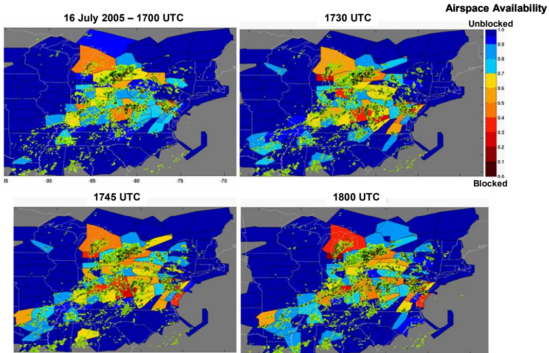
Figure 1-2. Variations in en route airspace sector capacities during convective weather on 16 July 2005. Note how rapidly airspace capacity can vary in both space and time. These capacity estimates were computed from CIWS precipitation and echo tops data by the algorithm described in Martin (2007). The colors indicate the estimated reduction in sector throughput, averaged across the jet routes traversing each section.
