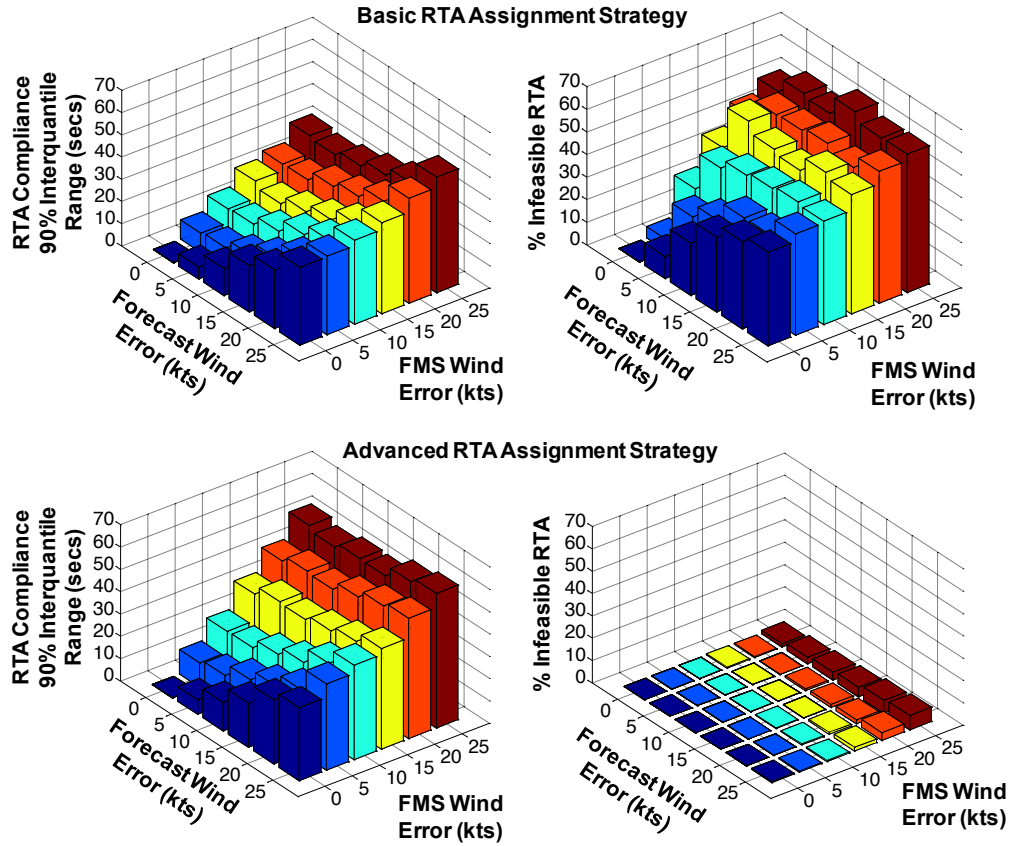
Figure 21. RTA Compliance 90% Interquartile Range (left), % Infeasible RTAs (right), and as a Function of Forecast Wind and FMS Wind Error for the Basic (top) and Advanced (bottom) RTA Assignment Strategy
