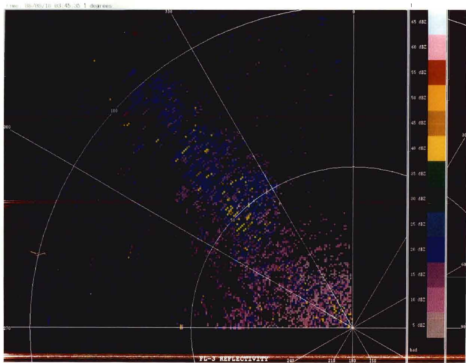
Figure I-2. FL-3 raw reflectivity output for same event as Figure I-1, showing spatial variance of anomalous propagation.
