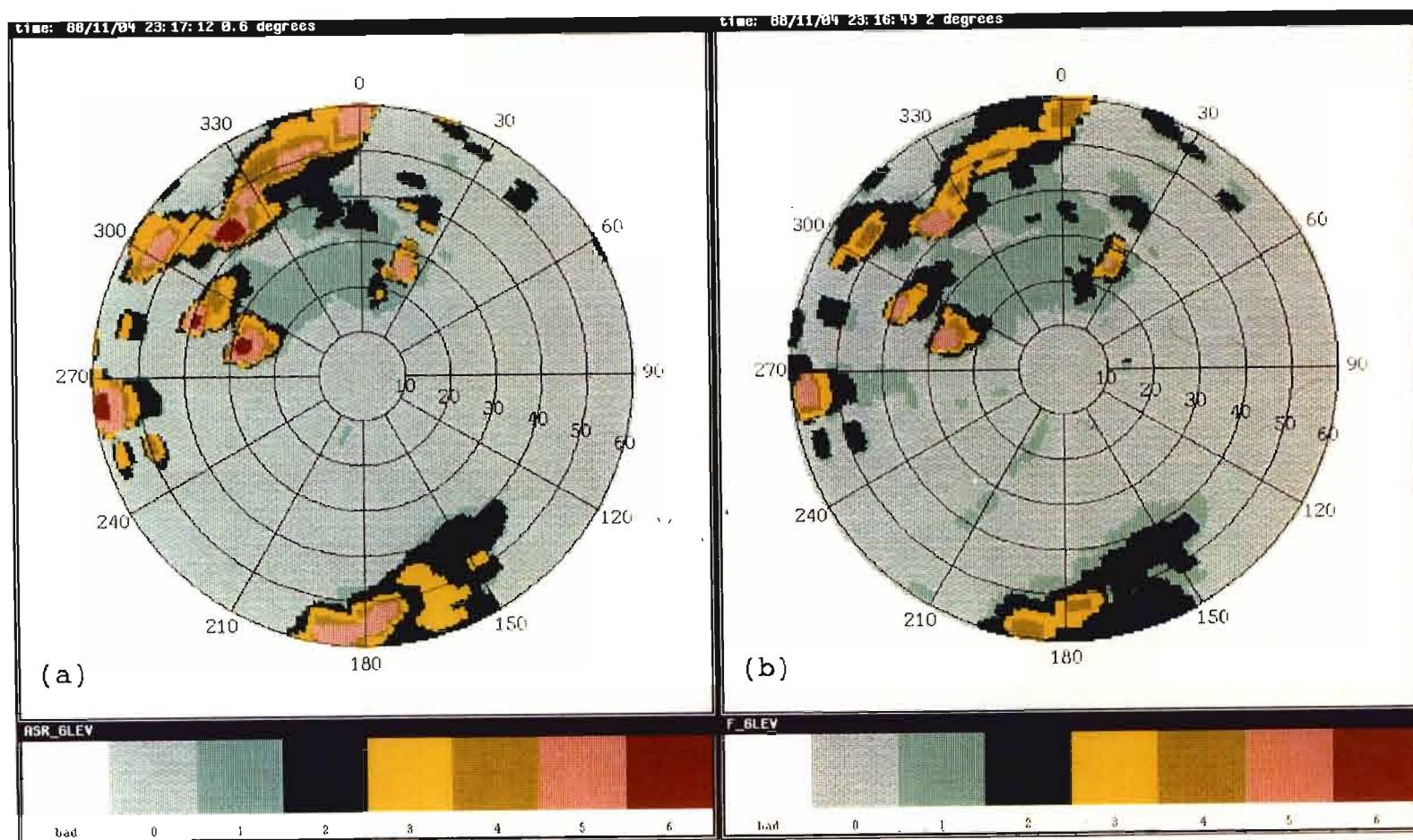
Figure 3-12. Comparison between (a) ASR-9 six-level CP and (b) emulation data, cold front, 4 November 1988. Although the PPIs show good spatial agreement, several of the ASR-9 weather contours are one level higher than the emulation data.
