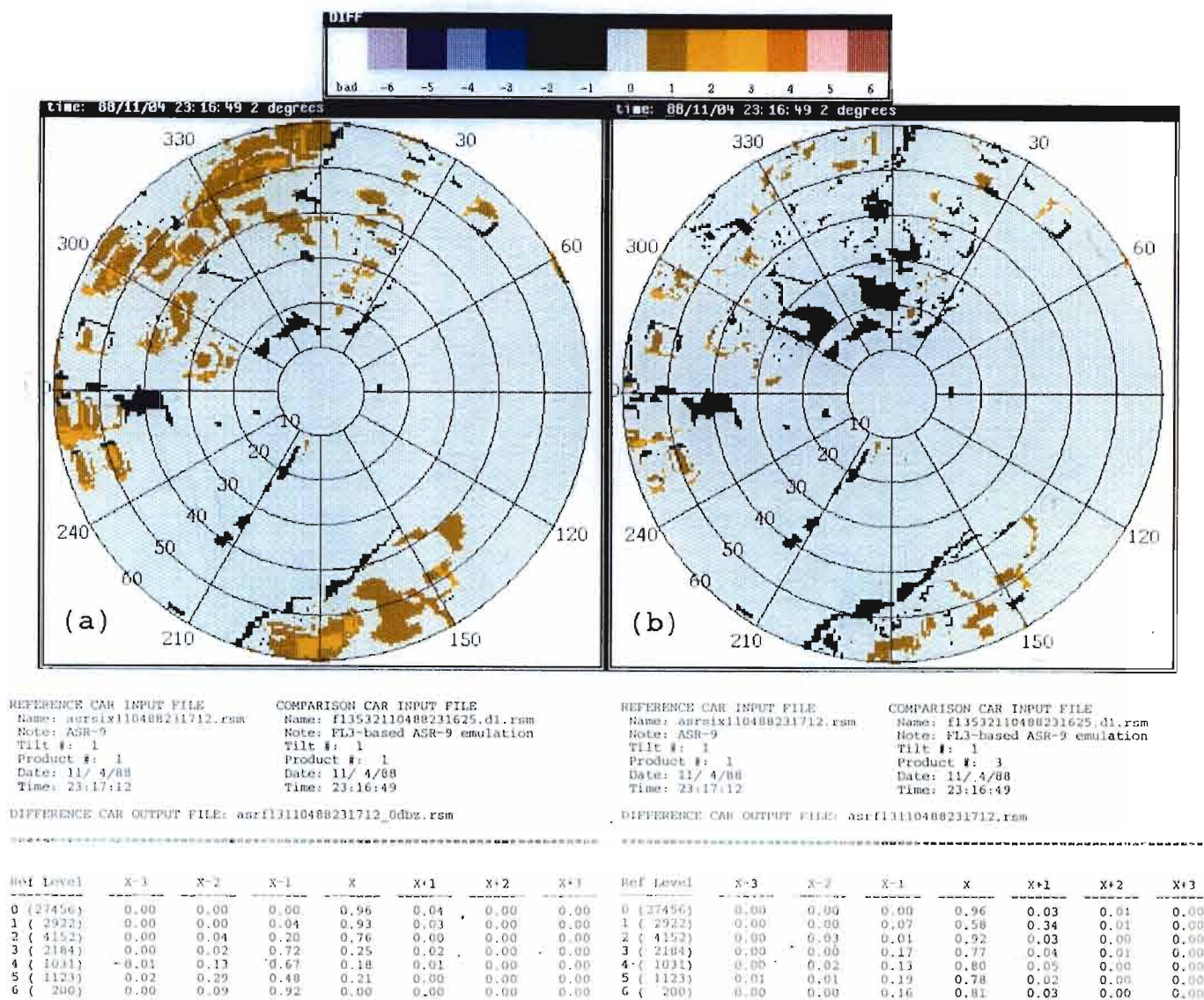
Figure 3-14. Reflectivity difference between ASR-9 six-level CP and emulation data increased by (a) 0 and (b) 3 dB, cold front, 4 November 1988. Statistics show, when the emulation data is increased by 3 dB, there is a significant decrease in the probability of differences of two levels (see column X-2) and the two radars are generally within one NWS level.
