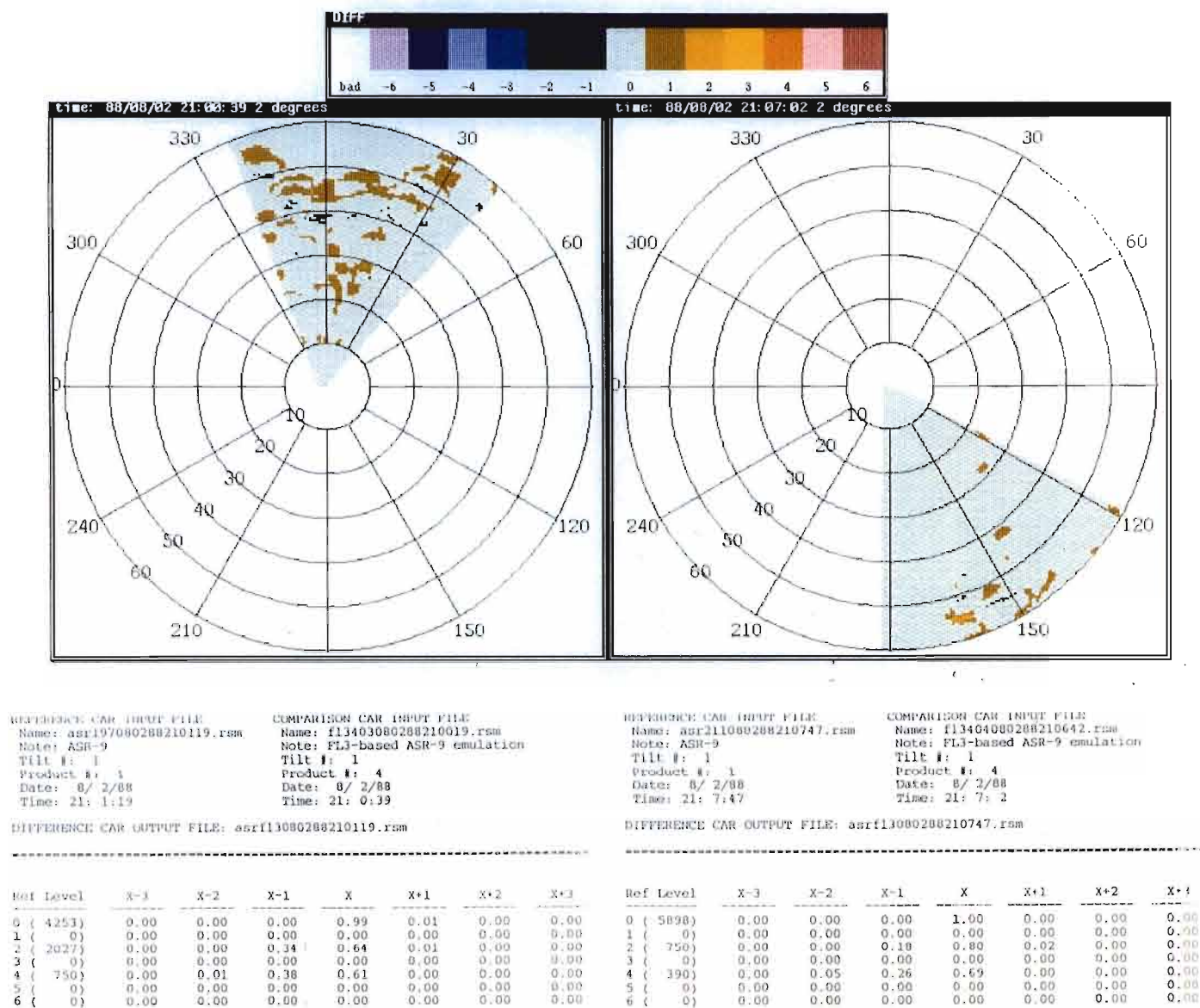
Figure 3-3. Reflectivity difference between ASR-9 two-level and emulation data, two convective storms, 2 August 1988. Both the difference plots and associated statistics indicate good agreement among the three radars.
