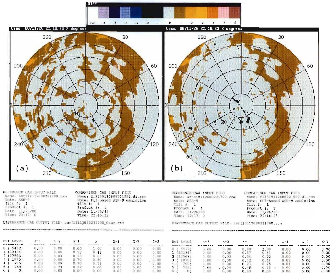
Figure 3-17. Reflectivity difference between ASR-9 six-level LP and emulation data increased by (a) 0 and (b) 3 dB, squall line, 26 November 1988. Statistics show that when the emulation data is increased by 3 dB, there is a significant decrease in the probability of two-level and one-level differences, while the two radars are generally within one NWS level.
