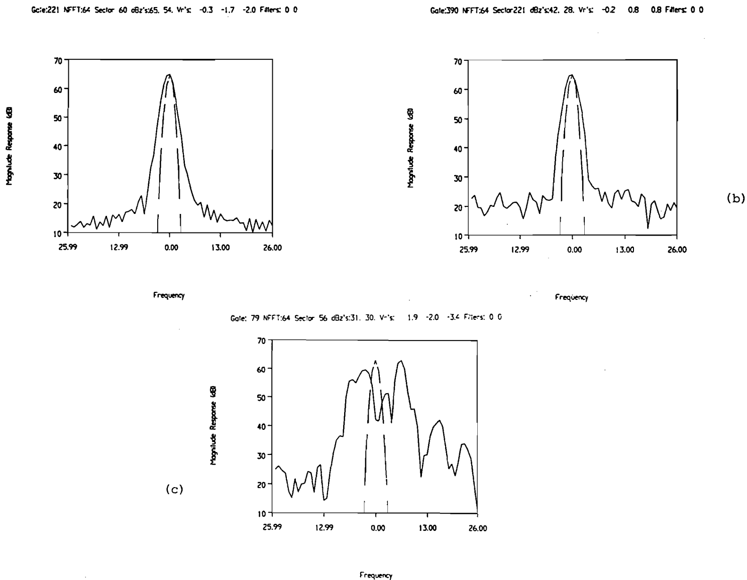
Figure I-4. Typical spectral characteristics of clutter, AP, and zero mean velocity weather; (a) Clutter spectrum, (b) AP spectrum, (c) Weather spectrum.
