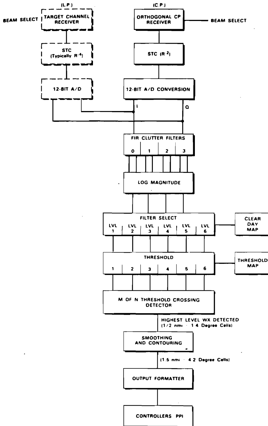
Figure 1-2. ASR-9 Weather Channel Processor Block Diagram.
