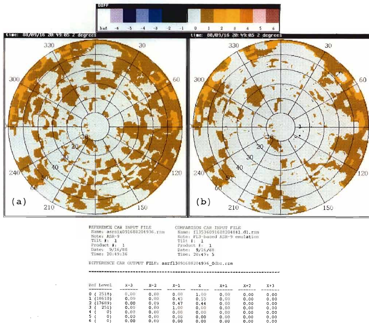
Figure 3-11. Reflectivity difference between ASR-9 six-level and emulation data increased by (a) 0 and (b) 3 dB, stratiform rain, 16 September 1988. Statistics show much better agreement between the two data products as was found without the 3 dB increase. The remaining discrepancy between Level 1 weather produced by both radars is assumed to be due to a difference in sensitivity between the two radars and threshold settings.
