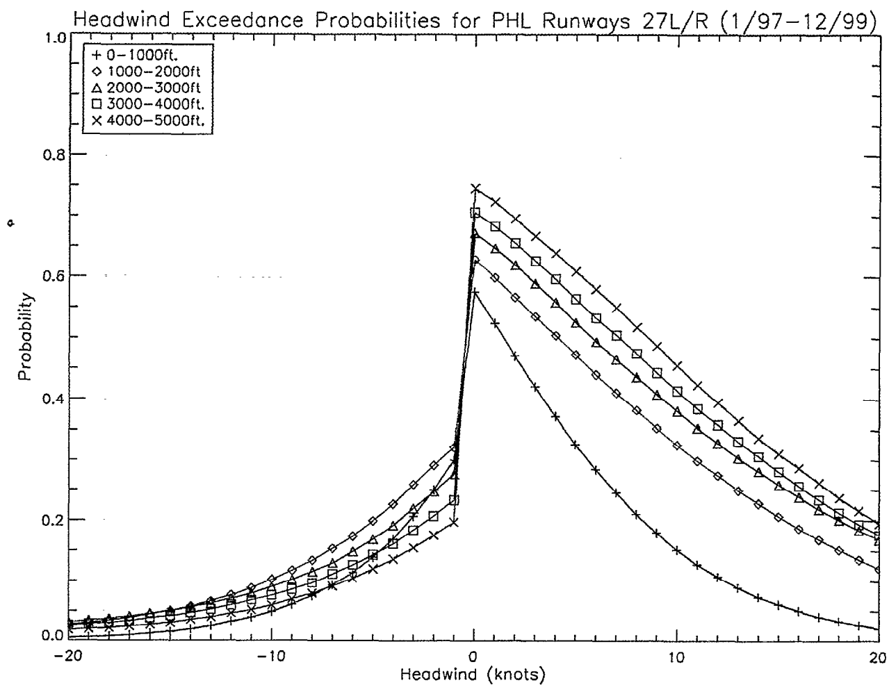
Figure 14. Headwind exceedance probabilities for PHL comparing 1000-foot layers between 0-5000 feet.
