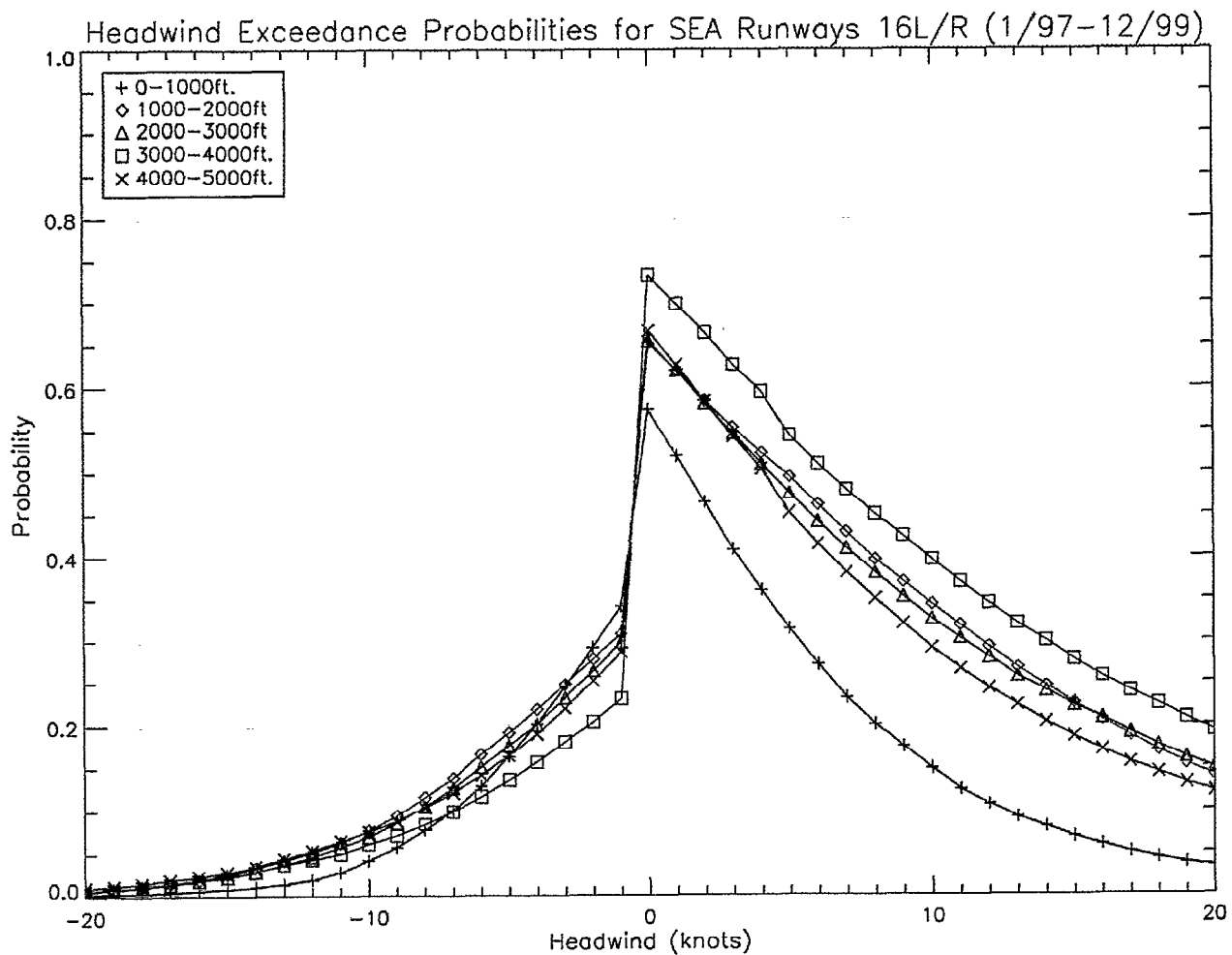
Figure 18. Headwind exceedance probabilities for SEA comparing 1000-foot layers between 0-5000 feet.
