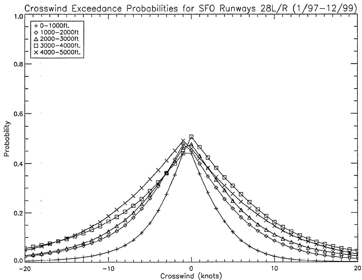
Figure 4. Crosswind exceedance probabilities for SFO comparing 1000-foot layers between 0-5000 feet.
