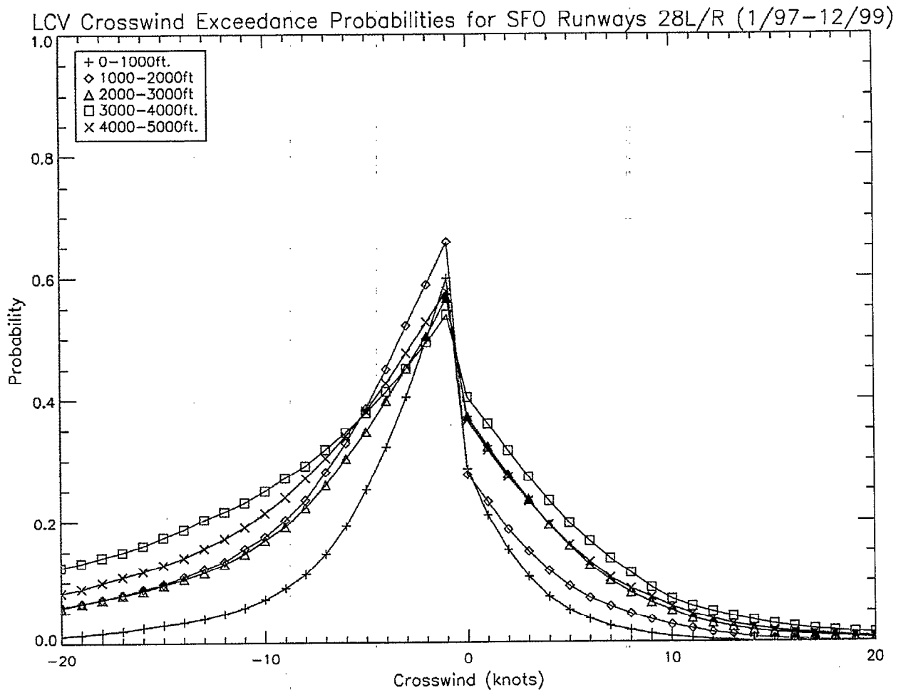
Figure 5. Crosswind exceedance probabilities for SFO during LCV conditions.
