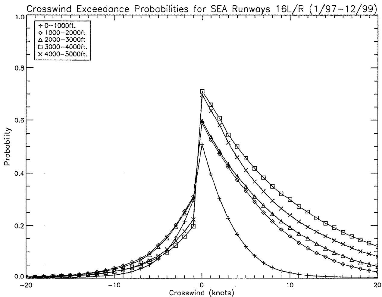
Figure 20. Crosswind exceedance probabilities for SEA comparing 1000-foot layers between 0-5000 feet.
