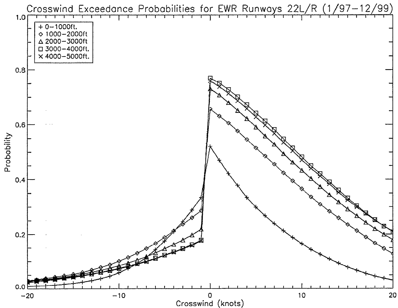
Figure 12. Crosswind exceedance probabilities for EWR comparing 1000-foot layers between 0-5000 feet.
