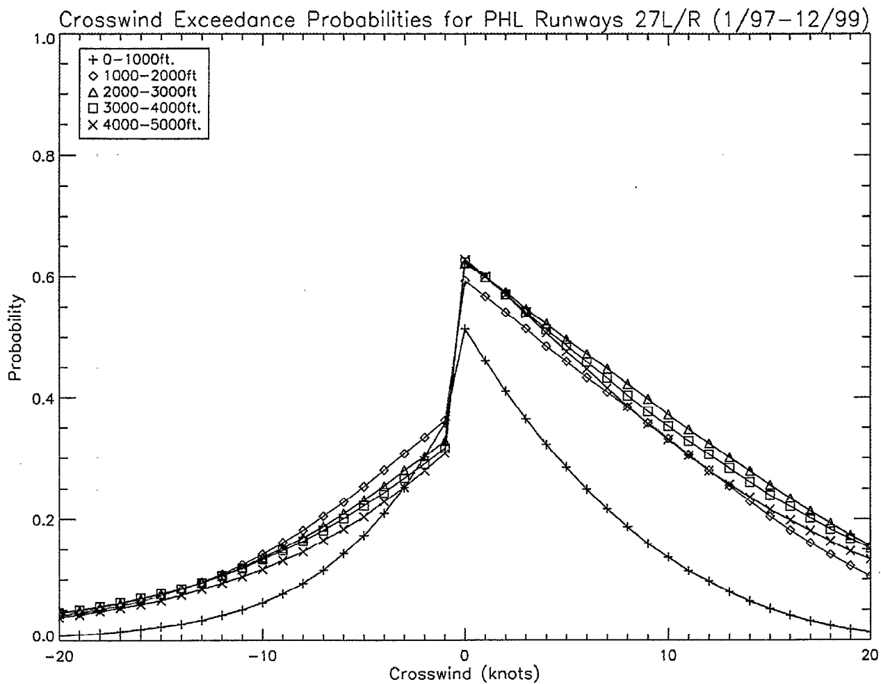
Figure 16. Crosswind exceedance probabilities for PHL comparing 1000-foot layers between 0-5000 feet.
