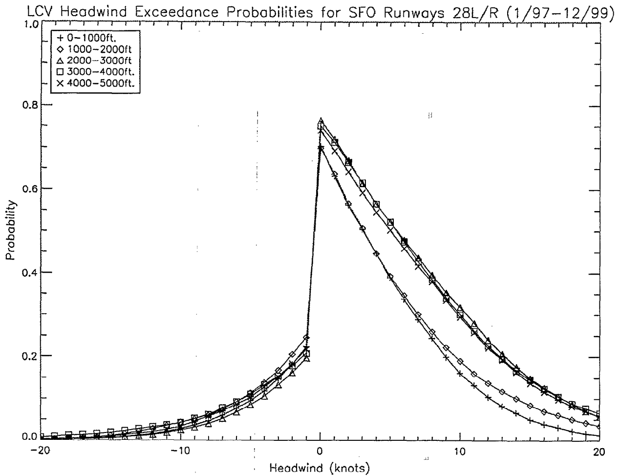
Figure 3. Headwind exceedance probabilities for SFO during LCV conditions.
