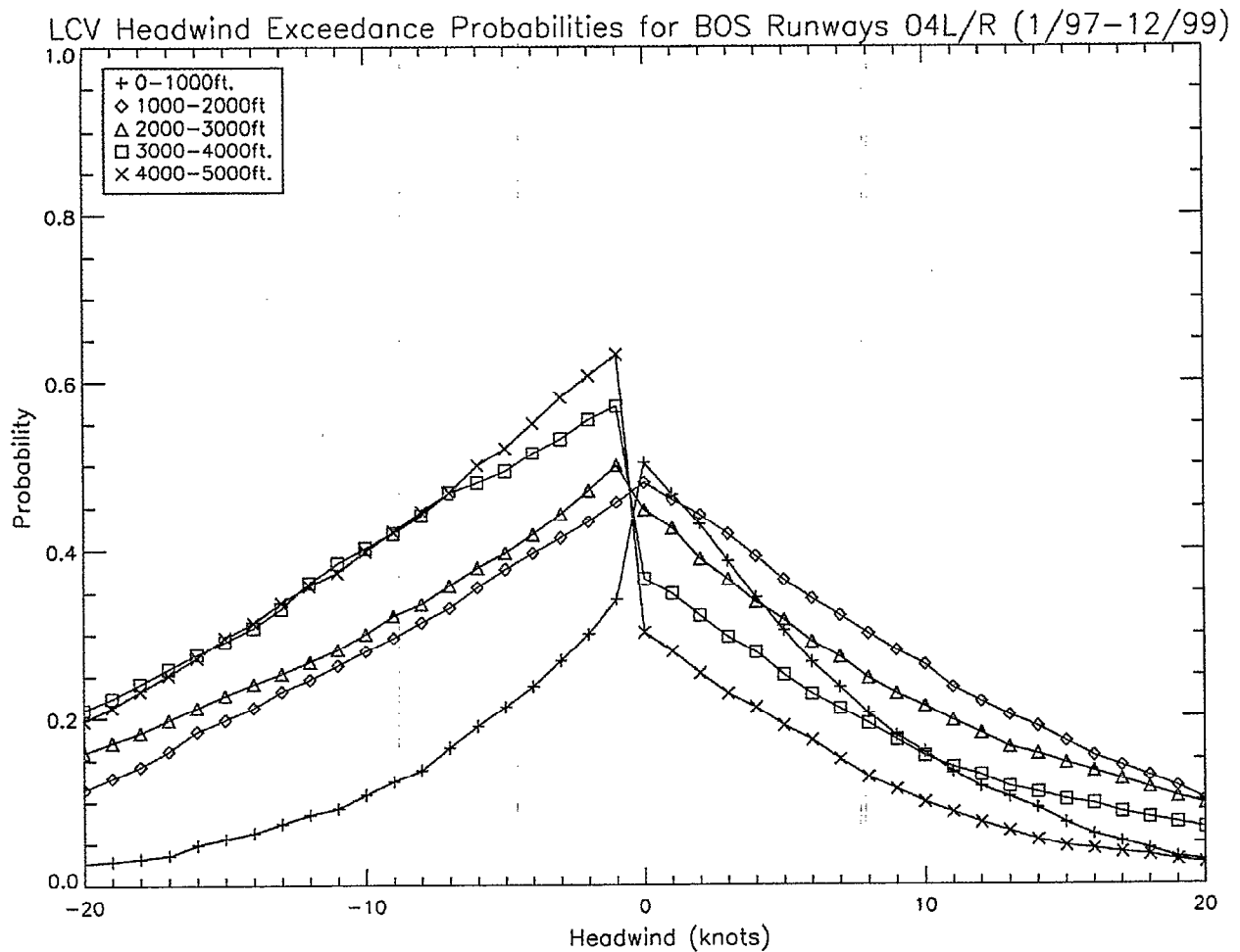
Figure 7. Headwind exceedance probabilities for BOS during LCV conditions.
