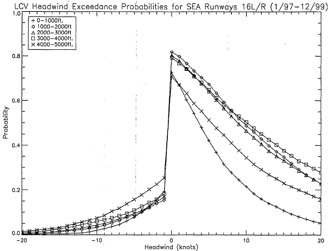
Figure 19. Headwind exceedance probabilities for SEA during LCV conditions.
