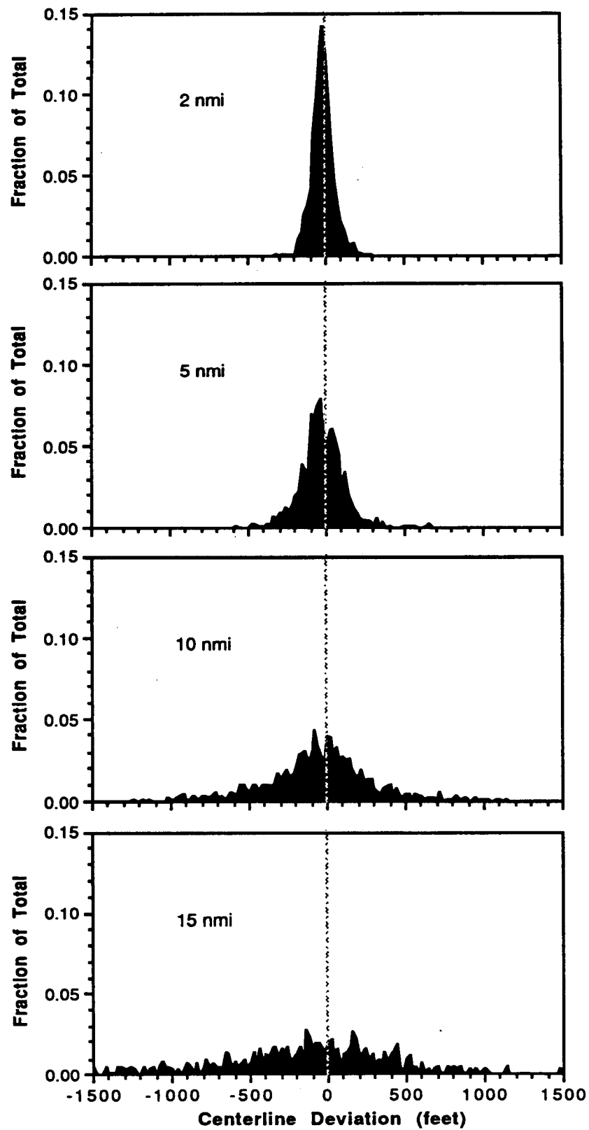
Figure 3-4. Distribution of ILS arrivals into Memphis in IMC (36L/R and 18L/R combined).
