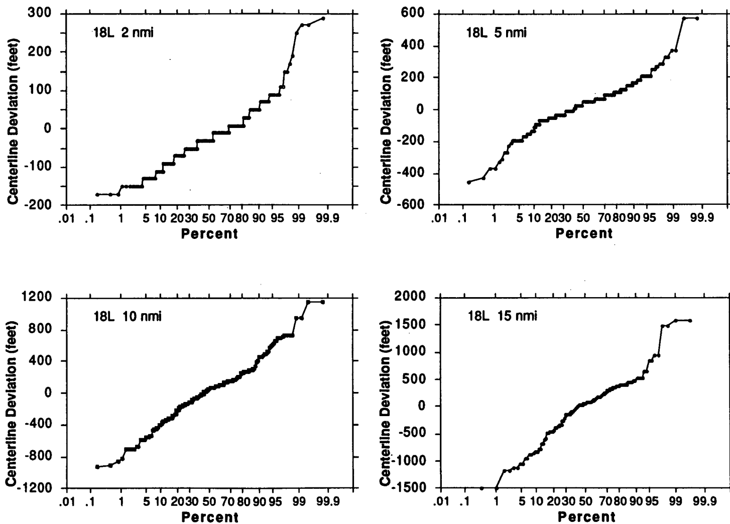
Figure B-7. The lateral deviations of Memphis IMC arrivals to 18L of aircraft over 12,500 lbs. plotted on a nonlinear probability scale. There were about 150 arrivals except at 15 nmi where there were 72 arrivals.
