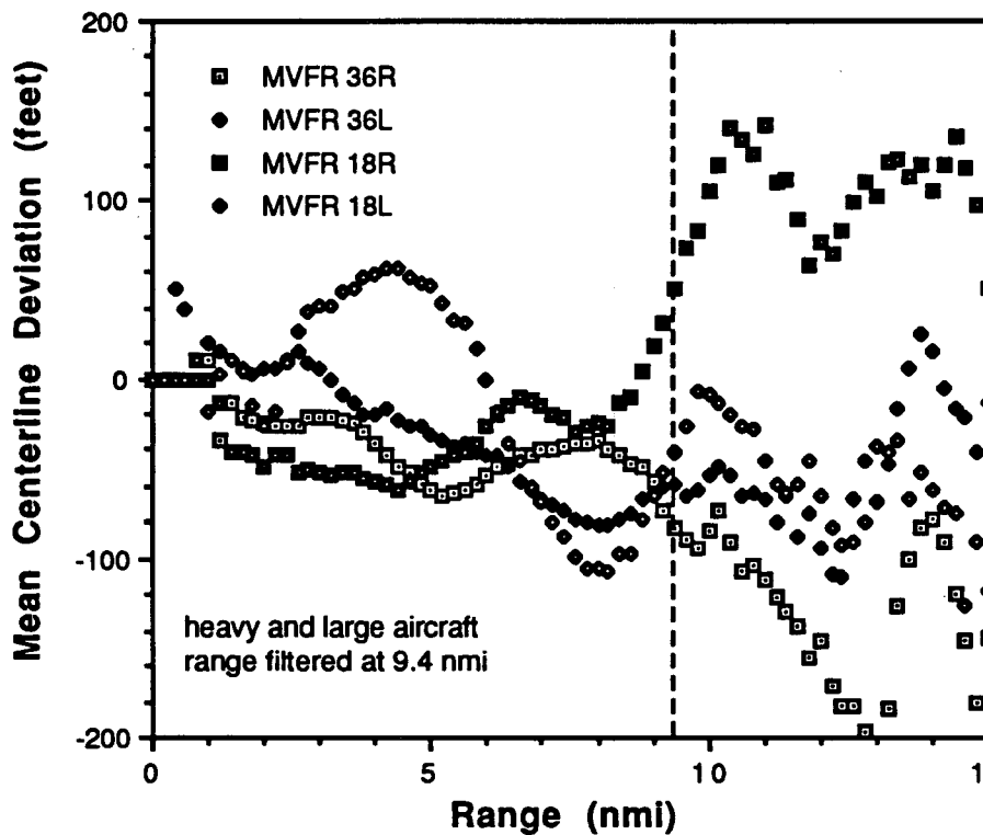
Figure 3-10. The mean centerline deviation of the arrivals to Memphis 36L/R and 18L/R in MVFR weather conditions.
