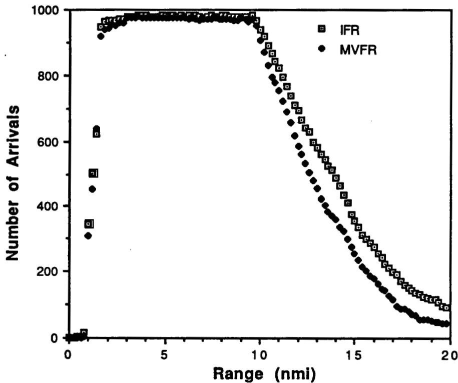
Figure 3-17. The number of aircraft over 12,500 lbs. arriving in Memphis in IFR and MVFR weather conditions, stabilized by 9.4 nmi.
