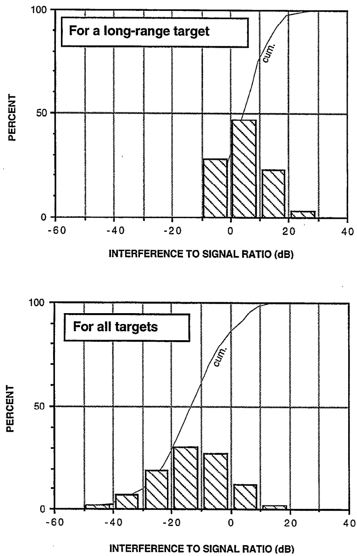
Figure 6. Power distributions of interfering receptions.
