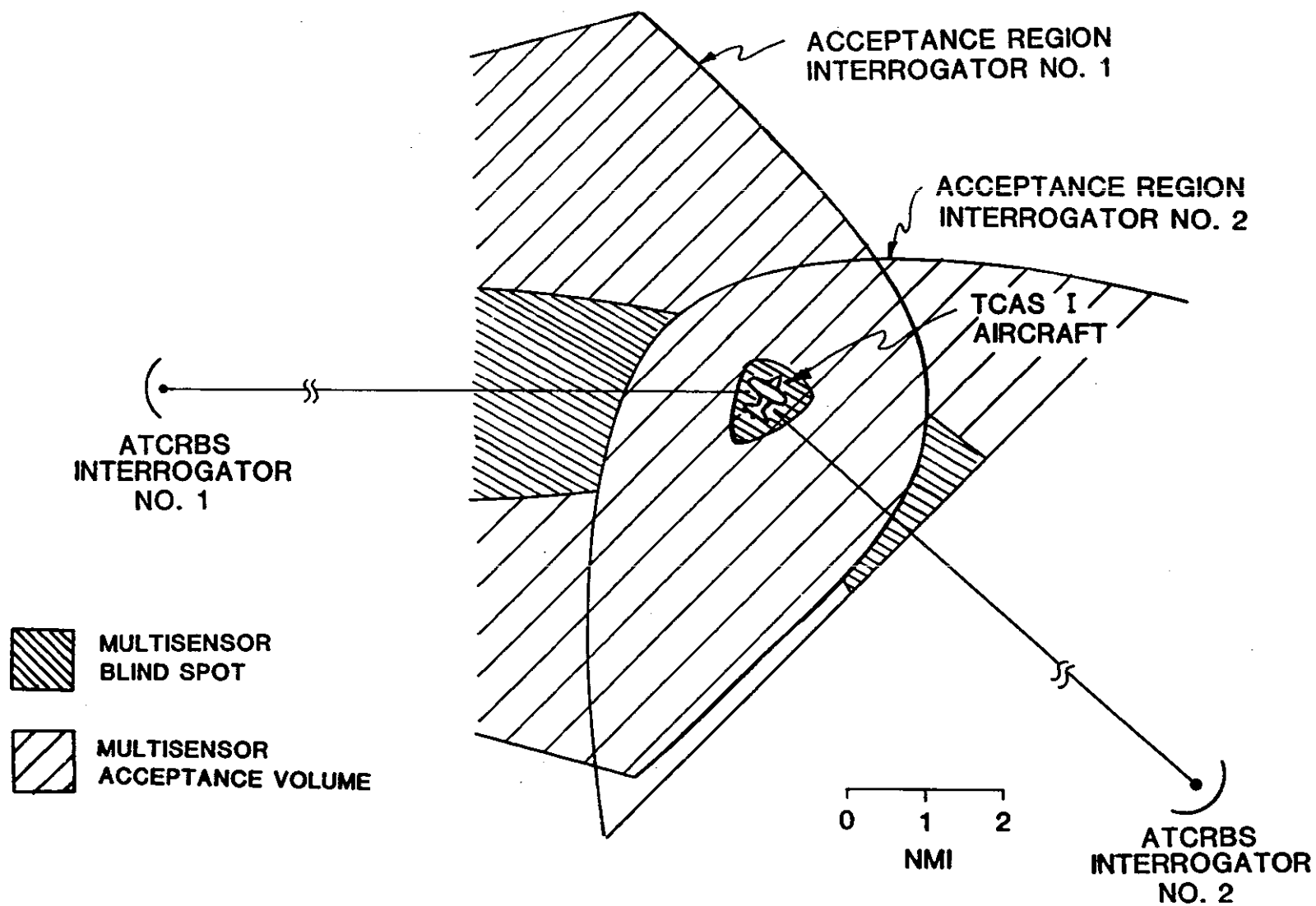
Fig. 4-12. Time-after-interrogation filter performance due to multiple interrogations.
