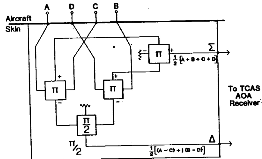
AOA HYBRID COMBINER
