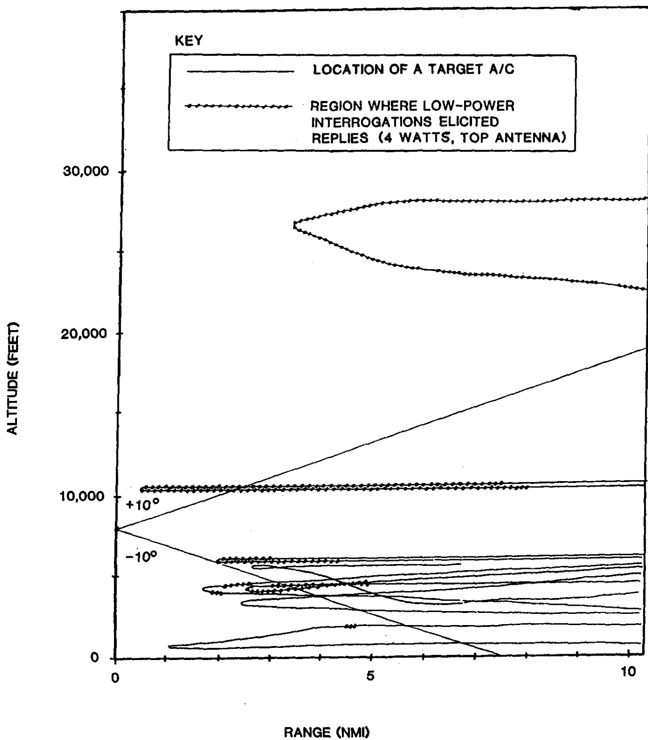
Fig. 7-1. Active TCAS I performance - Boston to New York.
