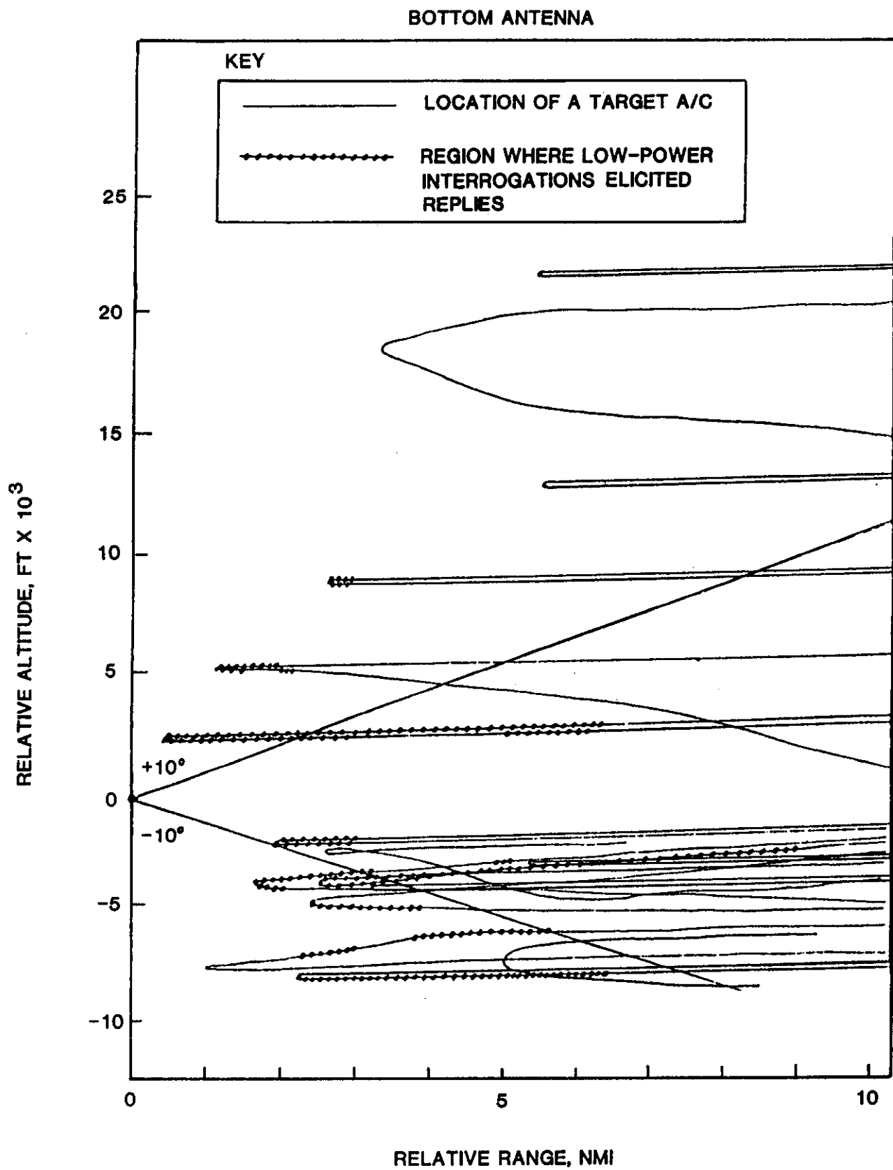
Fig. 4-6B. Antenna pattern filtering results, bottom antenna.
