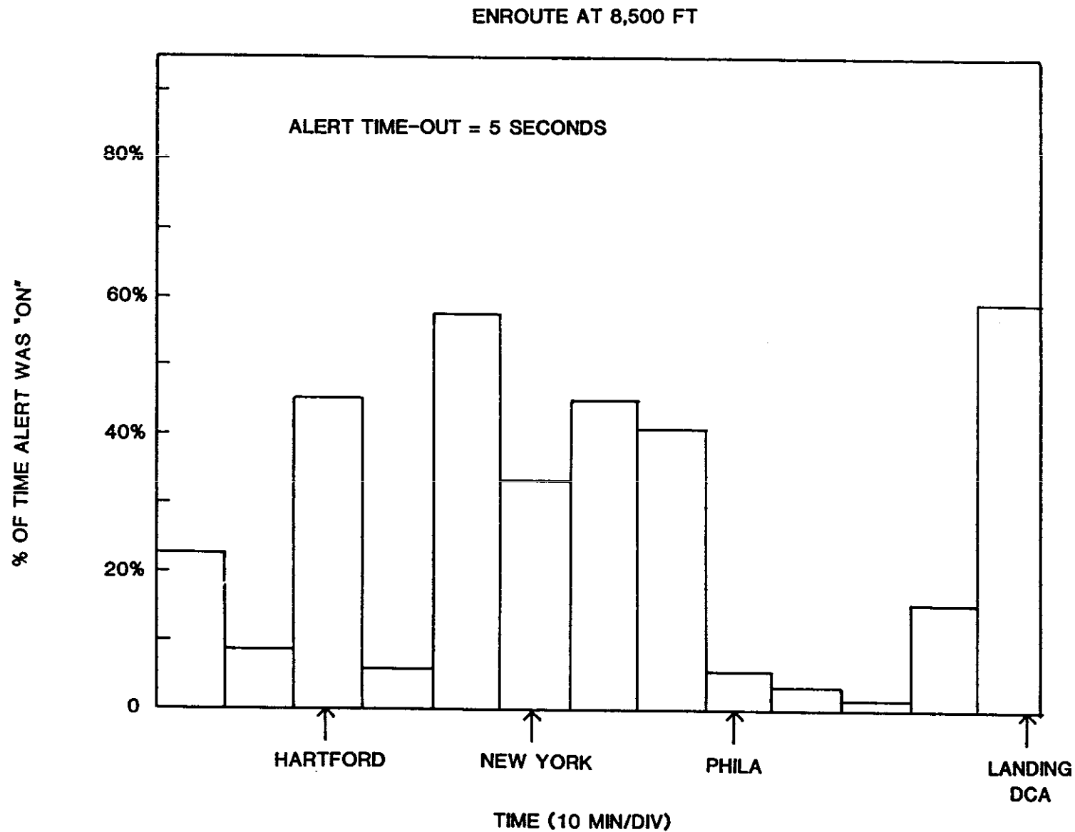
Fig. 6-11. Passive detector alert rate: Boston to Washington at 8,500 ft.
