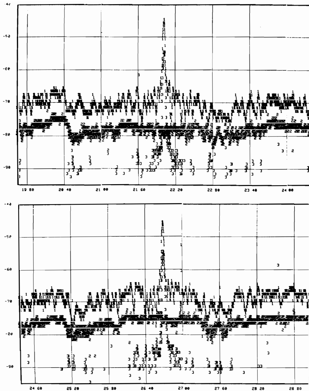
Fig. 3-2b. Antenna Pattern, Composite - Philadelphia (ASR-7), 19.80-28.80 Secs.
