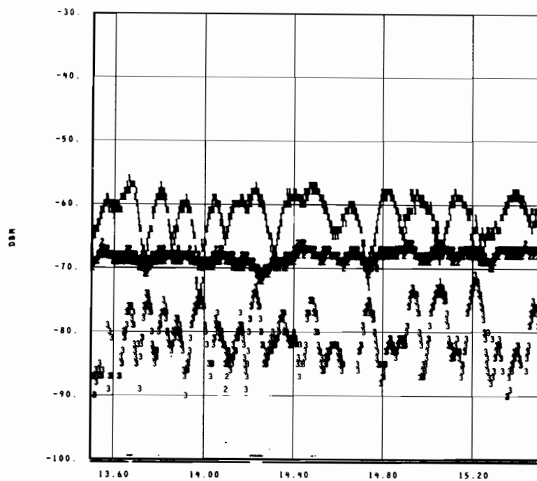
TIME JFK ARSR EL=22 ANF 7 NM E (12-16-77 14:49 K=10)
