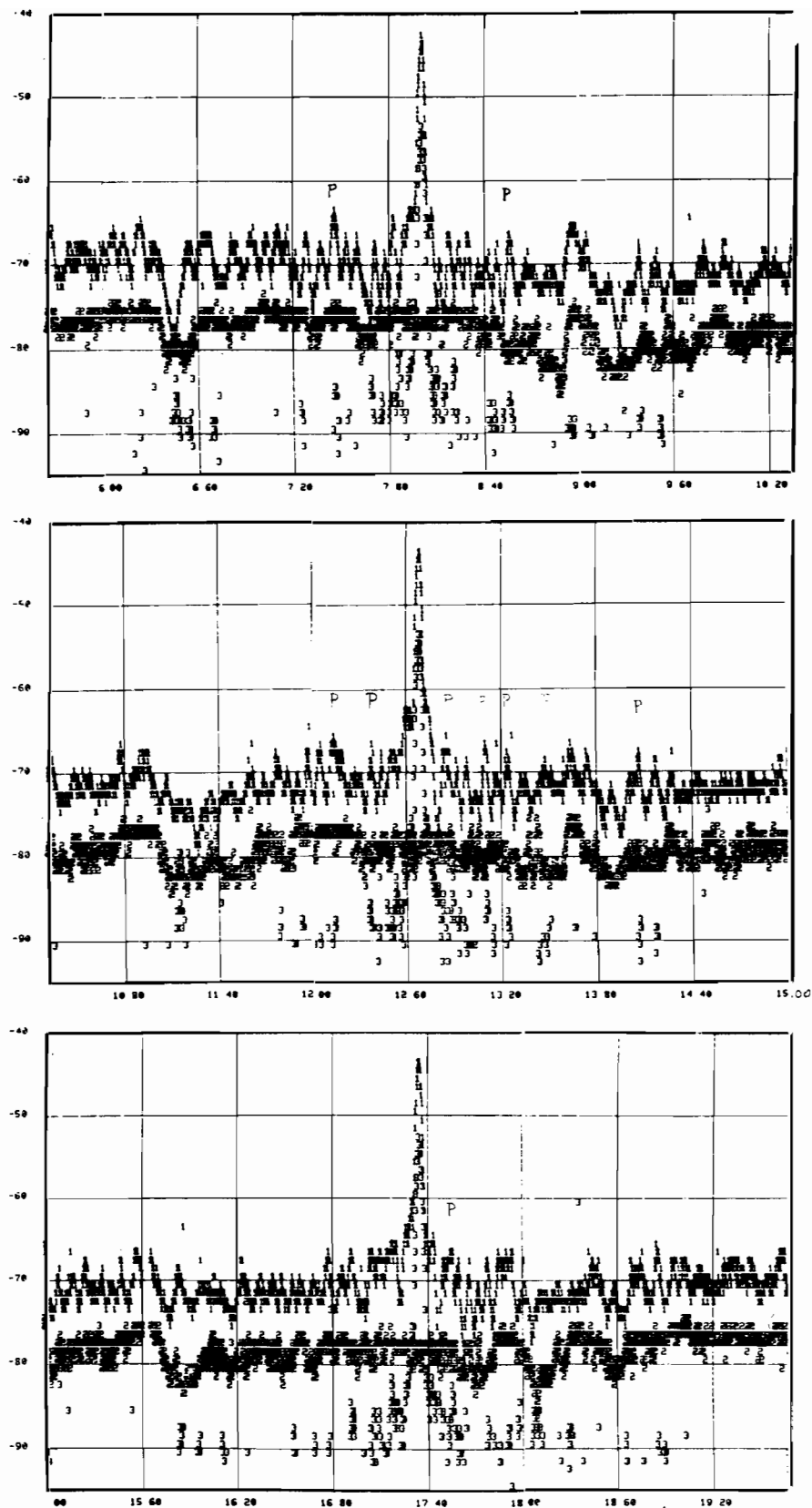
Fig. 3-2a. Antenna Pattern, Composite - Philadelphia (ASR-7), 6.00-19.20 Secs.
