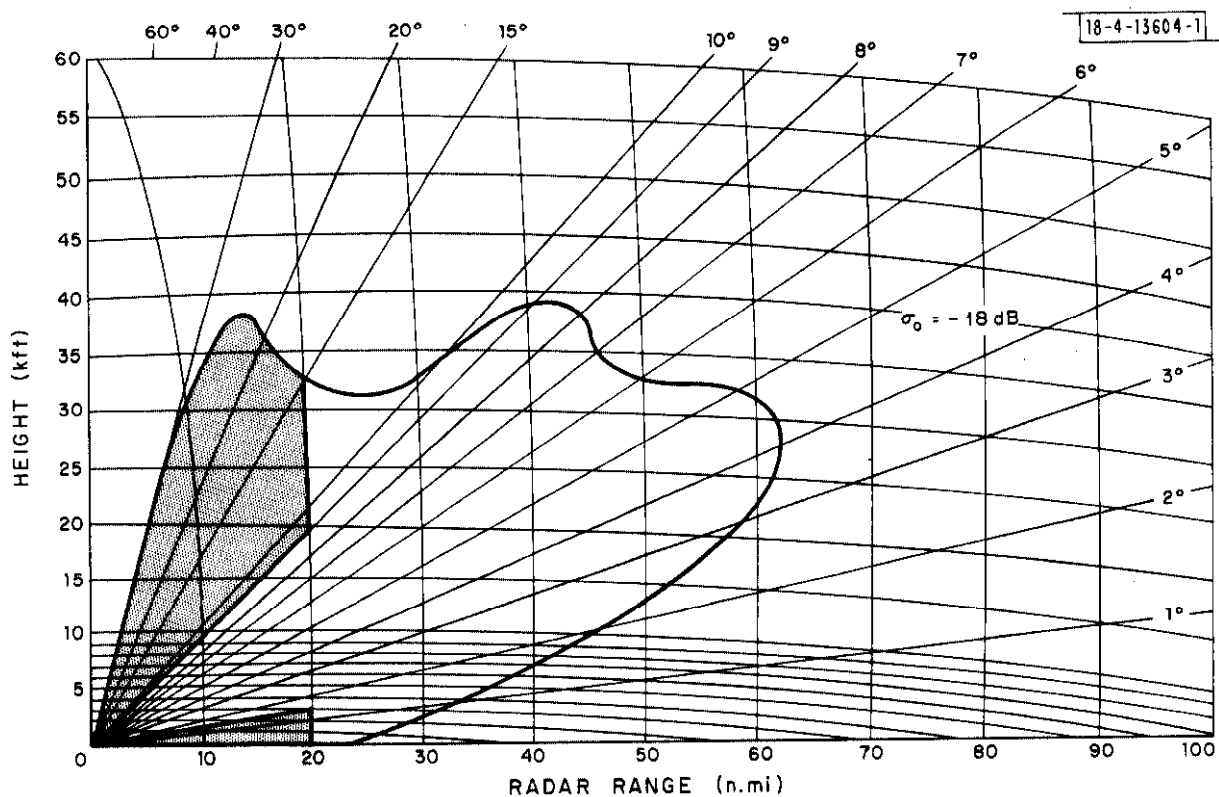
Figure 5. Solid Curve is Coverage of ASR-7 Radar Against a 2 \text{ m}^2 Target in Receiver Noise. (Ref. 3) Cross Hatched Region Shows Region of Poor Performance Against Ground Clutter.
