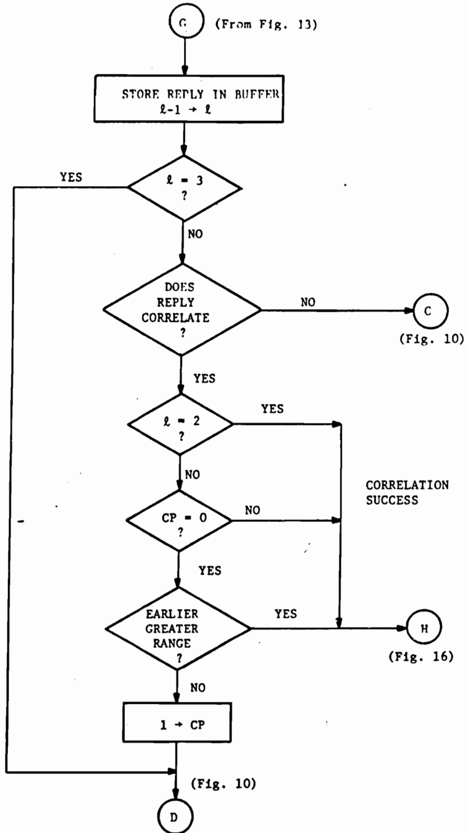
Fig. 15. Acquisition Processing (Cont.)
