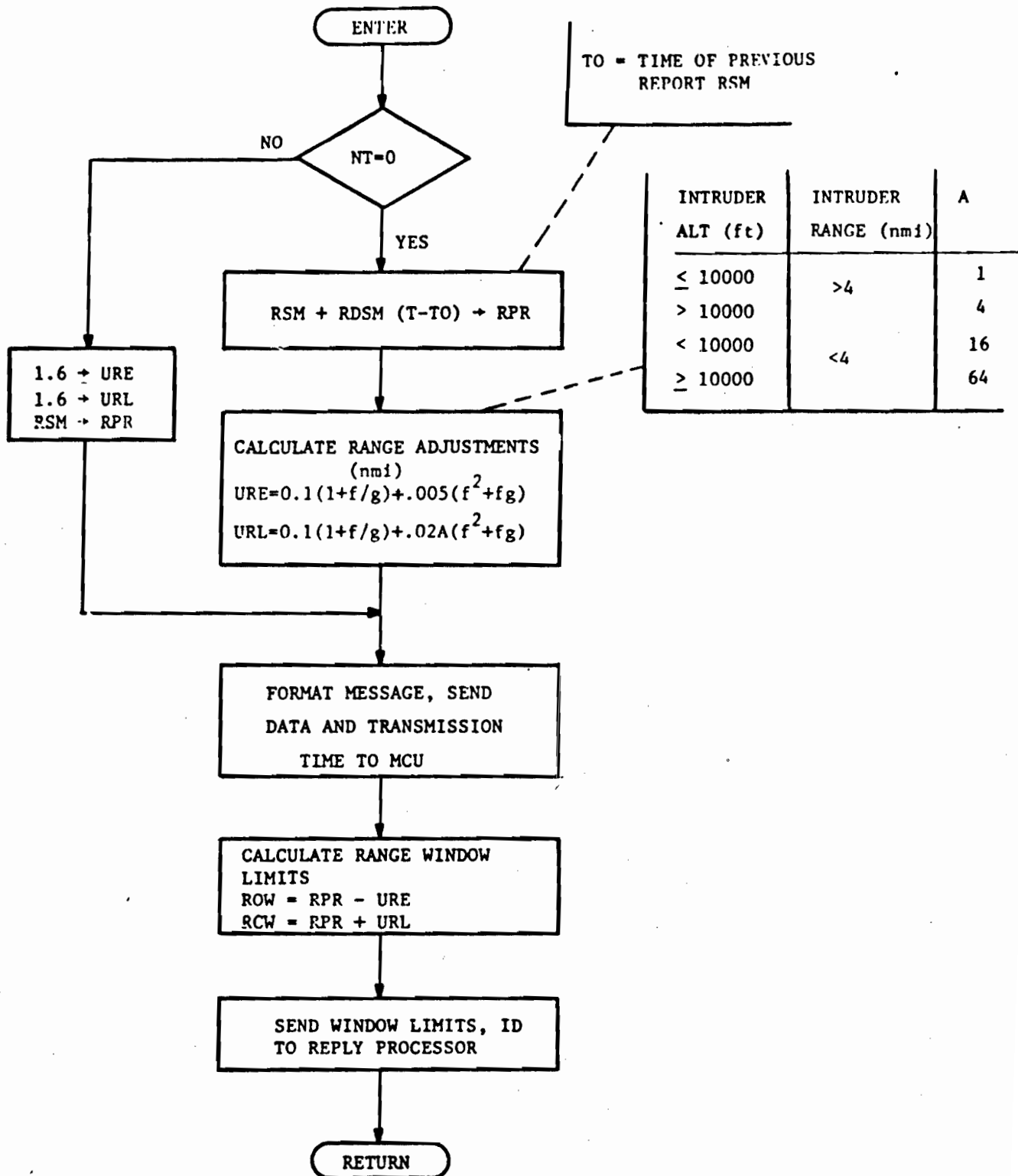
Fig. 19. Roll Call Processing - Interrogation Subroutine.
