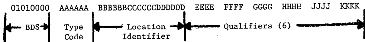
Fig. 4.1. Comm-B Message Field for Pilot Weather Requests.
