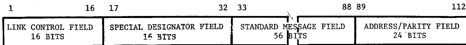
NORMAL (COMM-A, COMM-B)
