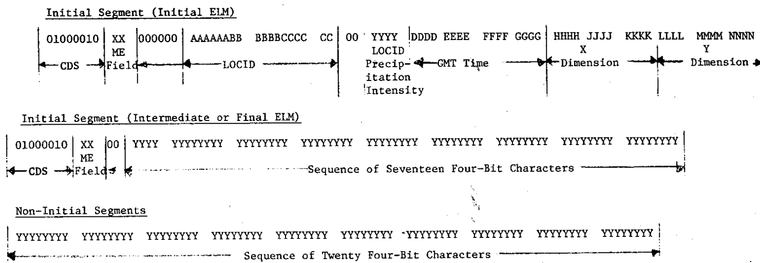
Fig. 4.5. Comm-C MC-Field for Digitized Weather Radar Map.
