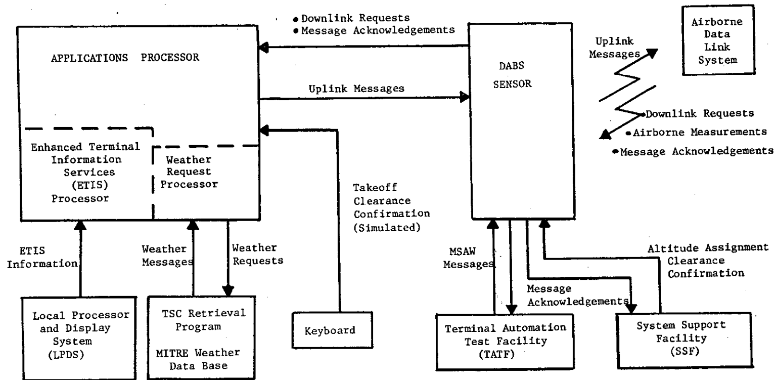
Fig. 1.1. DABS Data Link Communications Flow Diagram for NAFEC Tests and Evaluations.
