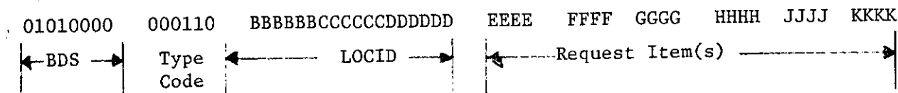
Fig. 5.1. Comm-B Message Field for ETIS Requests.
