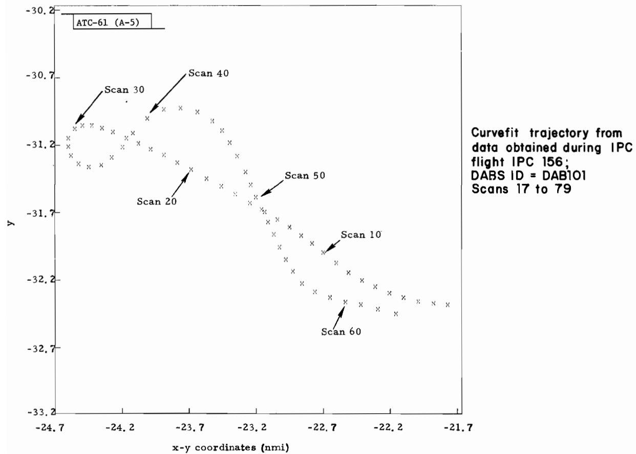
Fig. A-5. Ampersand maneuver of IPC flight 156
