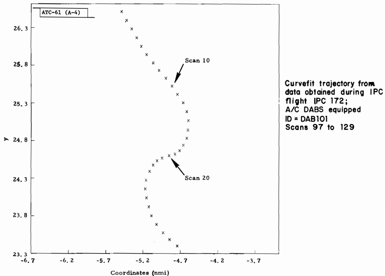
Fig. A-4. Reconstructed s-maneuver flown during an IPC test flight.
