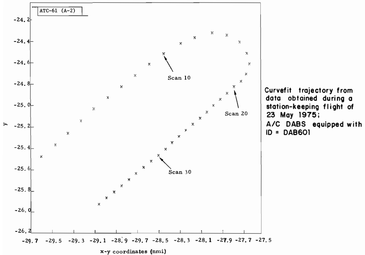
Fig. A-2. Reconstructed actual turn (Cherokee turning in wind).
