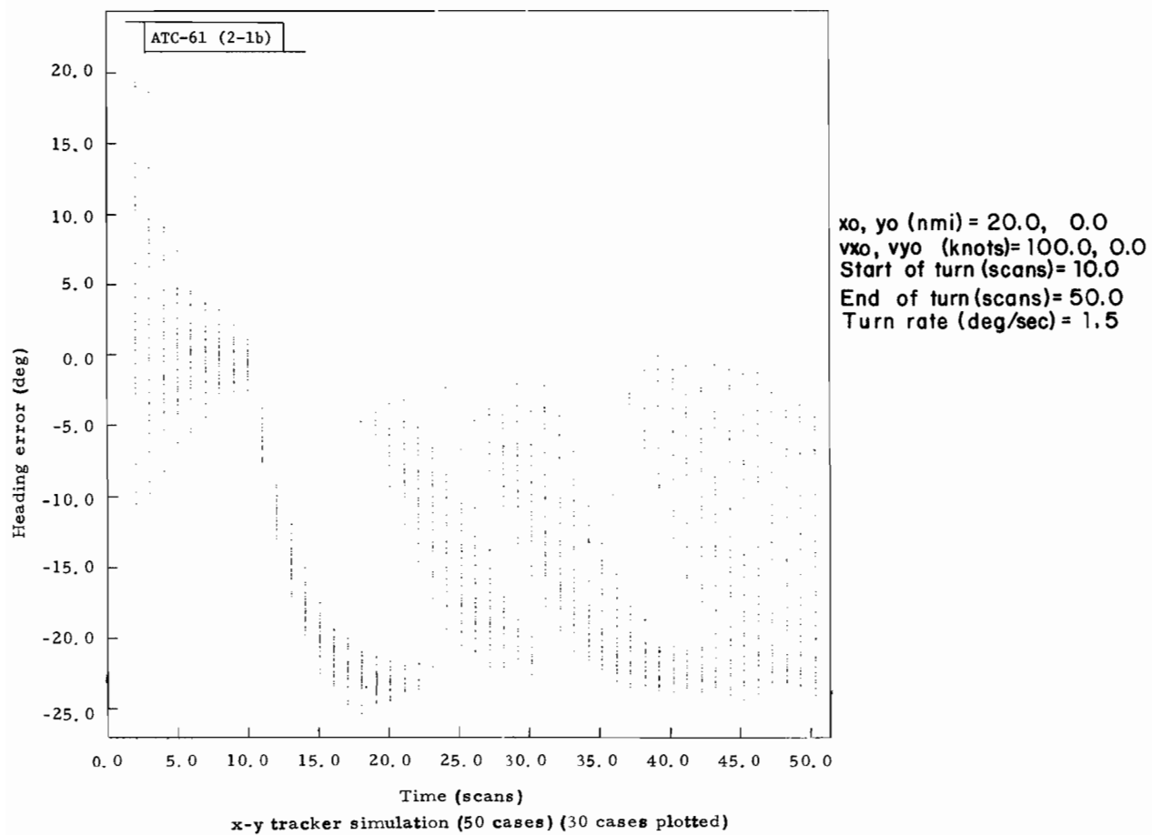
Fig. 2-1(b). Dynamic heading error vs scan ( 1.5^{\circ}/\text{sec} turn rate).
