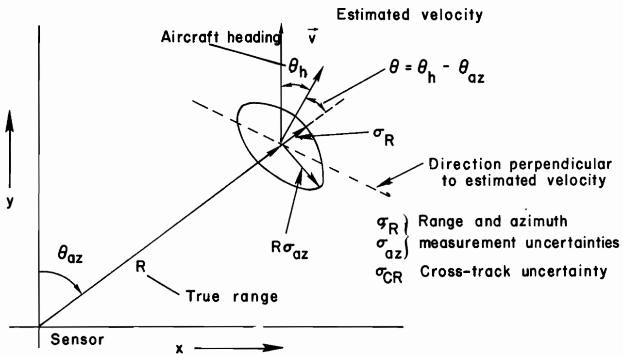
Fig. B-1. Cross-track uncertainty.
