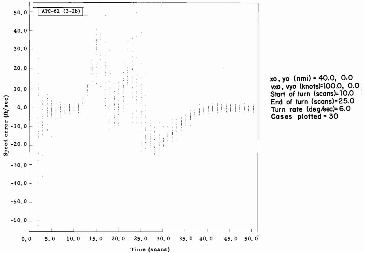
Fig. 3-2(b). Dynamic speed error vs scan for turn illustrated in Fig. A-1 (ideal turn).
