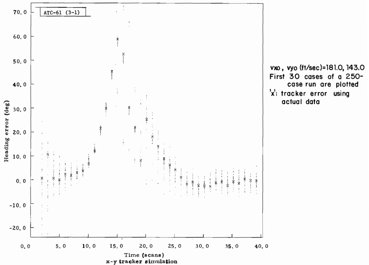
Fig. 3-1. Dynamic heading error vs scan for turn illustrated in Fig. A-2.
