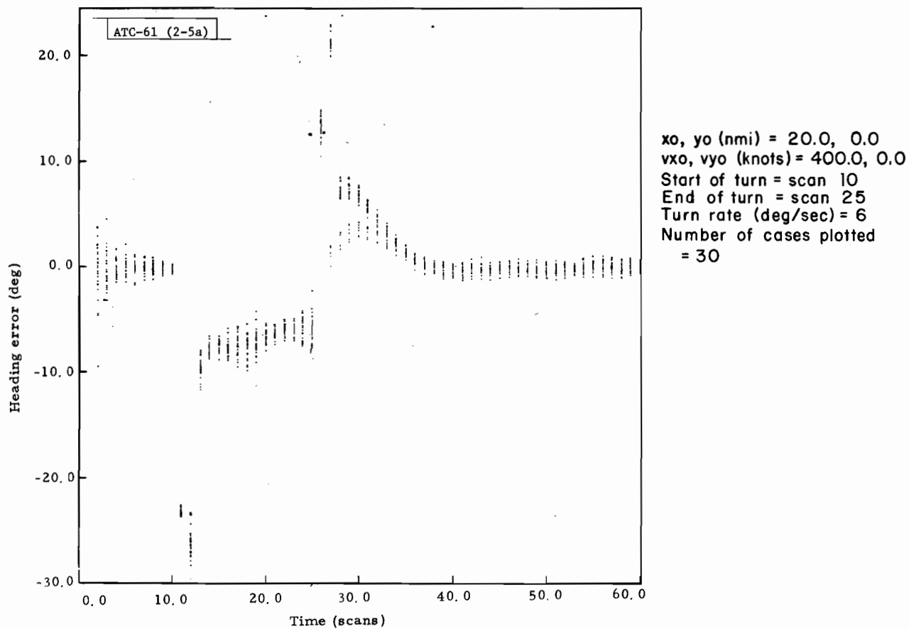
Fig. 2-5(a). Tracker dynamic heading performance in saturation mode (Region 1).
