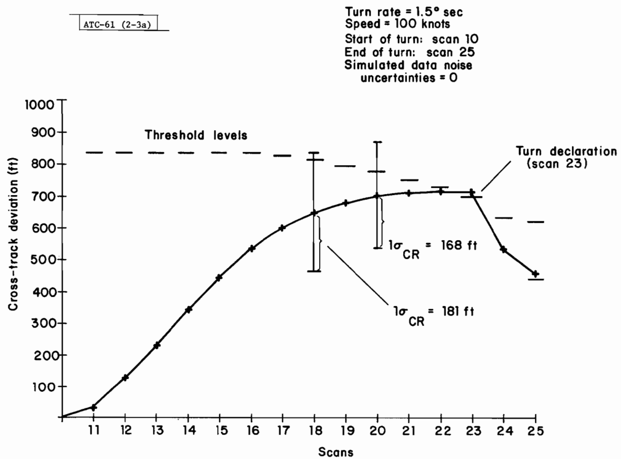
Fig. 2-3(a). Turn declaration; low turn rate ( 1.5^\circ/\text{sec} turn rate; ideal noise).
