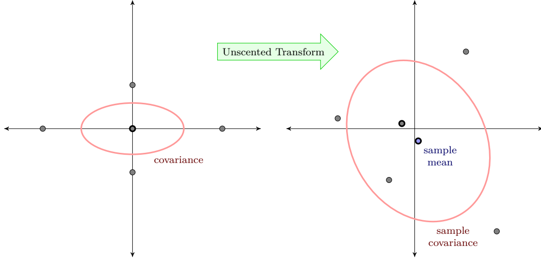
Figure B-2. The unscented transform. Sigma points are shown in gray. The central sigma point has a thicker outline.
