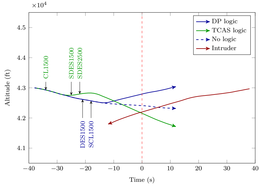
(a) Vertical profile.
