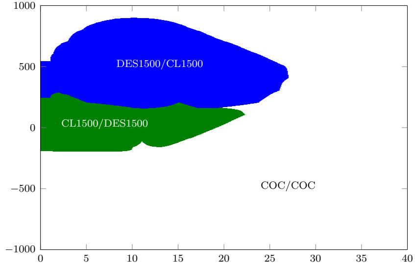
(b) \dot{h}_0 = 1500 ft/min, \dot{h}_1 = 0 ft/min, s_{RA} = \text{COC/COC}
