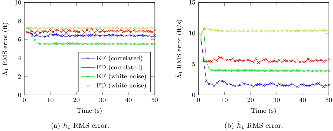
Figure B-4. Vertical tracking performance.
