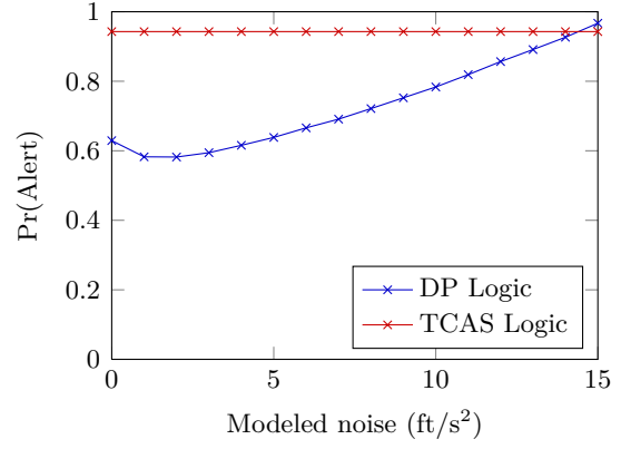
(b) Alert performance.
