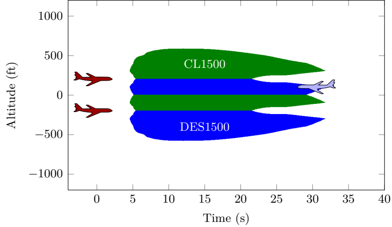
Figure 32. Closest command arbitration strategy. Two intruder aircraft are on the left, and the own aircraft is on the right. All aircraft are initially level and no advisory has been issued. The parameters from Section 3 with zero terminal cycles were used.
