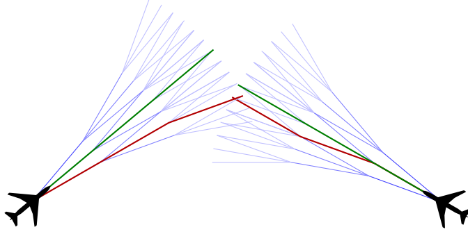
Figure 1. Trajectory propagation methods. Nominal trajectory propagation (green) only examines the most likely trajectory. Worst-case trajectory propagation (red) searches the space of possible trajectories for one that results in NMAC. Probabilistic trajectory propagation (blue) accounts for the relative likelihood of all trajectories.
