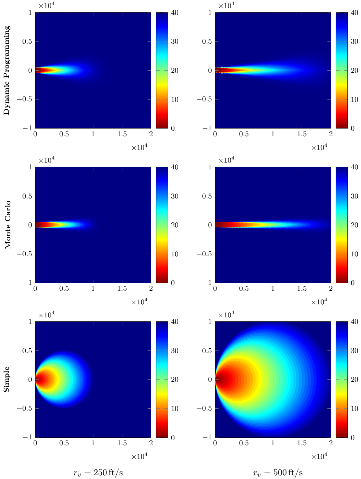
Figure 16. Mean of the entry distribution for two slices of the state space when the relative horizontal velocity is pointing directly left. Horizontal axis represents the relative x displacement (ft) and the vertical axis the relative y displacement (ft).
