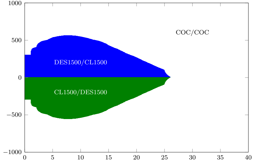
(a) \dot{h}_0 = 0 ft/min, \dot{h}_1 = 0 ft/min, s_{RA} = \text{COC/COC}
