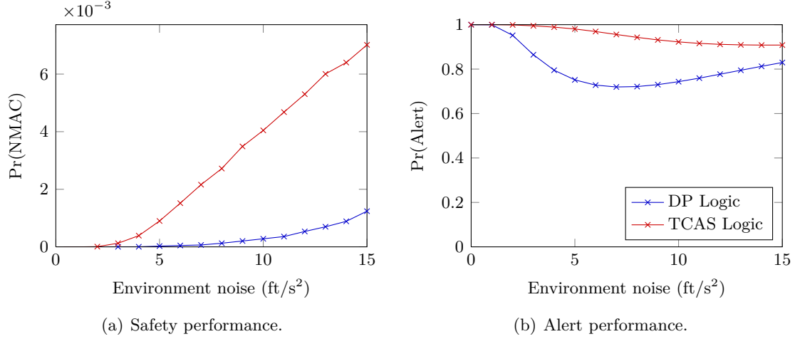
Figure 9. Parametric robustness with varying environment and constant logic optimized at \sigma_h = 8 \text{ ft/s}^2 .
