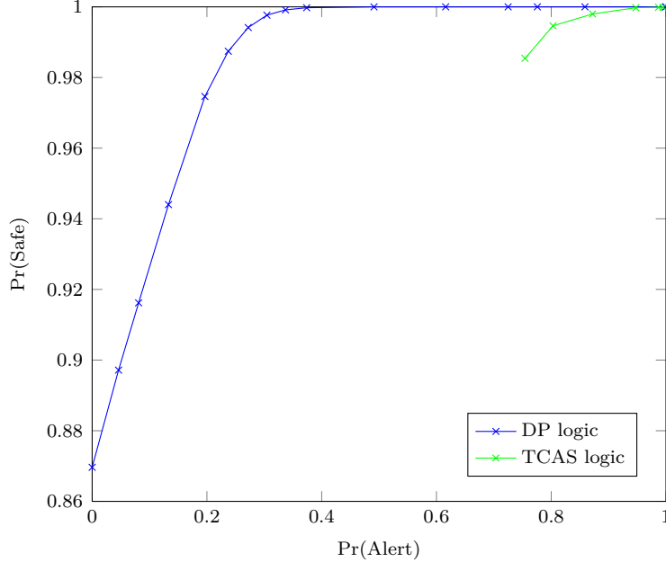
Figure 6. Safety curve. Each point on the curve was estimated from 100,000 simulations.
