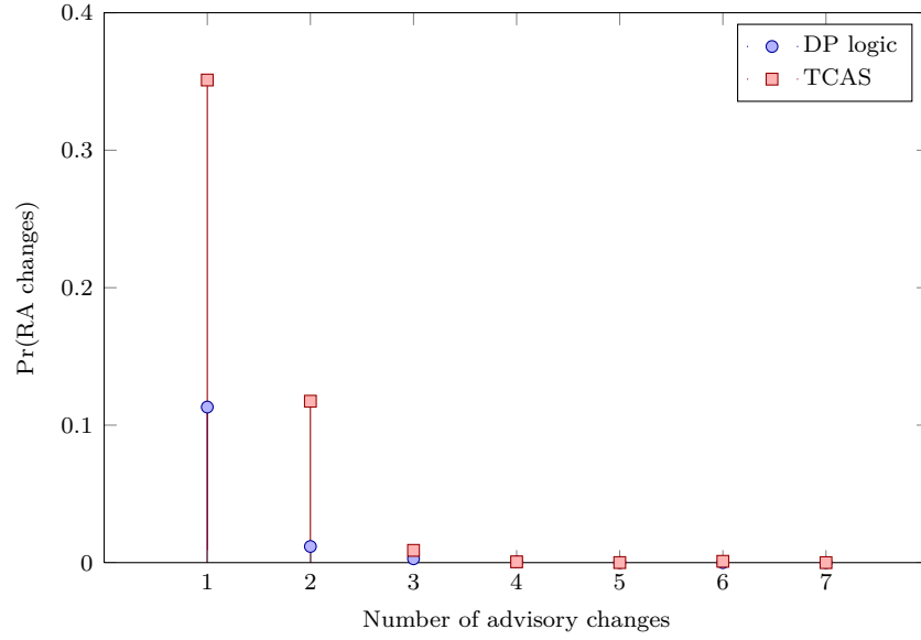
(a) Distribution of advisory changes. The probability of no changes is 0.8645 for DP and 0.5211 for TCAS.
