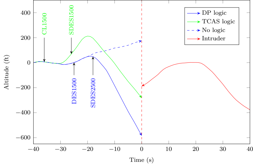
Figure 5. Example encounter comparing the performance of the DP logic against the current TCAS logic. The own aircraft approaches from the left, and the intruder approaches from the right.
