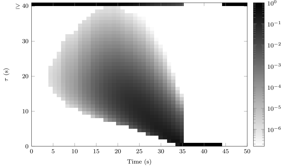
Figure 25. Entry time distribution over time for the example encounter.
