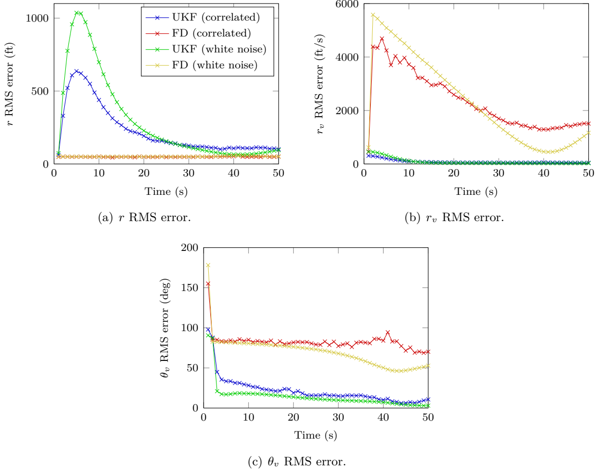
Figure B-3. Horizontal tracking performance.
