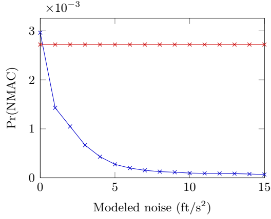
(a) Safety performance.
