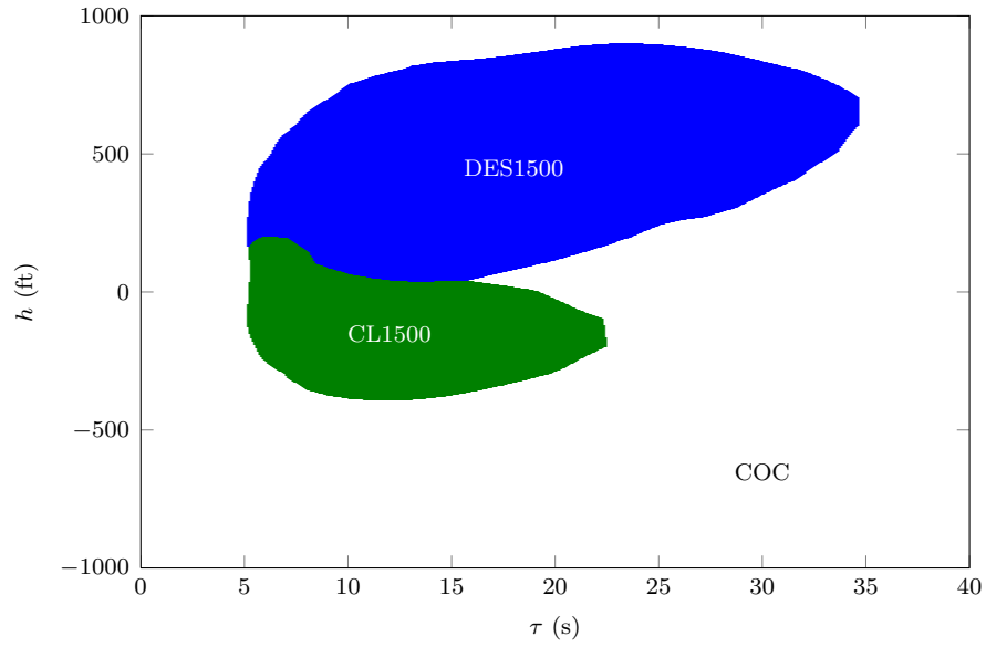
(b) \dot{h}_0 = 1000 ft/min, \dot{h}_1 = 0 ft/min, s_{\text{RA}} = \text{COC}
