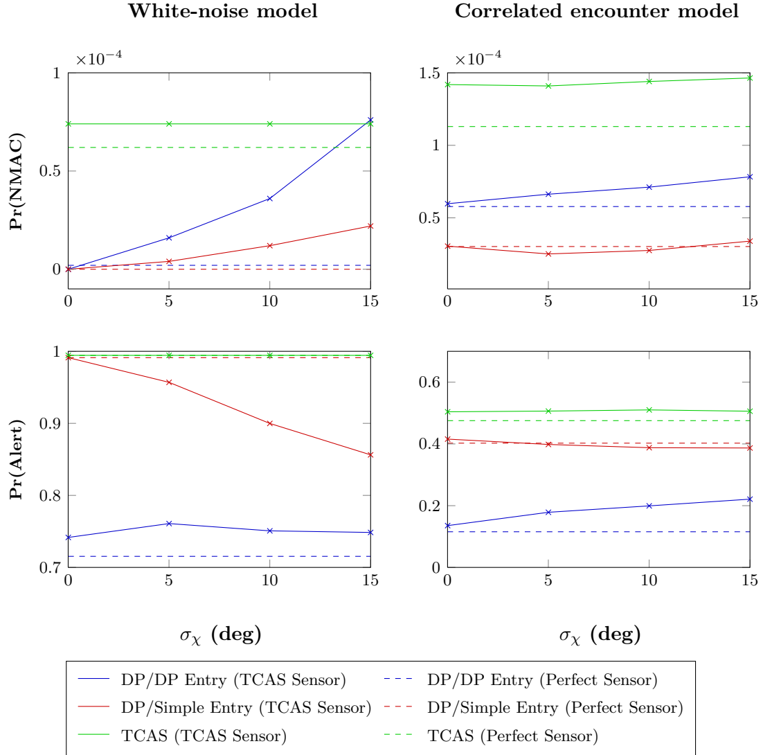
Figure 29. Sensor noise robustness. Each point on the curves was estimated from 500,000 simulations.
