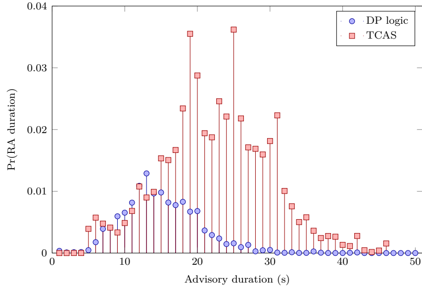
(b) Distribution of advisory duration. The probability of no duration is 0.8638 for DP and 0.5211 for TCAS.
