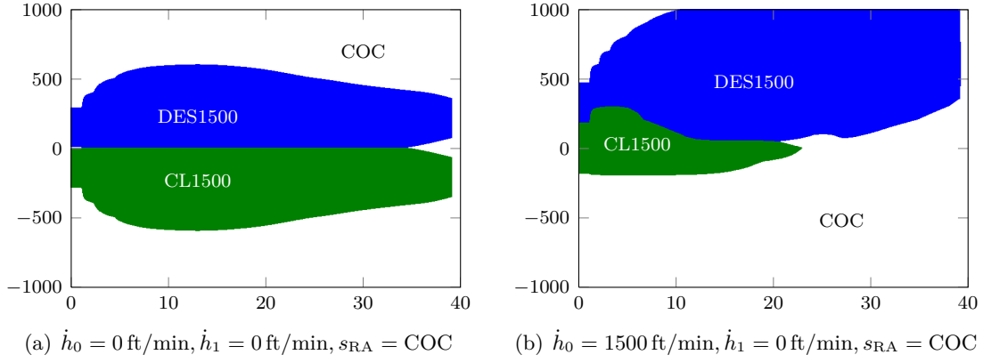
Figure 20. Optimal action plots for five terminal cycles. Horizontal axis indicates \tau (s) and the vertical axis indicates h (ft).
