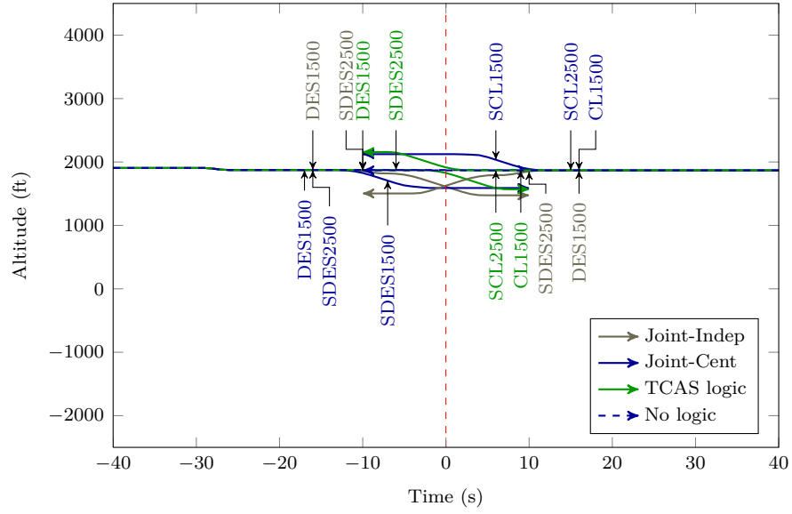
(a) Vertical profile.
