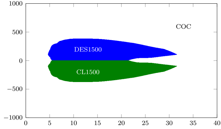
(a) \dot{h}_0 = 0 ft/min, \dot{h}_1 = 0 ft/min, s_{RA} = \text{COC}
