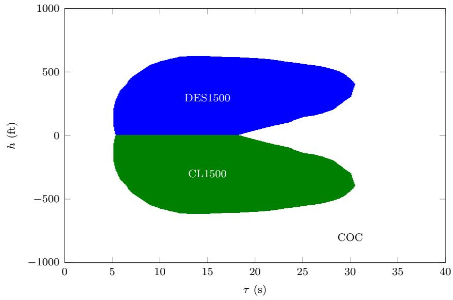
(a) \dot{h}_0 = 0 ft/min, \dot{h}_1 = 0 ft/min, s_{\text{RA}} = \text{COC}
