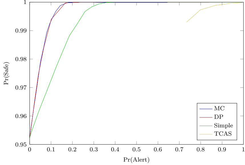
Figure 19. Safety curves. Each point on the curves was estimated from 10,000 simulations.
