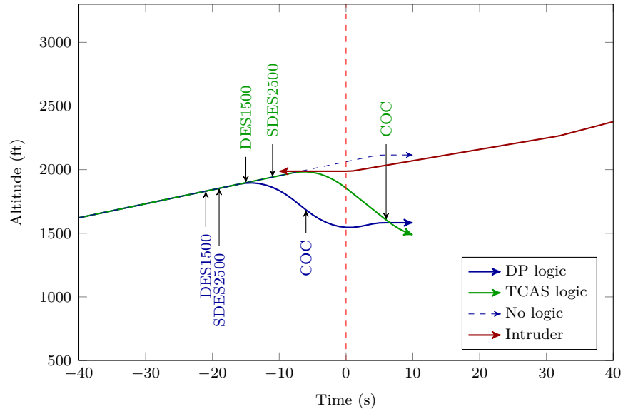
(a) Vertical profile.
