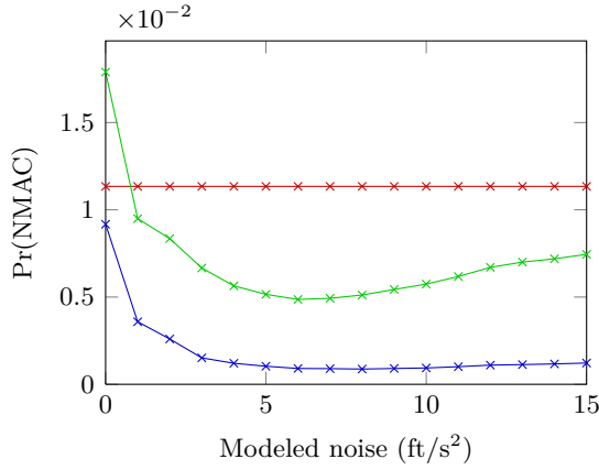
(a) Safety performance.
