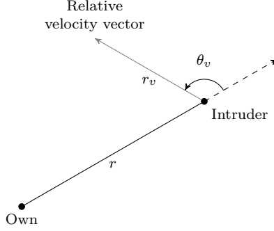
Figure 15. Three-variable model of horizontal dynamics.
