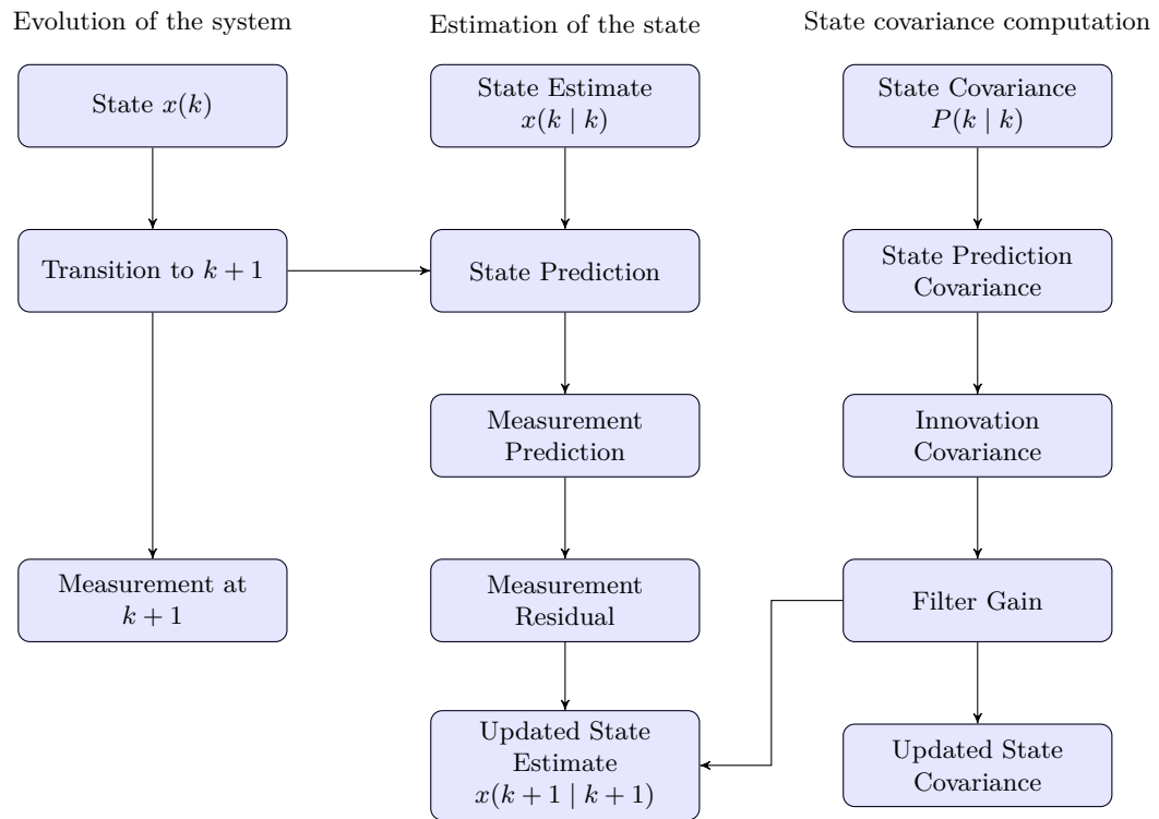
Figure B-1. Recursive estimation process using the Kalman filter.
