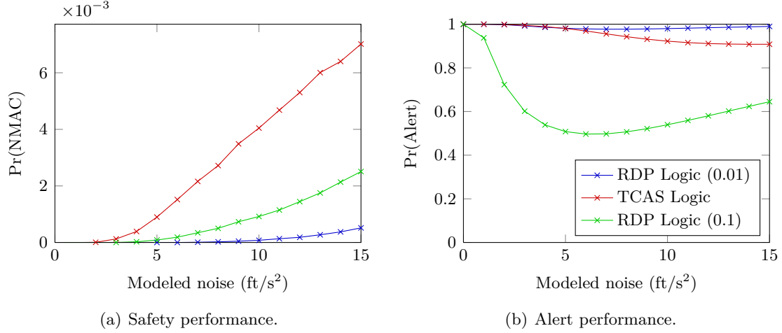
Figure 12. Robust logic performance on white-noise encounter model. DP alert cost is in parentheses.
