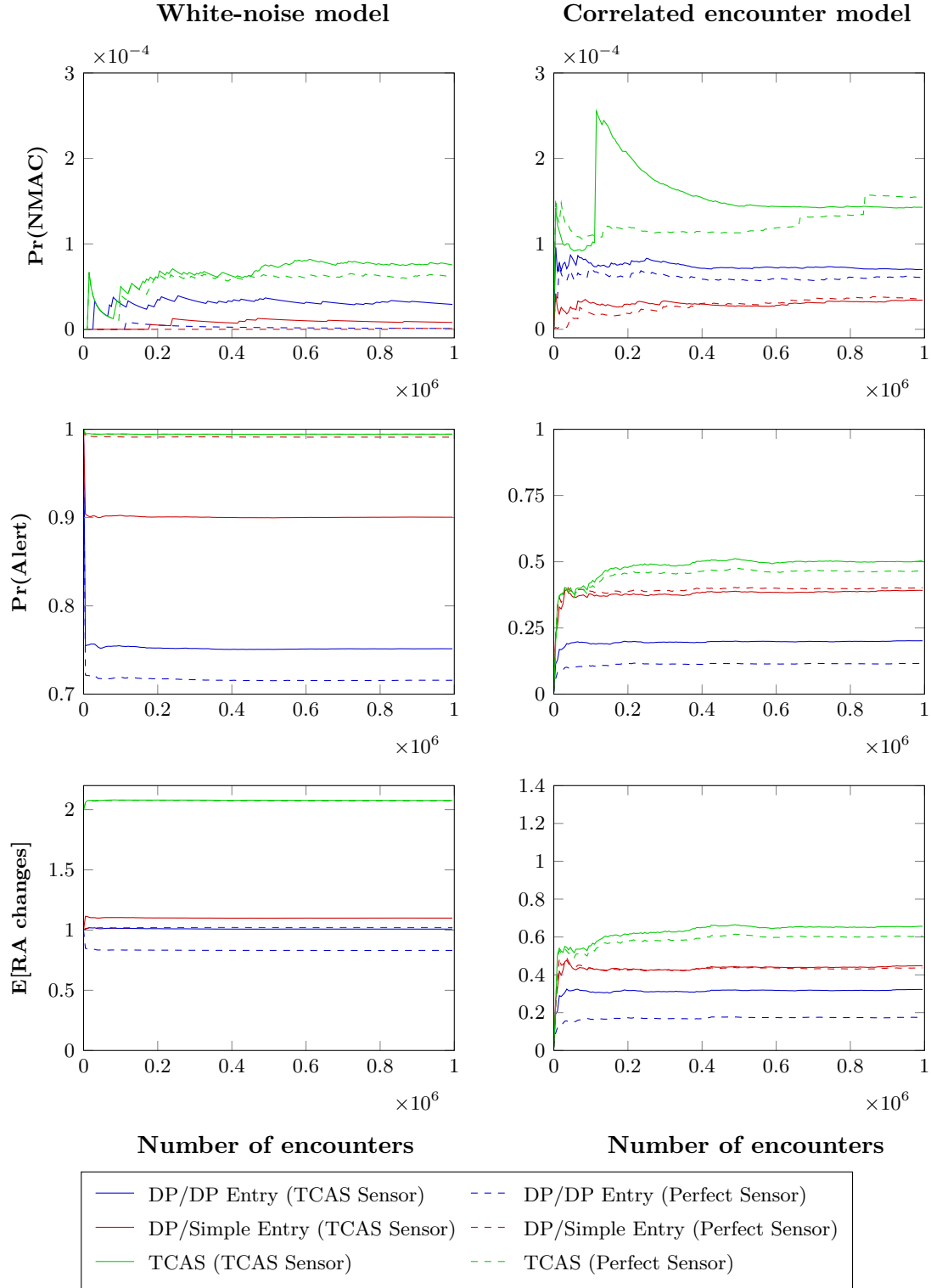
Figure 28. Convergence curves for DP and TCAS with and without sensor noise.
