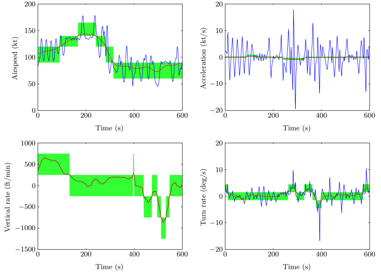
Figure 9. A plot of extracted features over time. Blue lines show features before smoothing, and red lines show features after smoothing. The green blocks show the bins to which the features are assigned.
