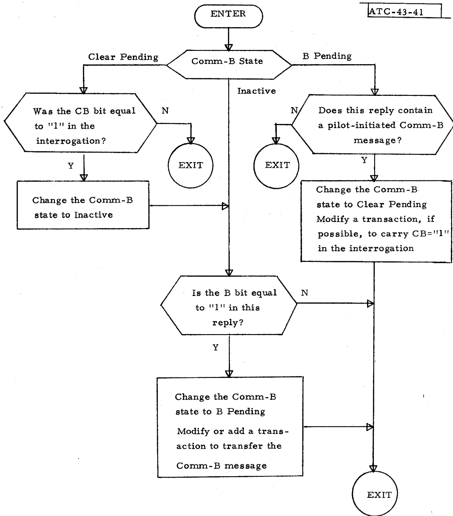
Figure 41. Comm-B Procedure
