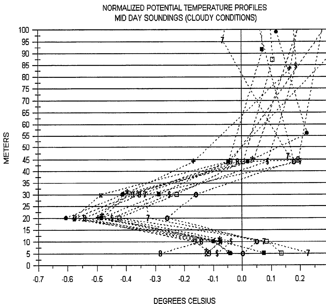
Figure 3. Normalized potential temperature profiles calculated for several days with neutral stability.
