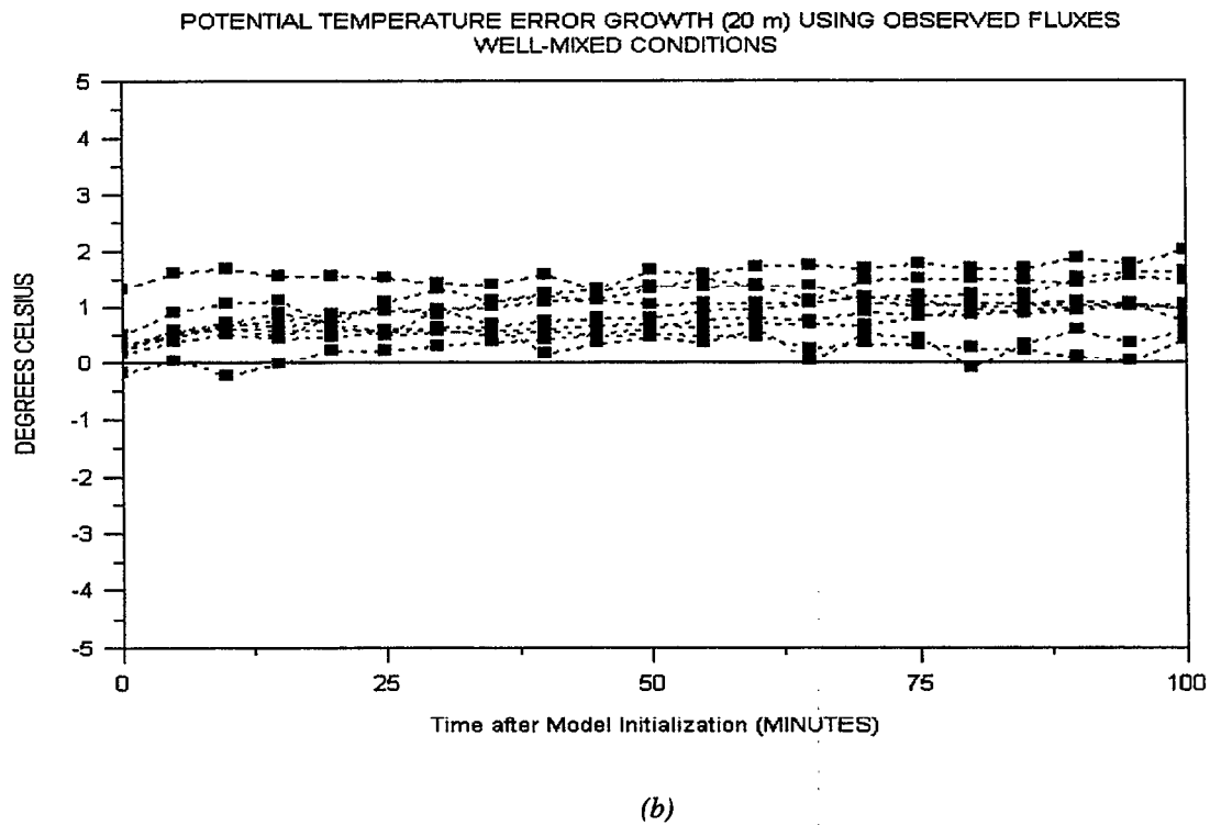
Figure 11. Modeled potential temperature error growth rate as compared with 20 m sensor during first 100 minutes using SVAT (a) and observed fluxes (b) for eight apparently well mixed cases.
