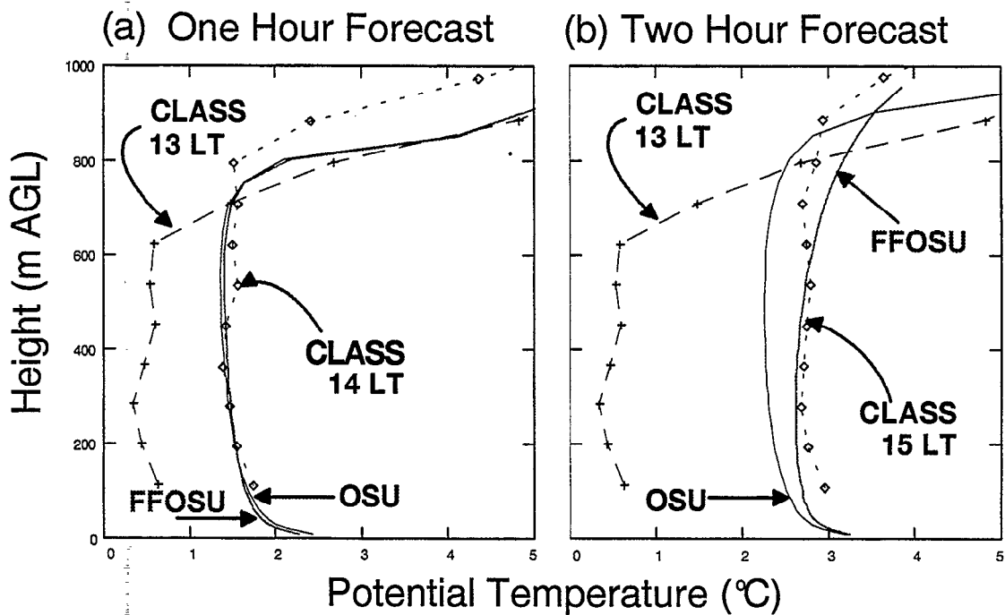
Figure 12. CLASS potential temperature profiles observed at 13, 14 and 15 LT 12 March 1992 versus one hour (a) and two hour (b) OSU and FFOSU forecasts valid at 14 and 15 LT.
