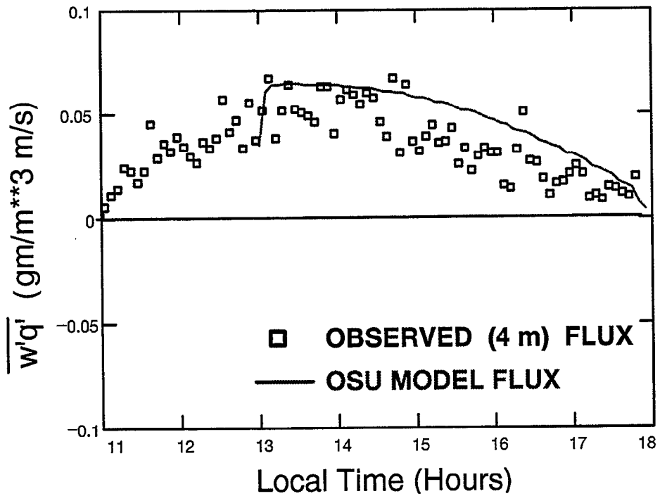
Figure 9. Observed 4 m versus modeled surface layer water vapor mixing ratio flux for 12 March 1992 at the STORM-FEST ASTER tower site.
