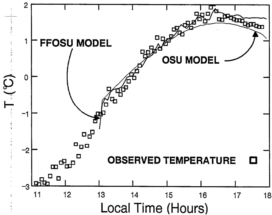
Figure 6. Observed versus original (OSU) and flux-forced (FFOSU) 10 m temperature for 12 March 1992 at the STORM-FEST ASTER tower site.
