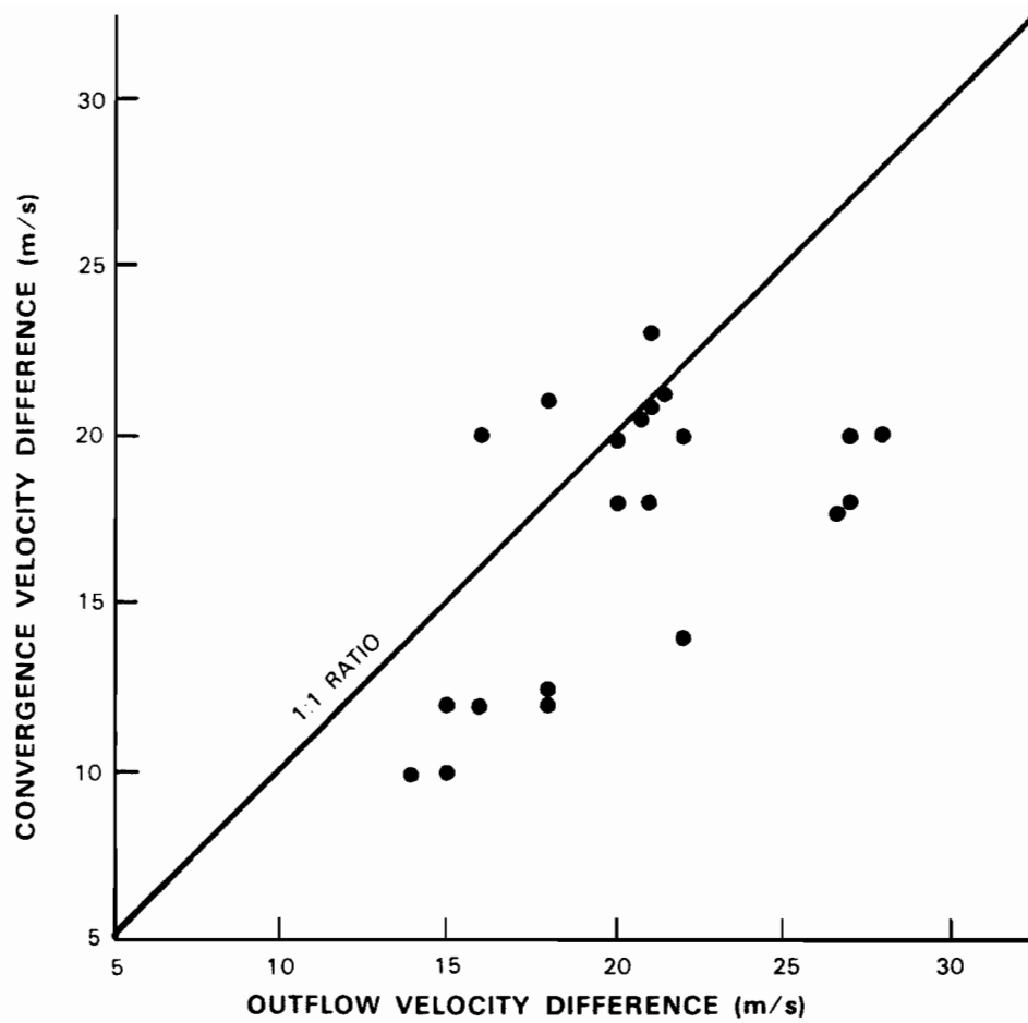
Fig. 2. Scattergram of convergence and surface outflow (m/s).
