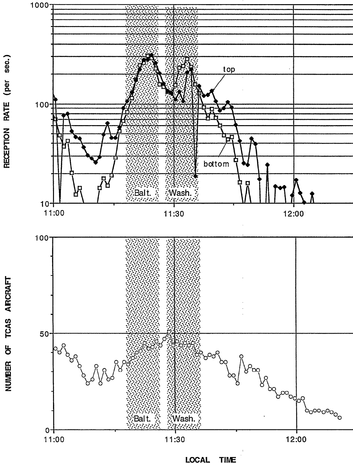
Figure 13. Total TCAS interrogations and suppressions received by the AMF, Washington.
