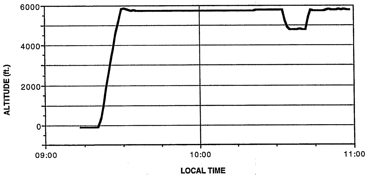
Figure 3. Flight path.
