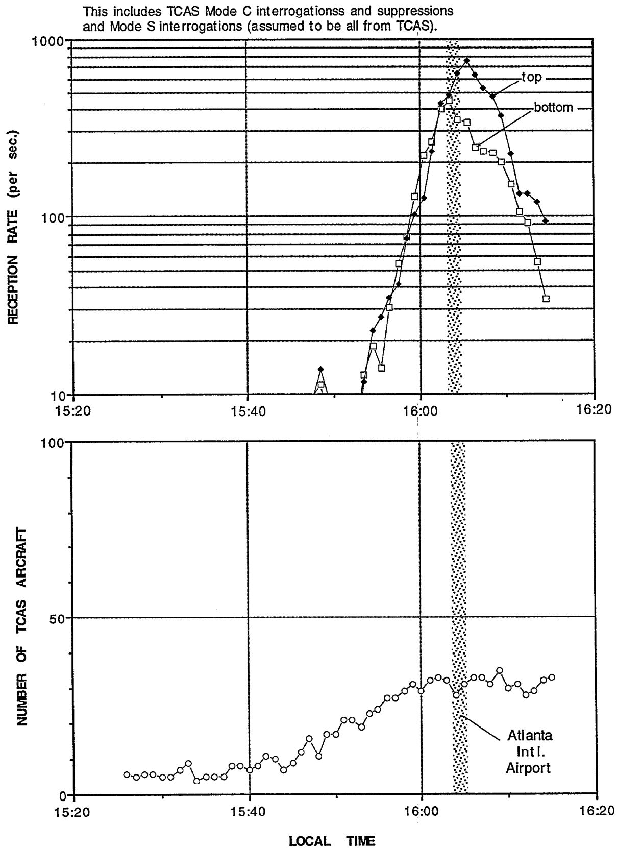
Figure 17. Total TCAS interrogations and suppressions received by the AMF (Atlanta).
