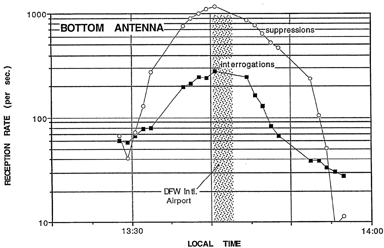
Figure 19. Total interrogations and suppressions received by the AMF (Dallas).
