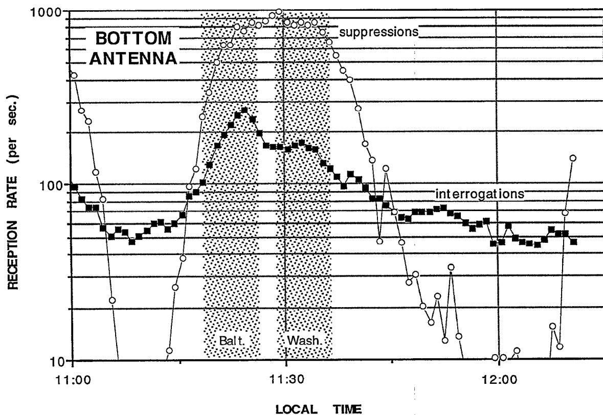
Figure 11. Total interrogations and suppressions received by the AMF (Washington).
