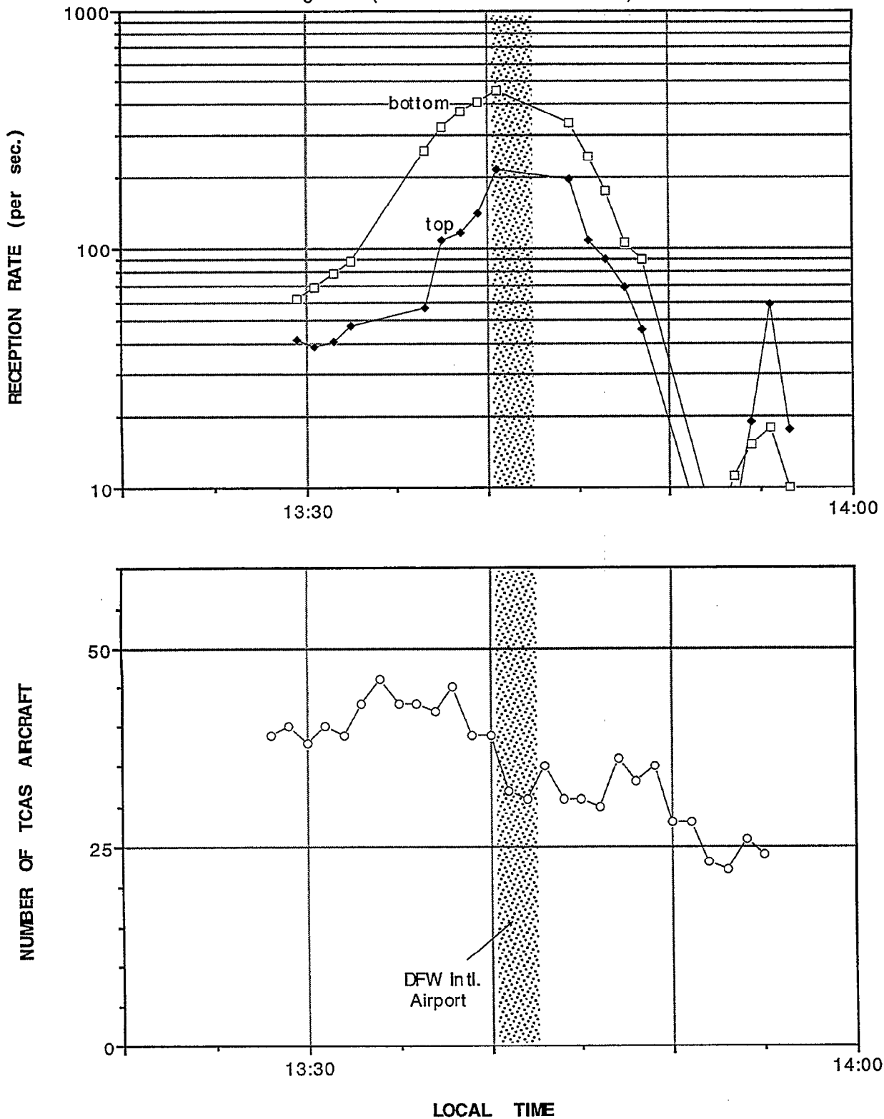
Figure 21. Total TCAS interrogations and suppressions received by the AMF (Dallas).
