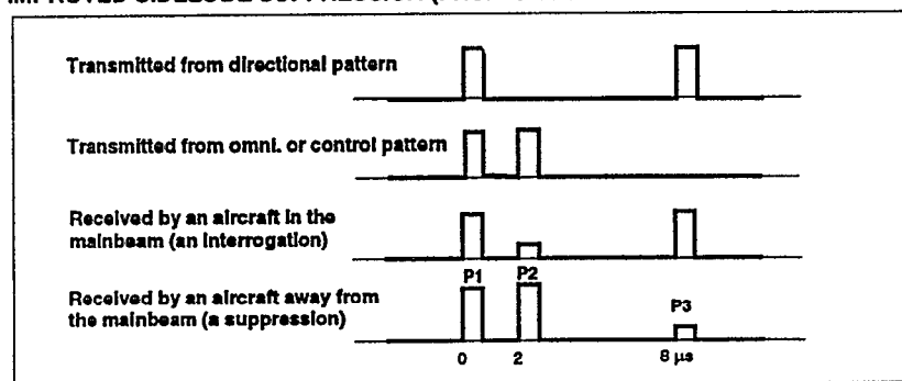
Figure 2. Transmissions in the 1030 MHz band.
