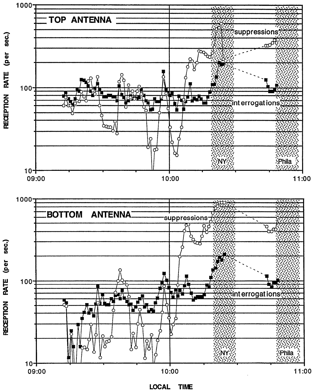
Figure 4. Total interrogations and suppressions received by the AMF.
