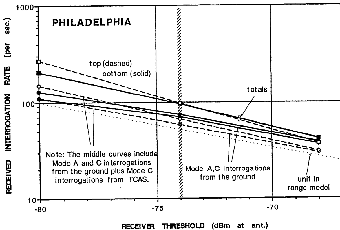
Figure 8. Power distributions.
