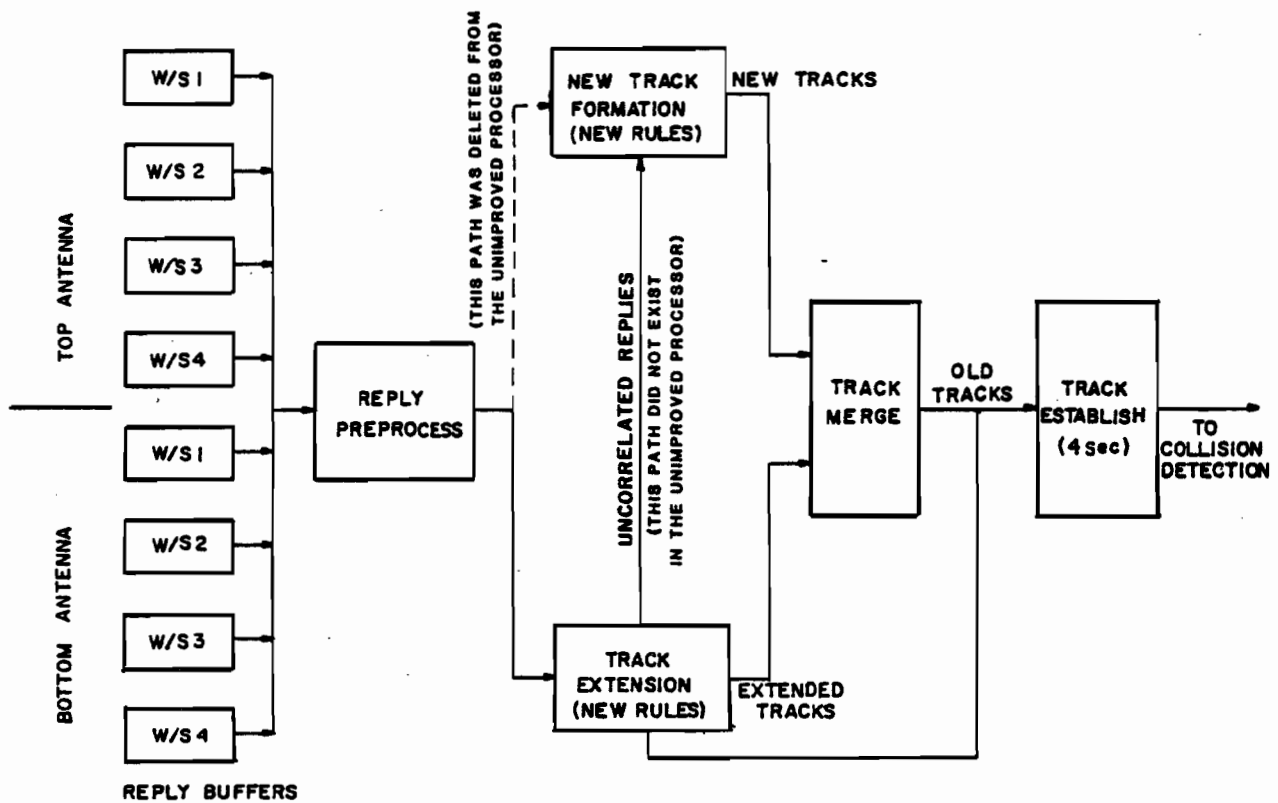
Fig. 3-35. Improved ATCRBS surveillance processing.
