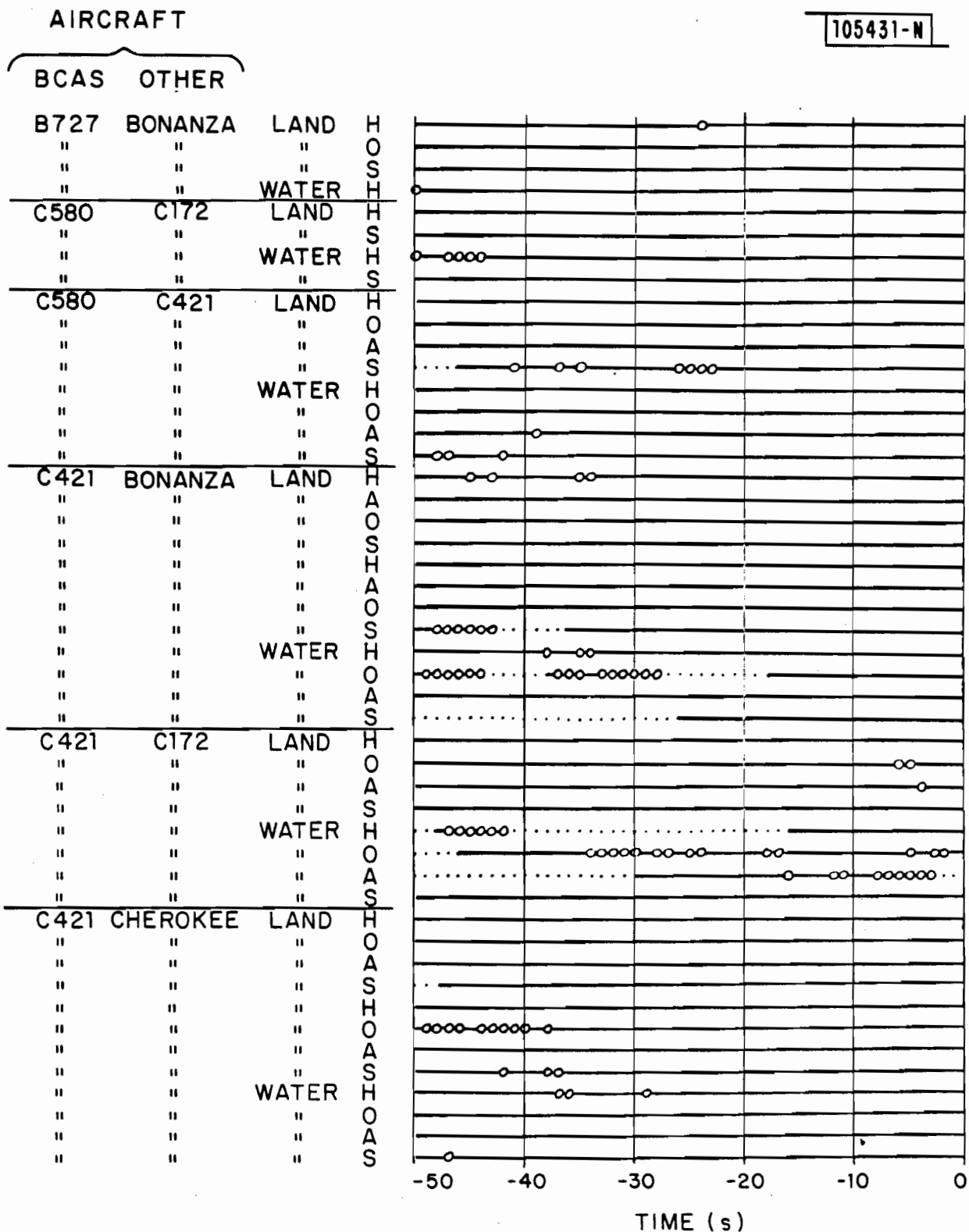
Fig. 3-23. Results of 48 encounters - DABS transponder without diversity.
