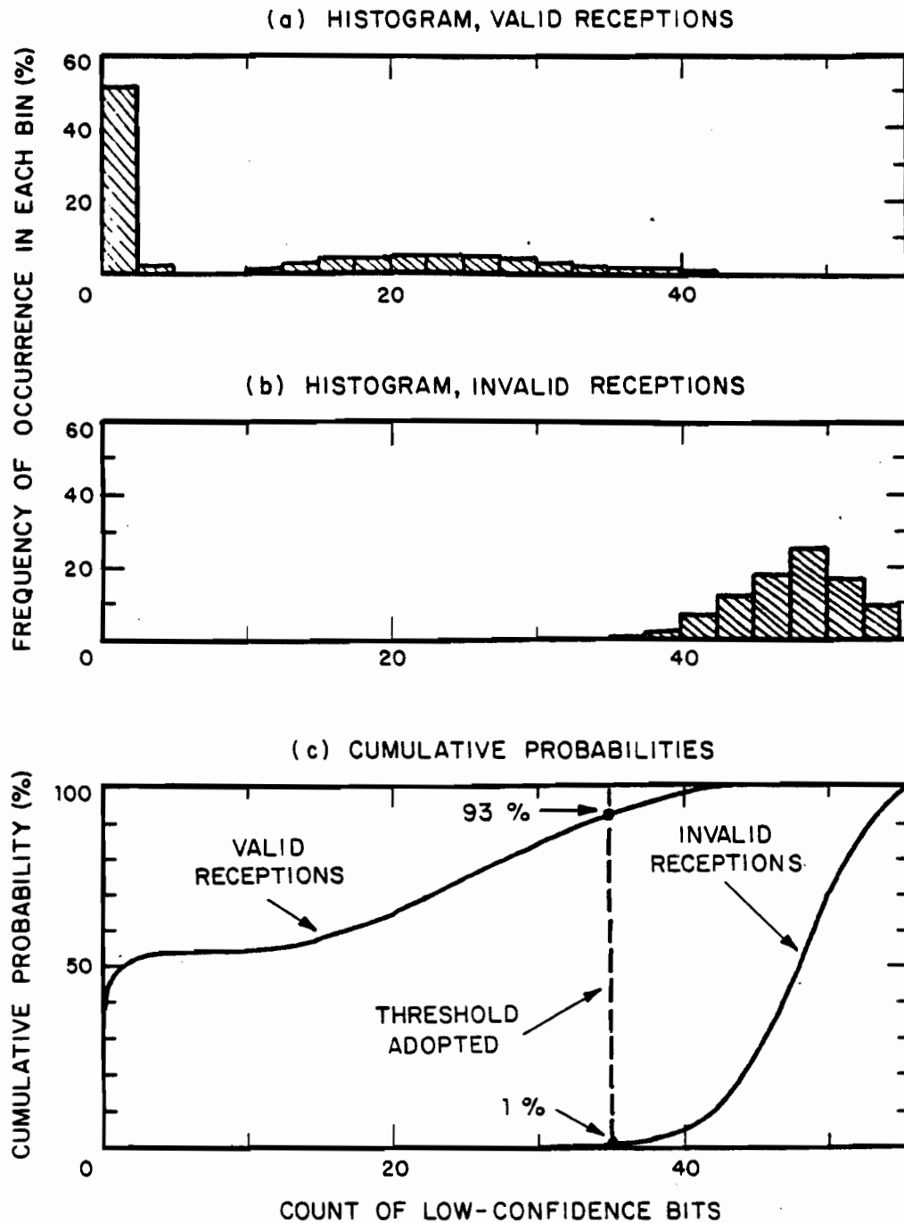
Fig. 3-13. Squitter measurement results.
