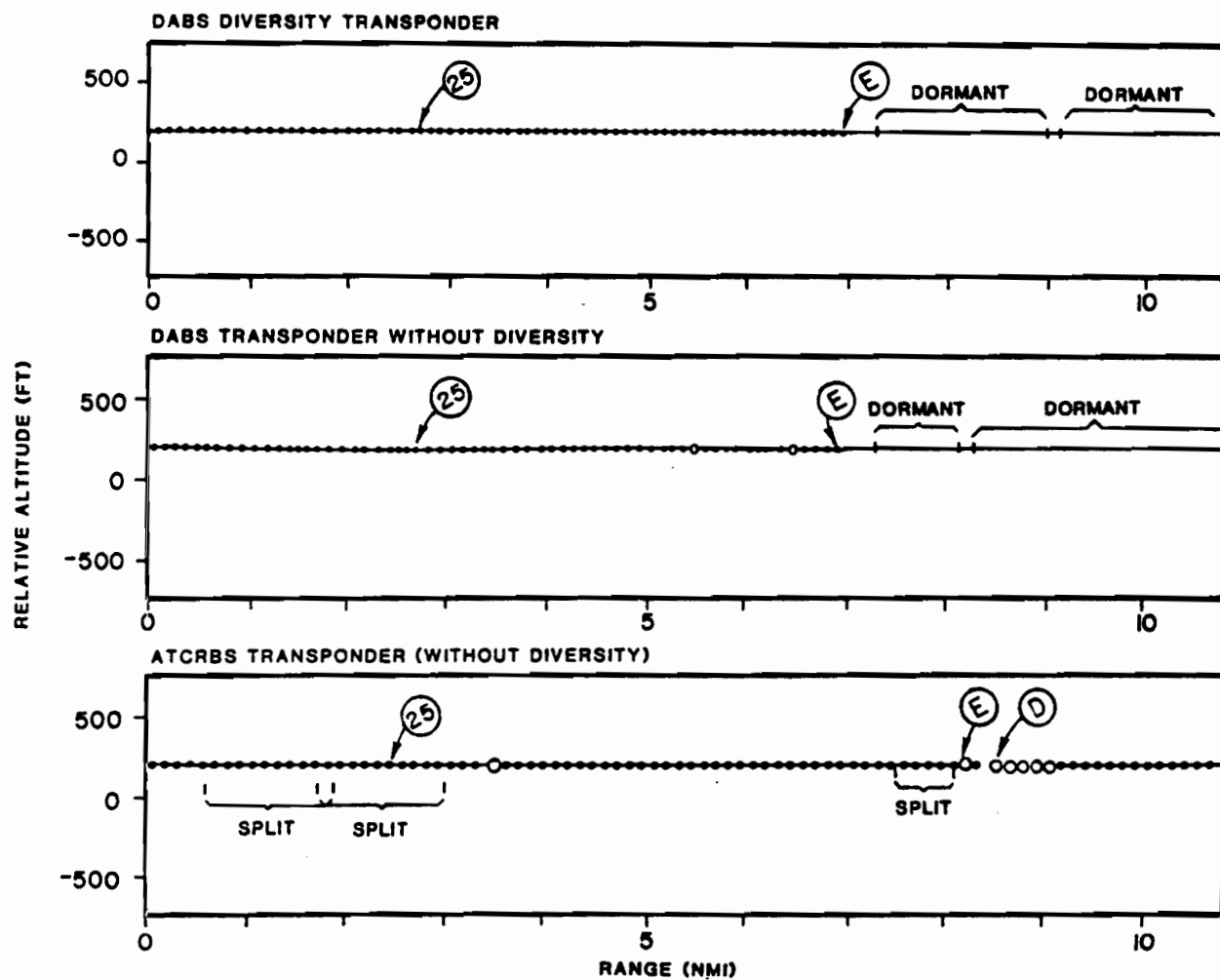
Fig. 3-21. BCAS performance: head-on encounters over ocean.
