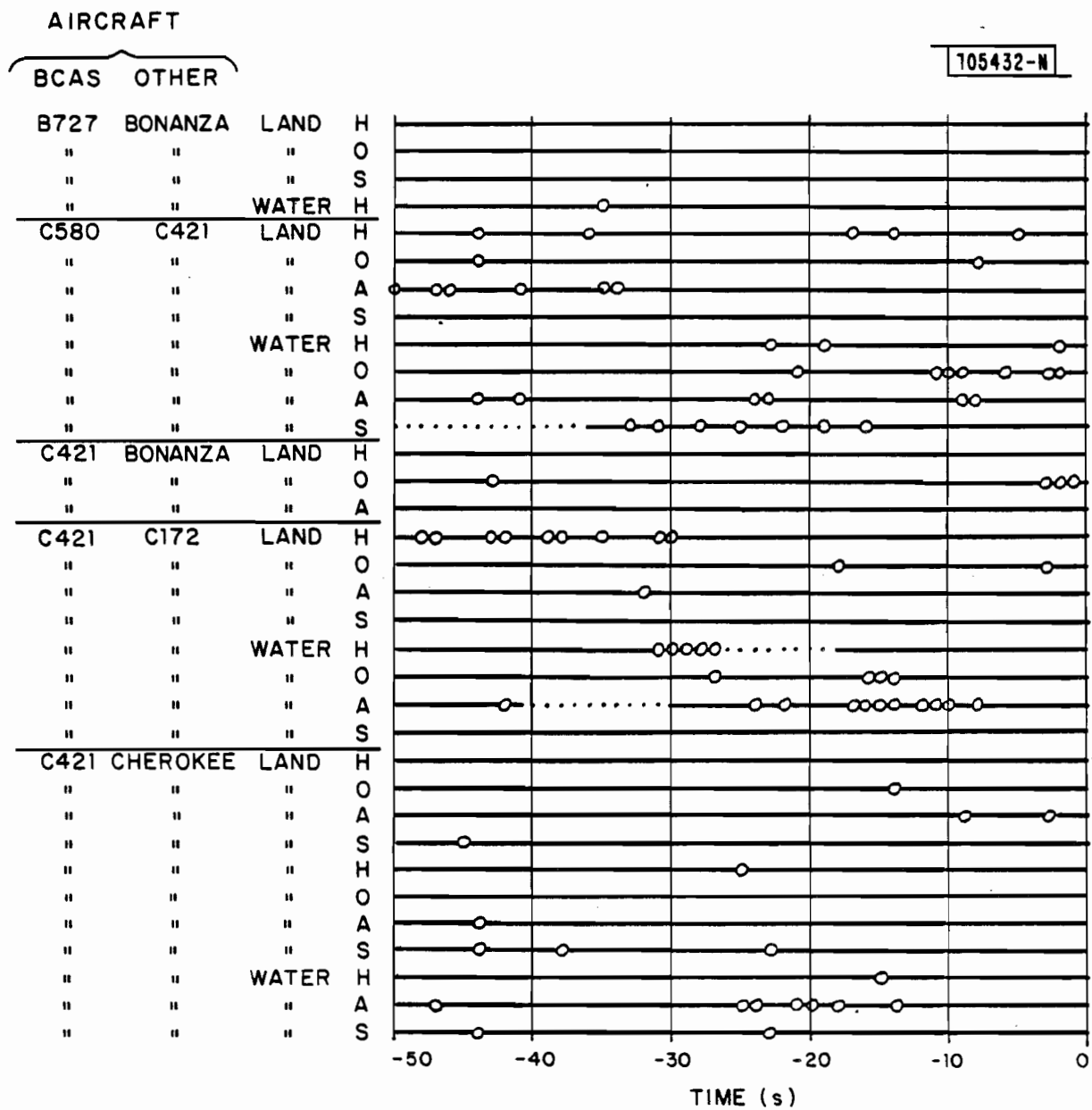
Fig. 3-24. Results of 34 encounters - ATCRBS transponder (without diversity).
