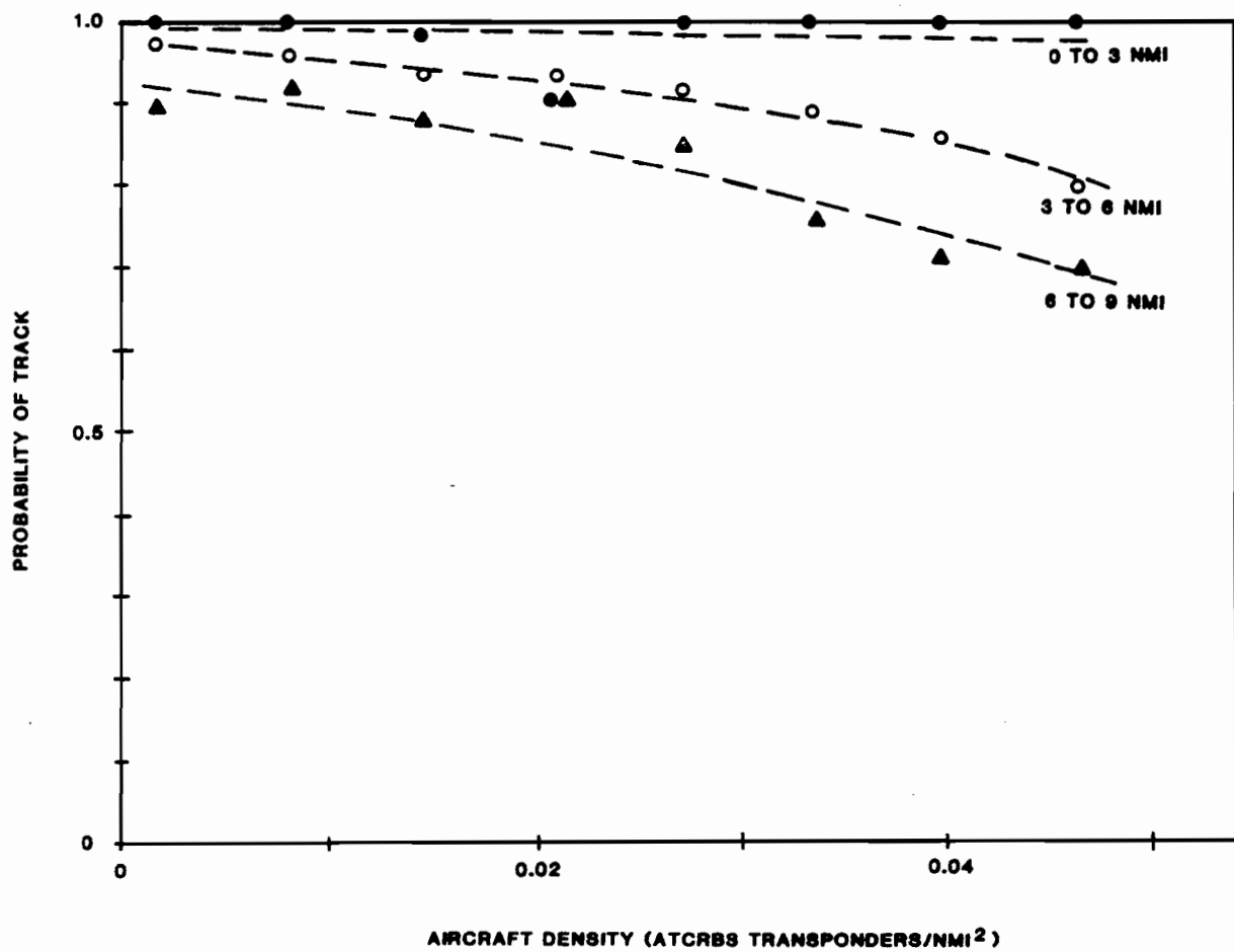
Fig. 4-4. Tracking performance vs density and range.
