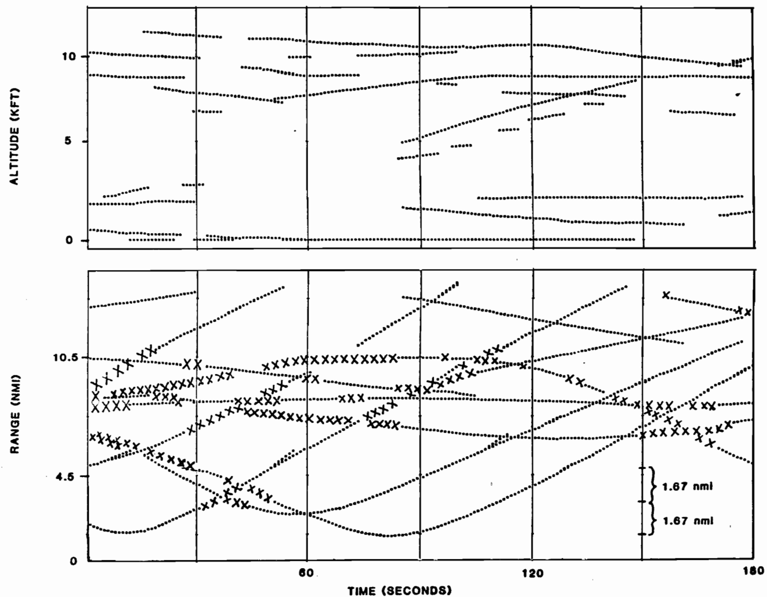
Fig. 3-40. Tracking performance - without whisper/shout.
