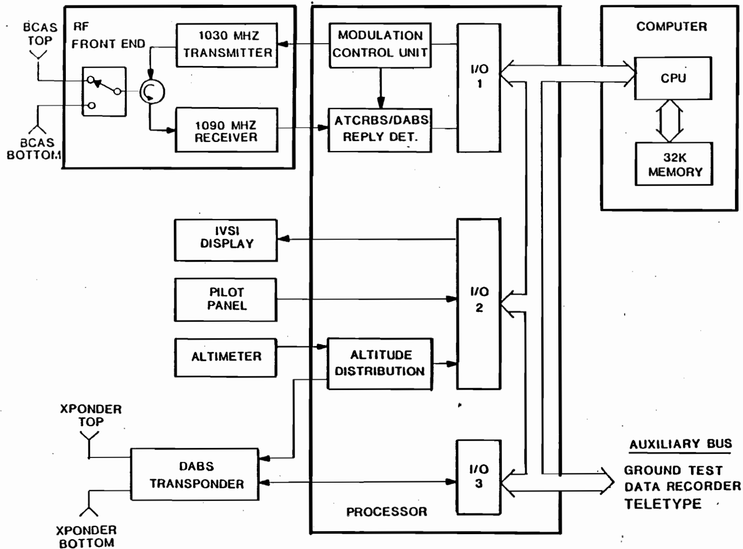
Fig. 2-5. BCAS Experimental Unit block diagram.
