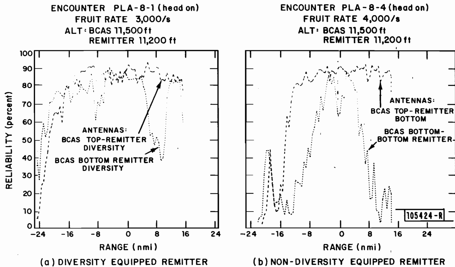
Fig. 3-7. Link round reliability for head-on encounters over Los Angeles.
