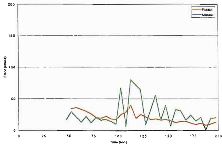
Figure 148. Outlier Test (Outlier at Time 100) - Ground Speed Error - CD2 Data - COTS A.
