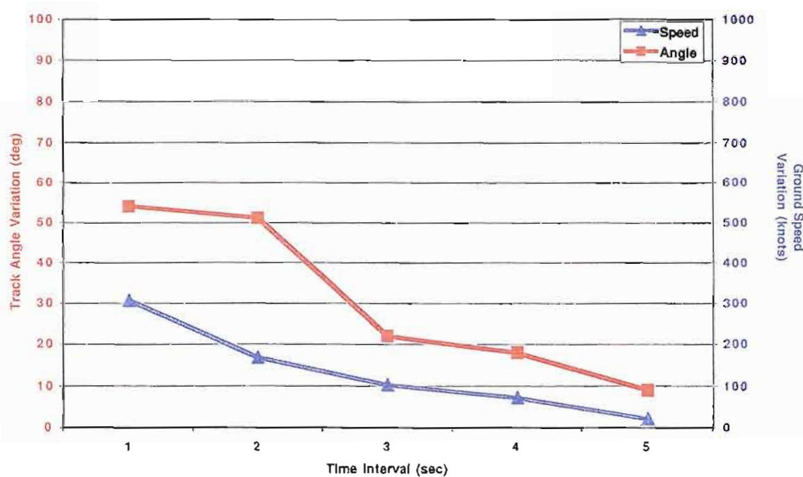
Figure 8. Effect of Inter-Report Interval on 2-pt Velocity Variation - Mode S Data.
