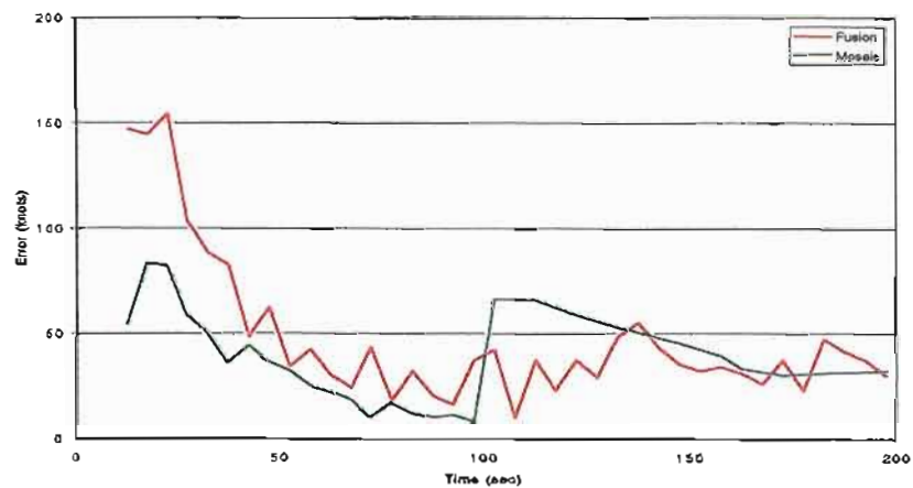
Figure 106. Sensor Hop Due to Biases Test - Sensor Change at 100 Seconds - Ground Speed Error - CD2 Data - COTS B.
