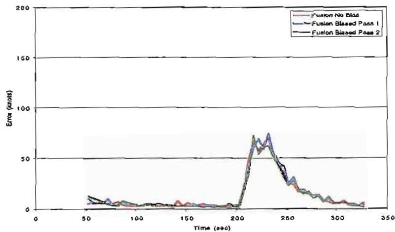
Figure 97. Bias Adaptation Test (1 Hour Adaptation Period) - Turn 200-230 Seconds - Ground Speed Error - Mode S Data - COTS D.
