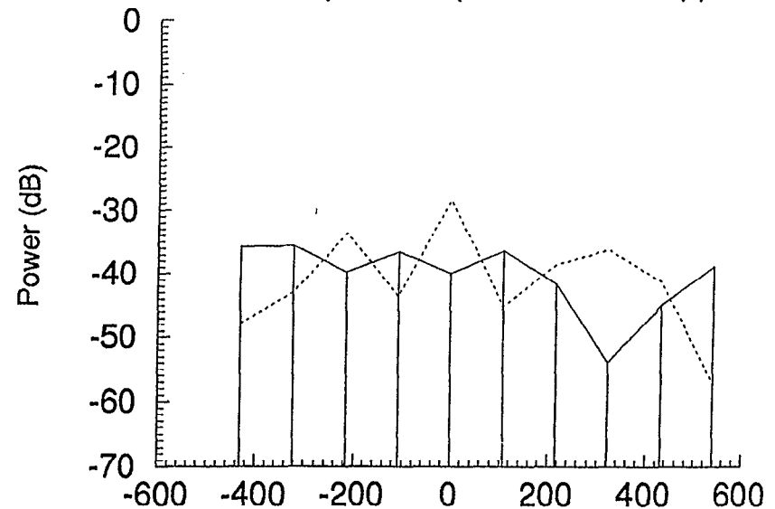
Figure 22d. Doppler Shift in Hertz (10 pulses).
