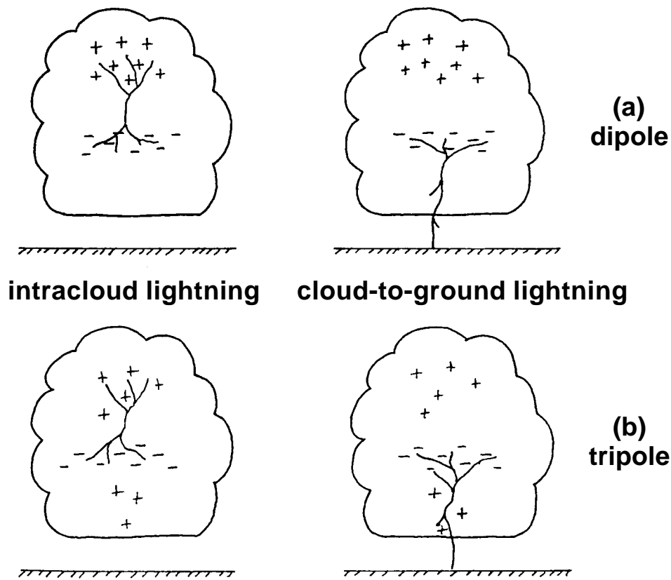
Figure C-5. Depiction of intracloud and cloud-to-ground lightning in prototype electrostatic structures: (a) dipole and (b) tripole (from Williams, et al., 1998).
