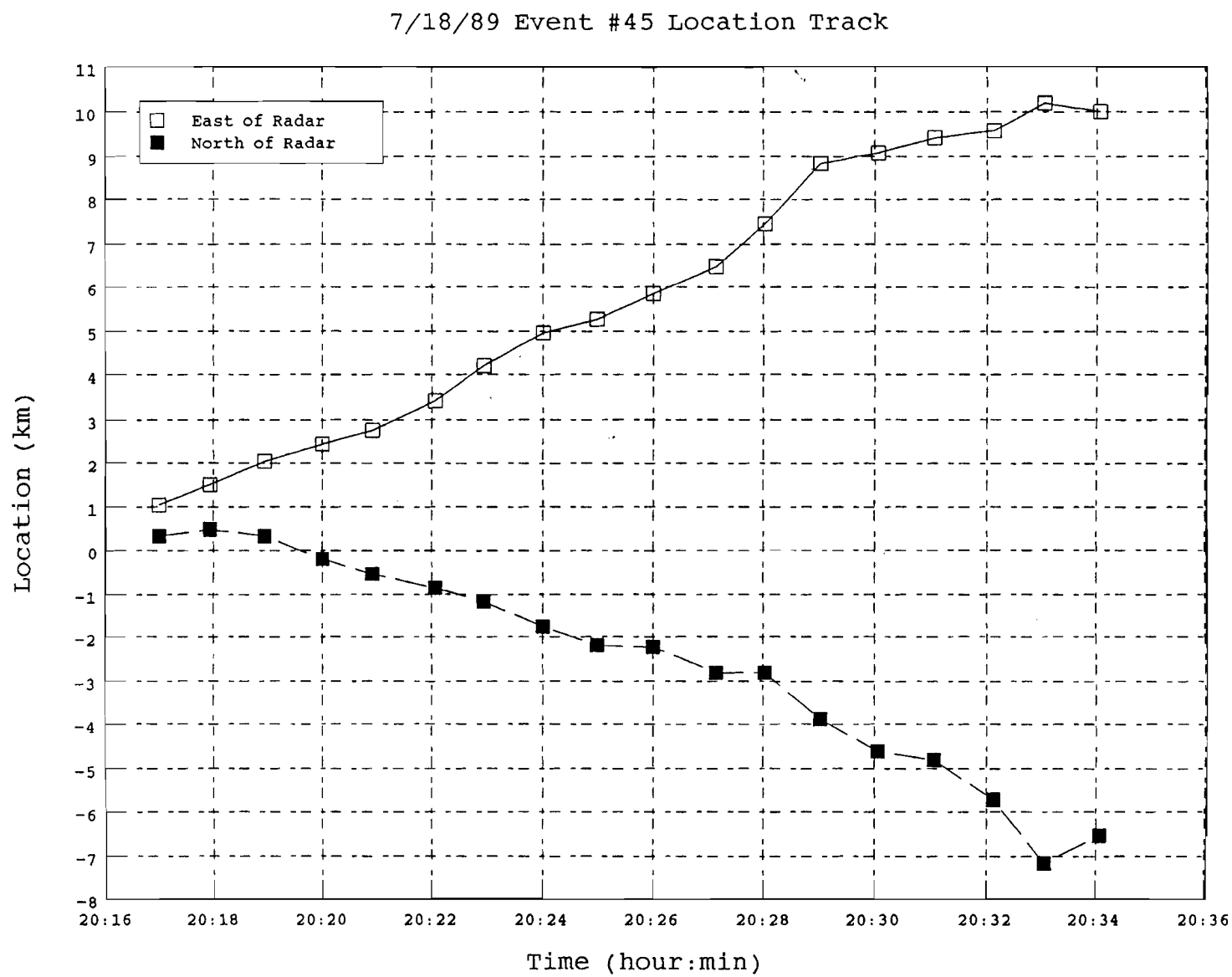
Figure 6. Motion of a strong Kansas City microburst as taken from the ITWS shear regions algorithm.
