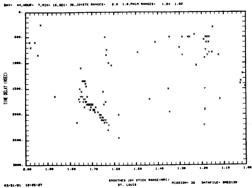
Fig.5-14(a). Data summary for St. Louis's approach with 50 ft. threshold height.
