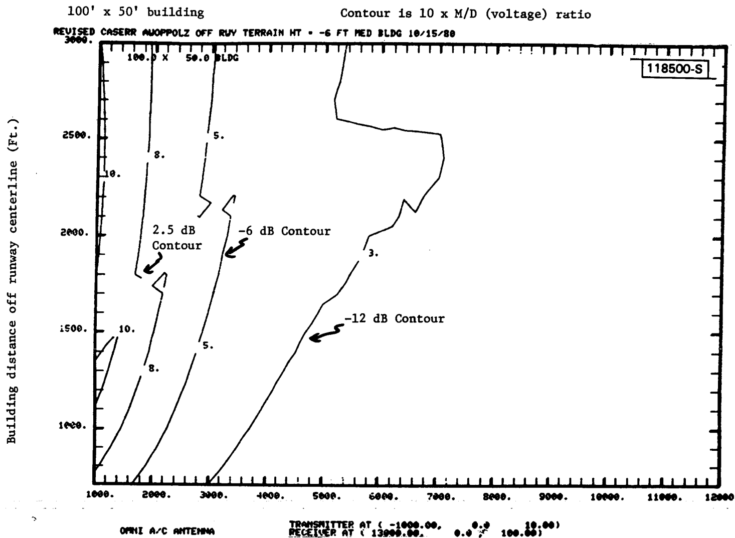
Fig.4-23. Effective M/D ratio from medium size building with receiver at Cat II decision height and off runway terrain 6.0 feet below runway level.
