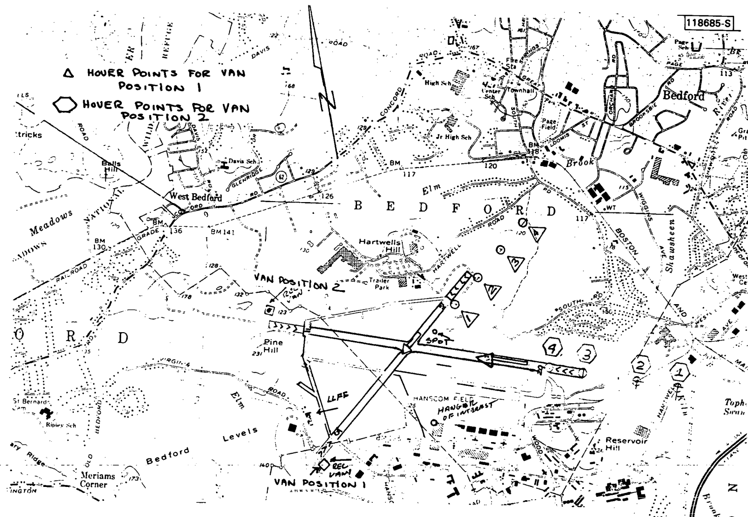
Fig.5-33. High time resolution multipath experiment geometry at L.G. Hanscom Airport (Bedford, MA).
