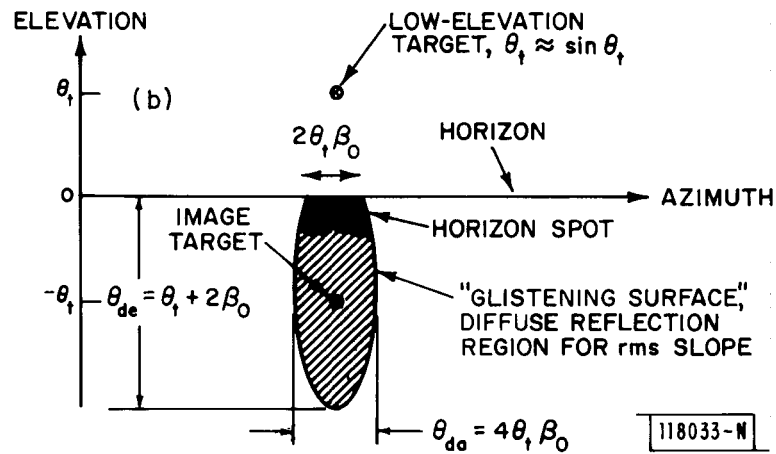
Fig.3-5. Diffuse multipath level and spatial distribution: (a) specular and diffuse scattering coefficient vs. roughness factor and (b) angular extent of glistering surface for rough surface scattering.
