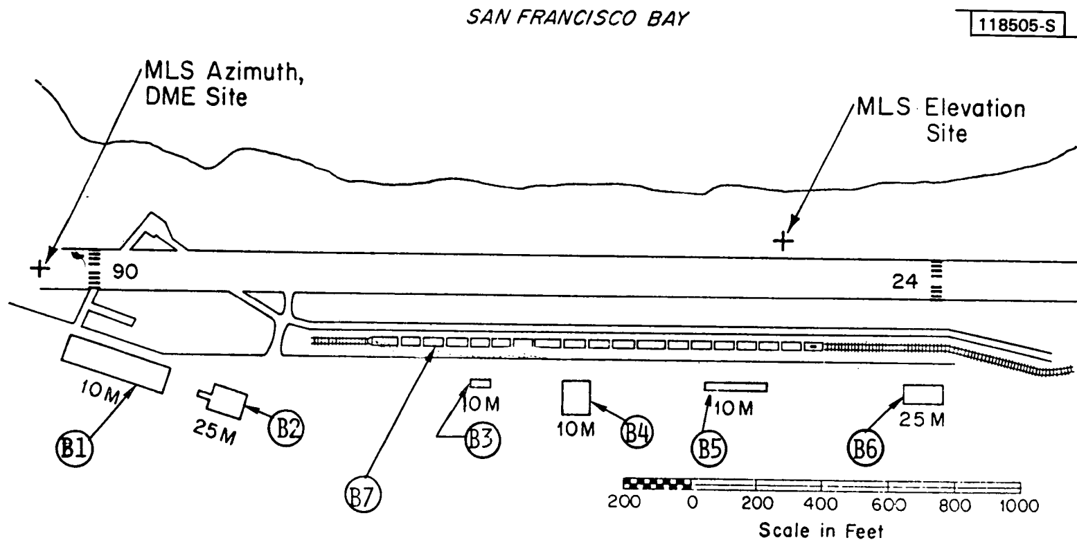
Fig.4-27. AWOP scenario 3 based on Crissey Army Airfield in San Francisco.
