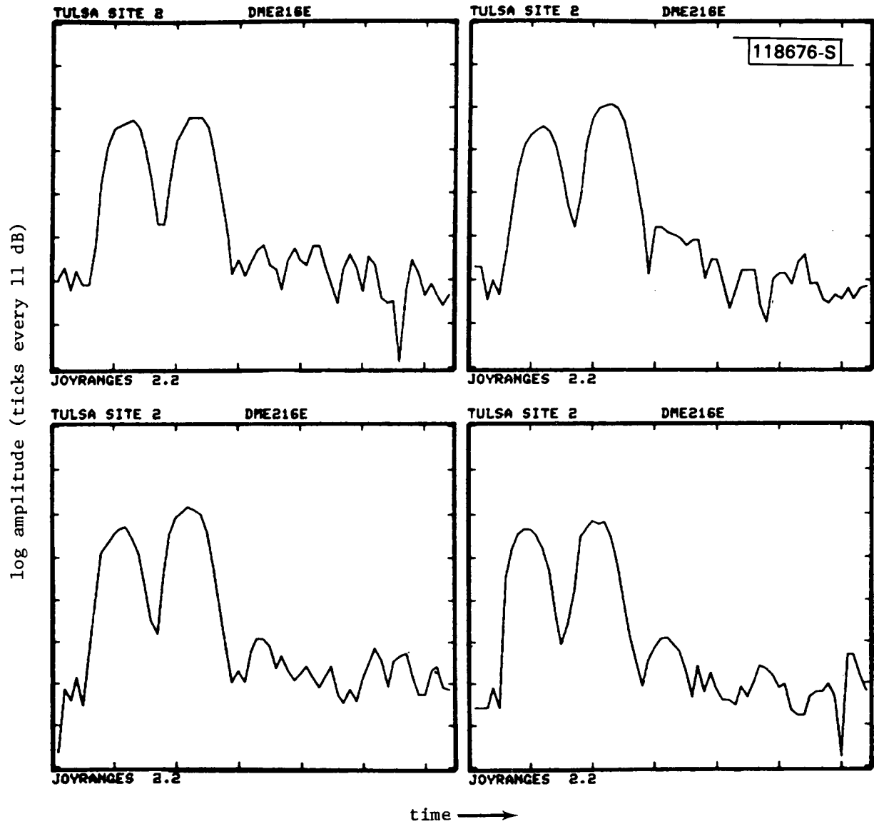
Fig.5-25. Tulsa site 2 waveforms near threshold.
