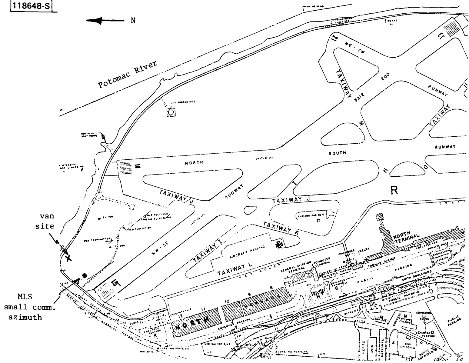
Fig.5-4. Washington National Airport DME multipath measurement site.
