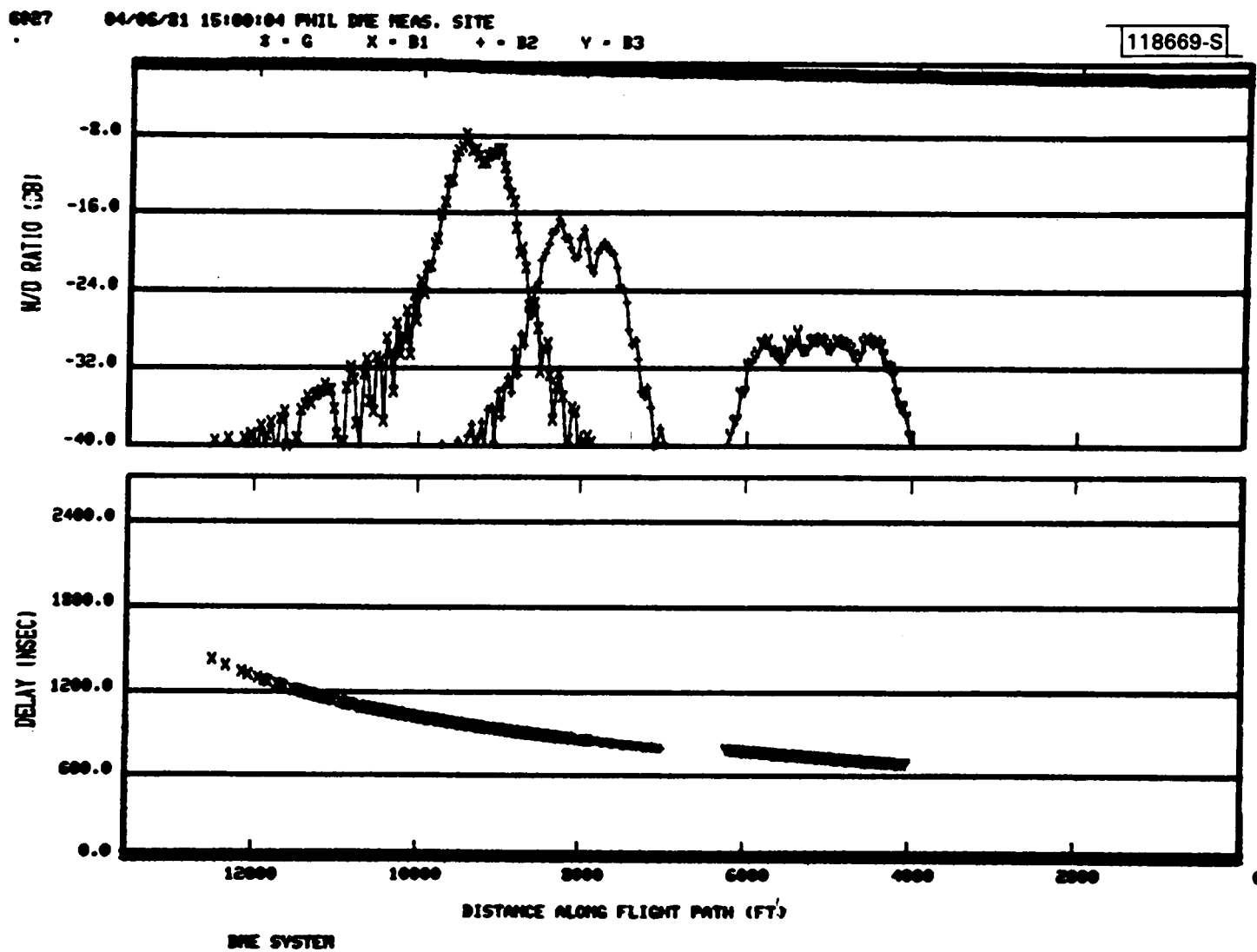
Fig.5-19. Computed multipath characteristics for PHL measurement scenario.
