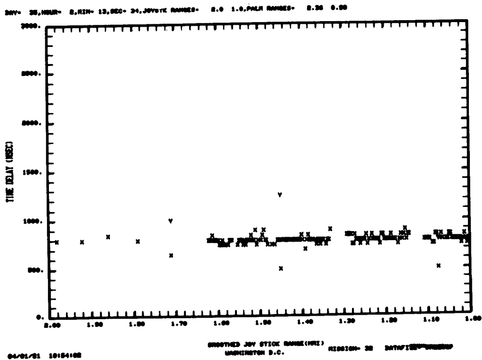
Fig.5-5(c). Summary results for 3° approach to DCA near threshold.
