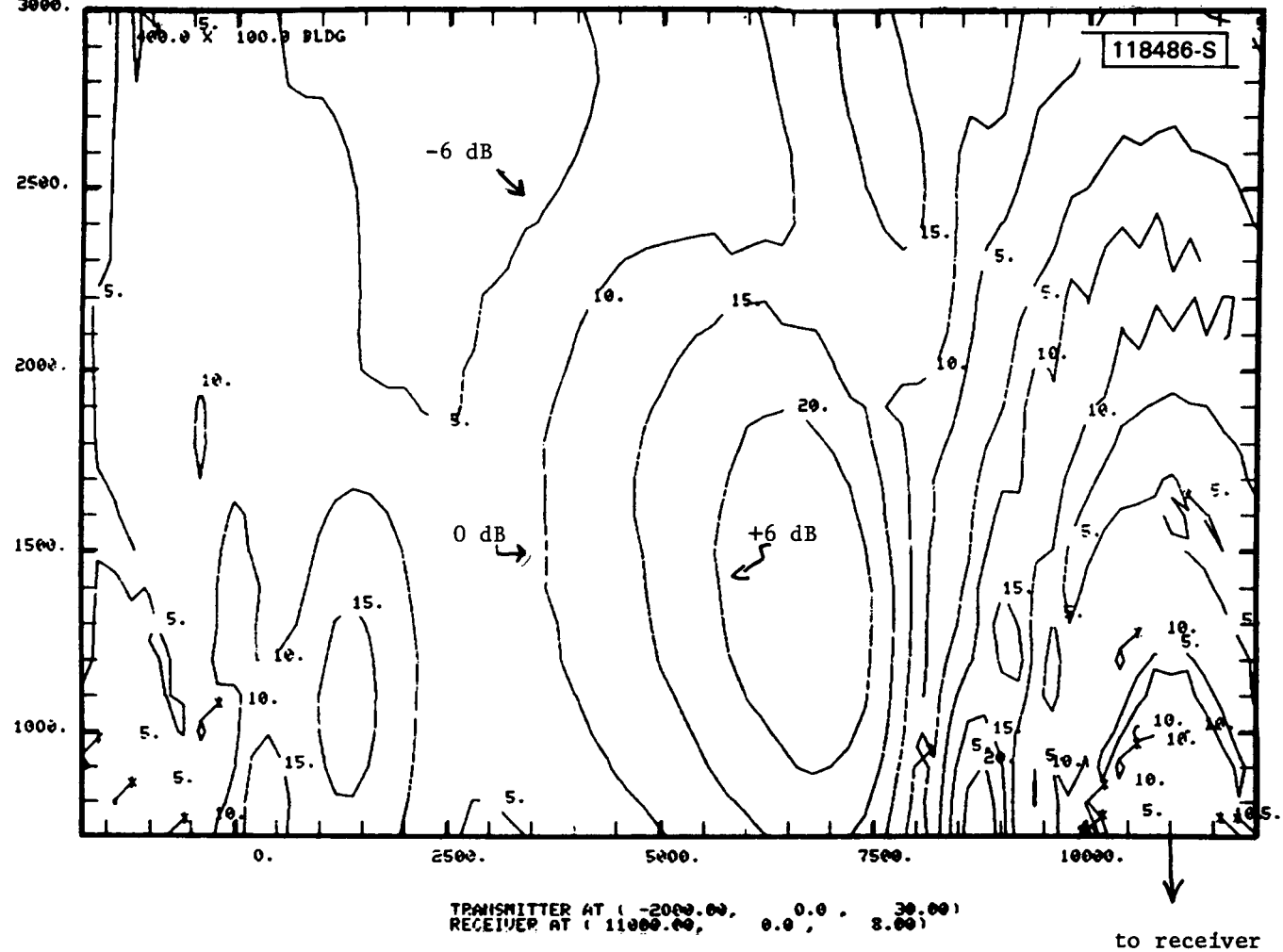
Fig.4-11(b). Effective L-band M/D ratio from large building for receiver near touchdown.
