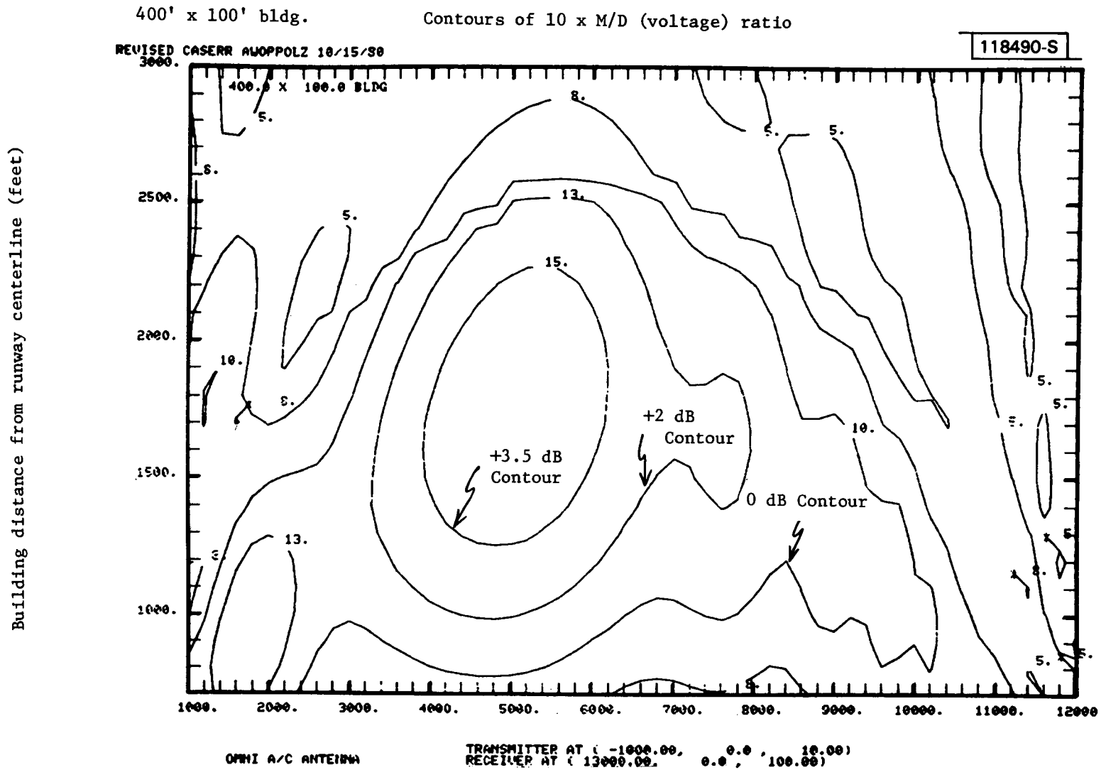
Fig.4-14. Effective M/D levels from large building with receiver near Cat II decision height.
