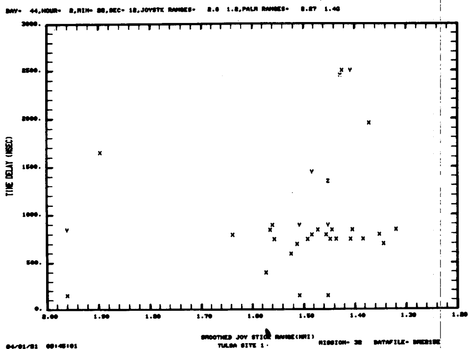
Fig.5-23(b). Tulsa site 1 data summary for 25 ft. threshold crossing height.
