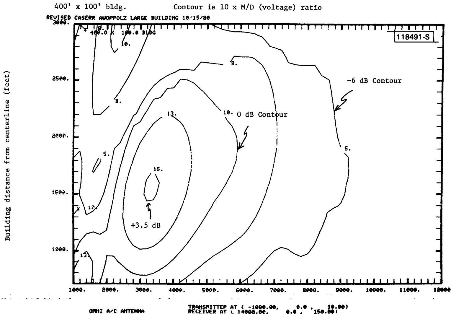
Fig.4-15. Effective M/D levels from large building with receiver between Cat I and Cat II decision heights.
