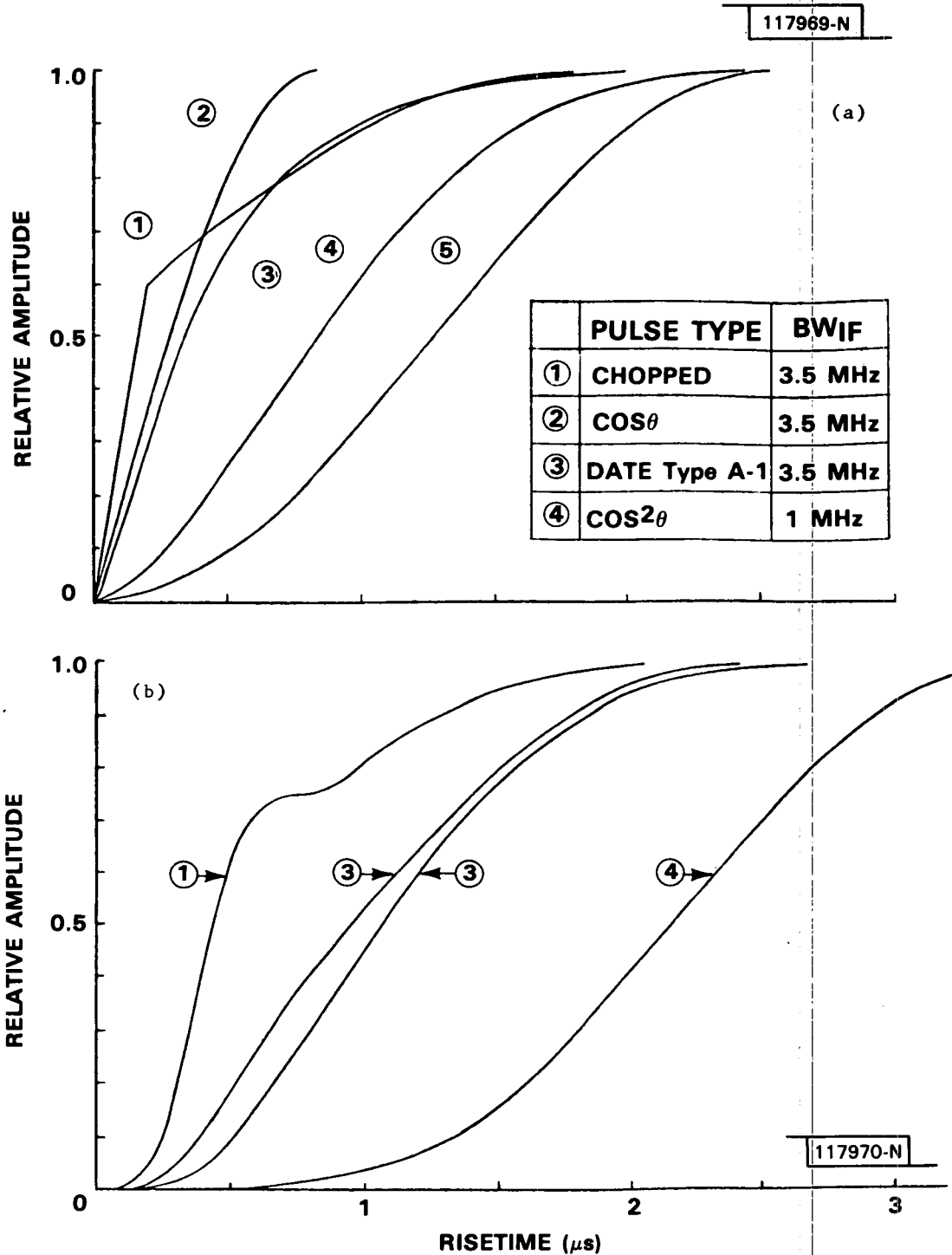
Fig.2-8. (a) Leading edge comparison of various proposed pulse shapes for air to ground (from [12]) and (b) leading edge characteristics of various proposed ground to air pulse shapes including IF filter effect (from [12]).
