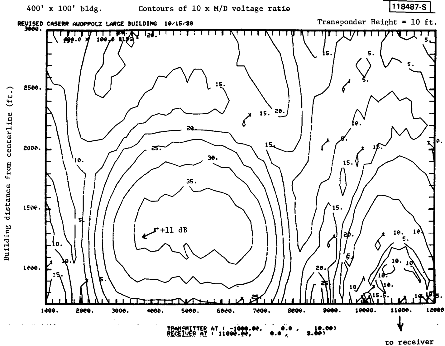
Fig.4-12(a). Effective L-band M/D level from large building for receiver near touchdown.
