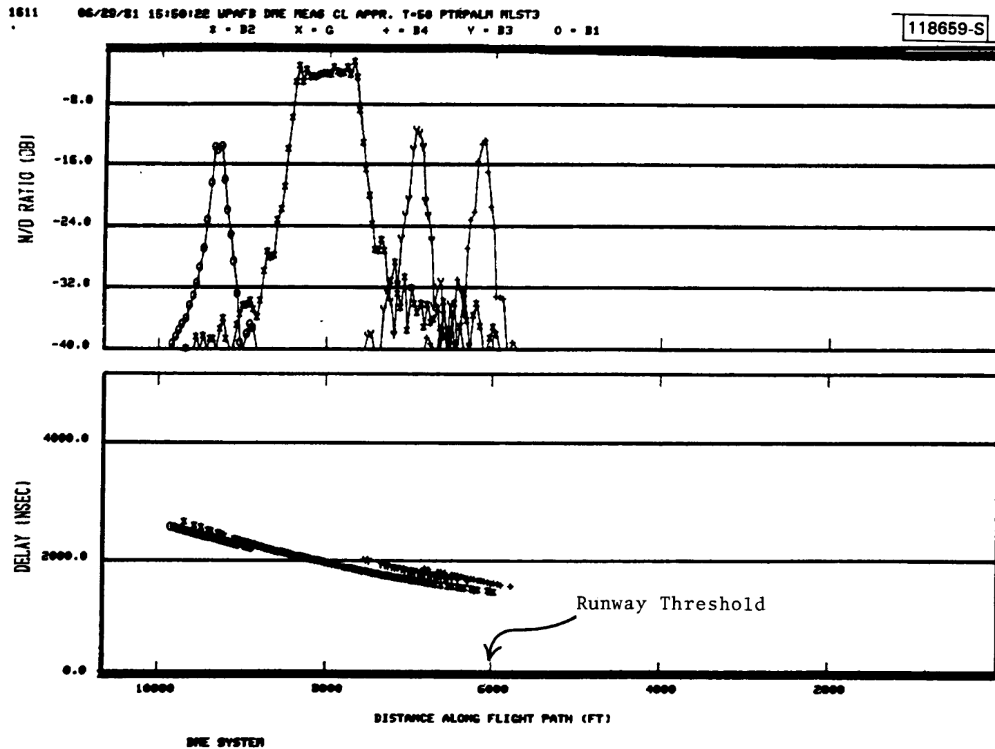
Fig.5-11. Computed DME multipath characteristics for WPAFB scenario.
