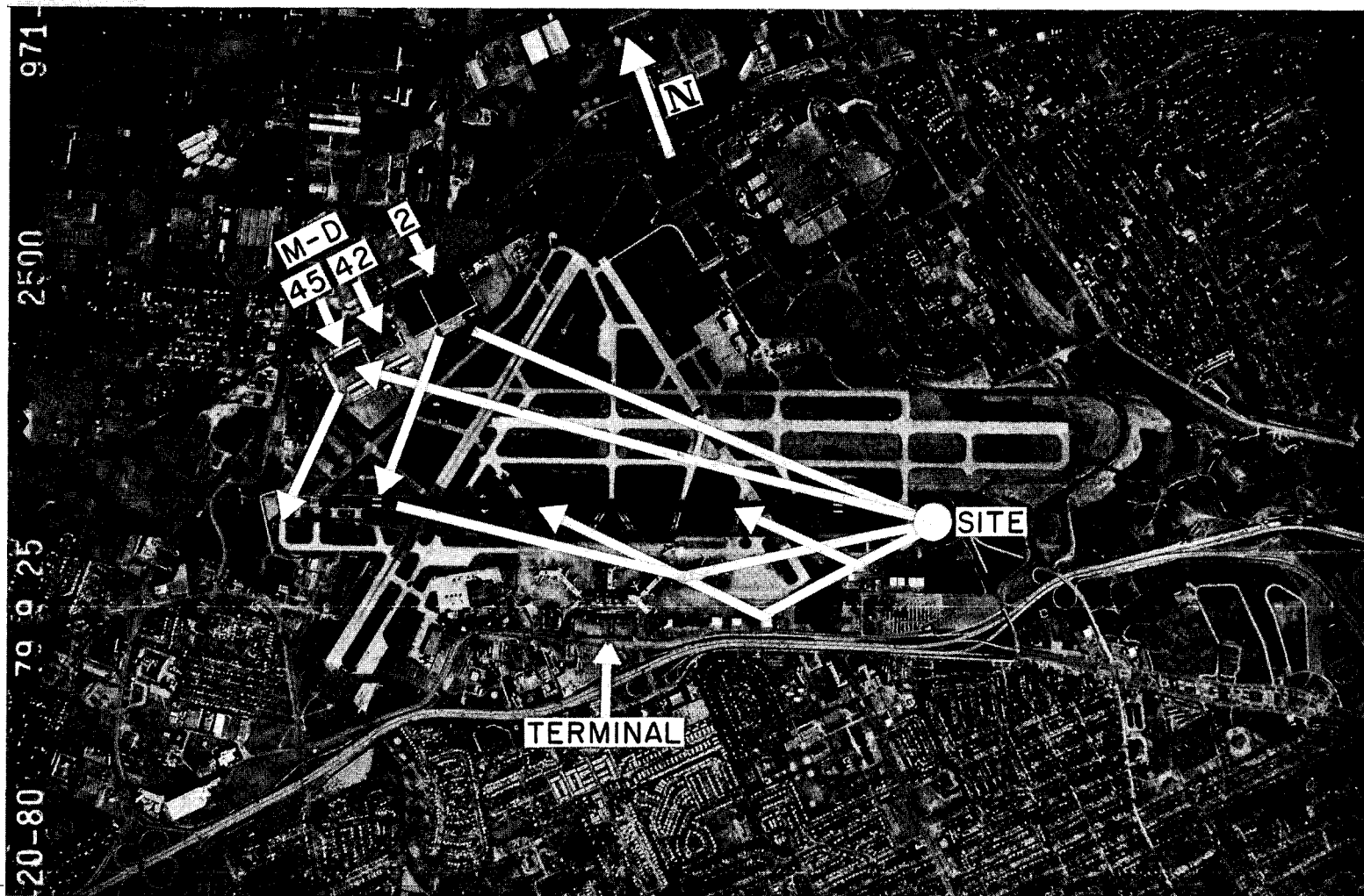
Fig.5-12. Lambert-St. Louis International, St. Louis, Missouri, showing azimuth reflection paths.
