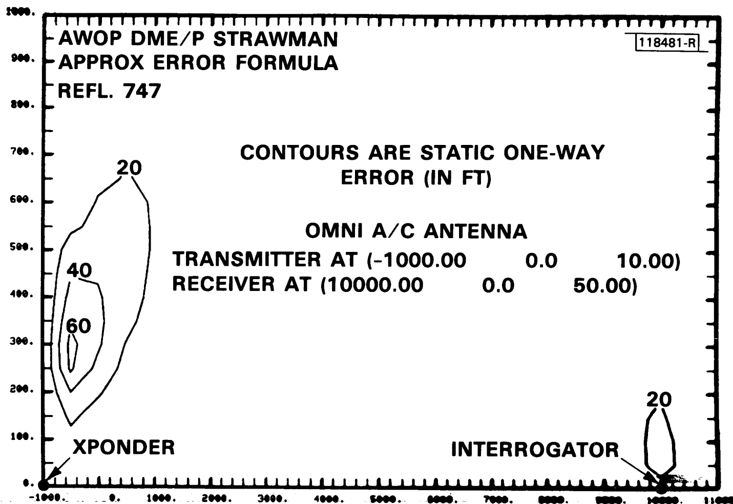
Fig.4-7. AWOP WG-M DME/P Strawman: B747 reflections at threshold.
