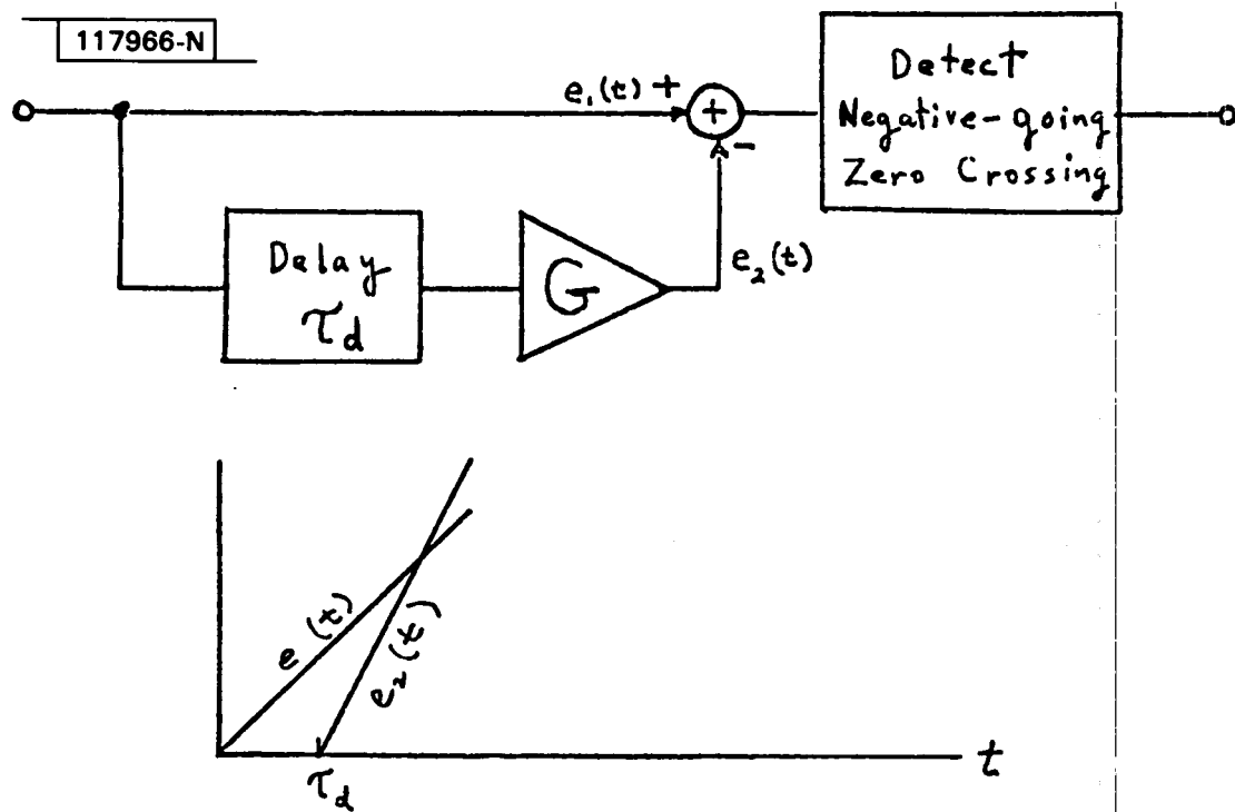
Fig.2-5. DME leading edge comparator circuit.
