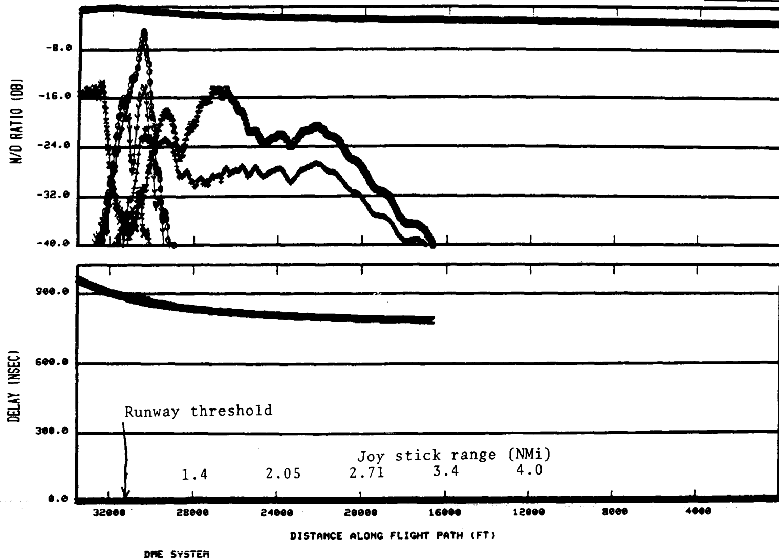
Fig.5-7. Computed multipath characteristics for DCA 3° approach scenario.
