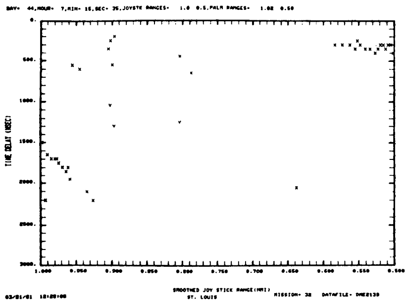
Fig.5-14(b). Data summary for St. Louis's approach with 50 ft. threshold height.
