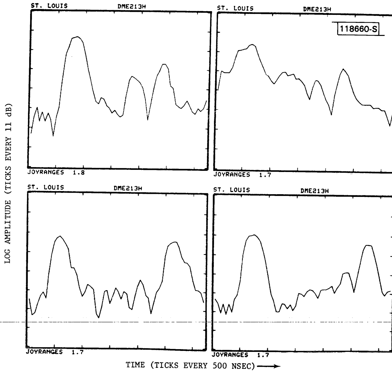
Fig.5-13. St. Louis waveforms at threshold (50 ft. AGL).
