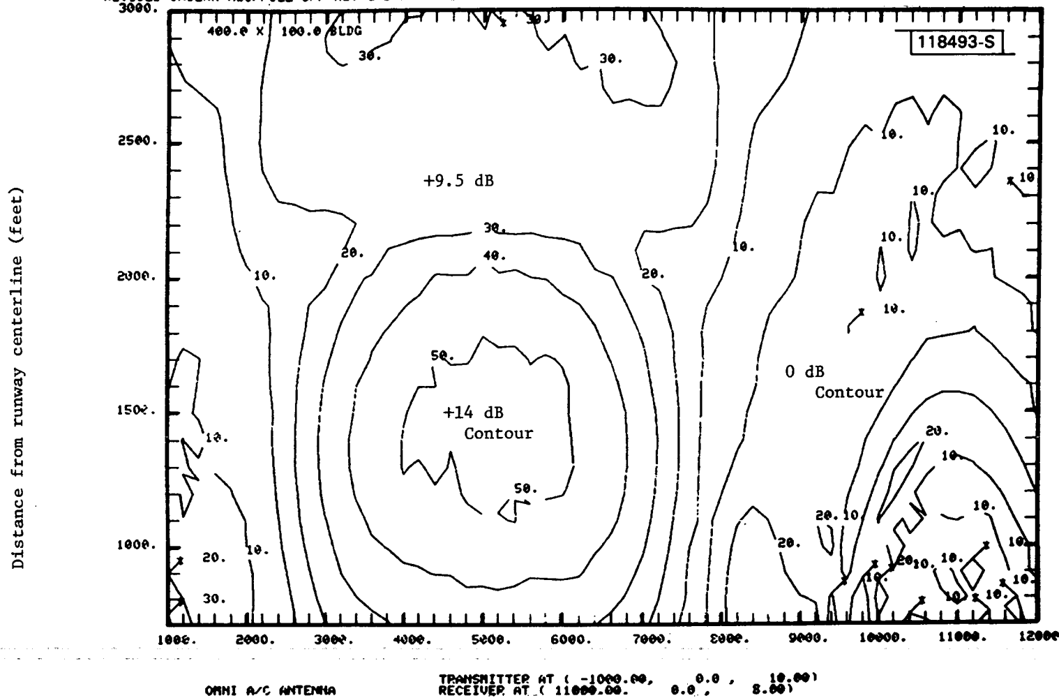
Fig.4-17. Effective M/D levels from large building with off runway terrain 3 feet below runway level when receiver is near touchdown.
