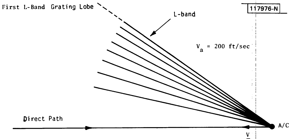
Fig.2-13. Multipath arrival directions for maximum motion averaging and first grating lobe.
