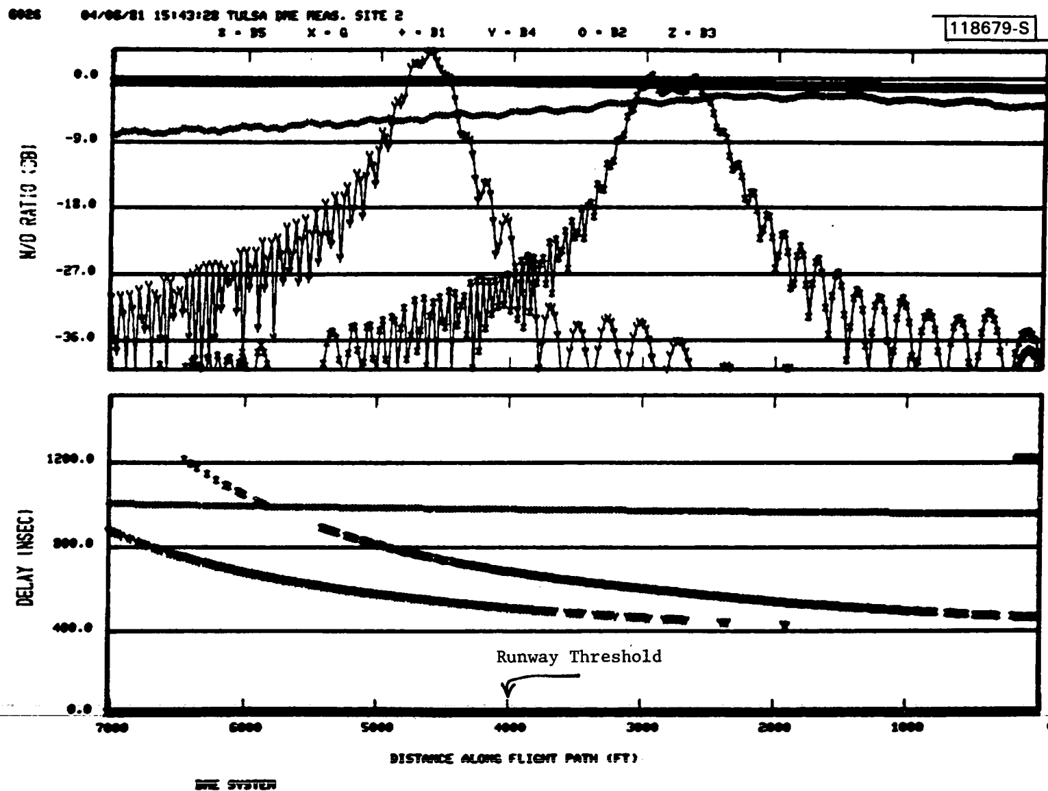
Fig.5-27. Computed DME multipath characteristics for simulation of Tulsa DME measurement site 2.
