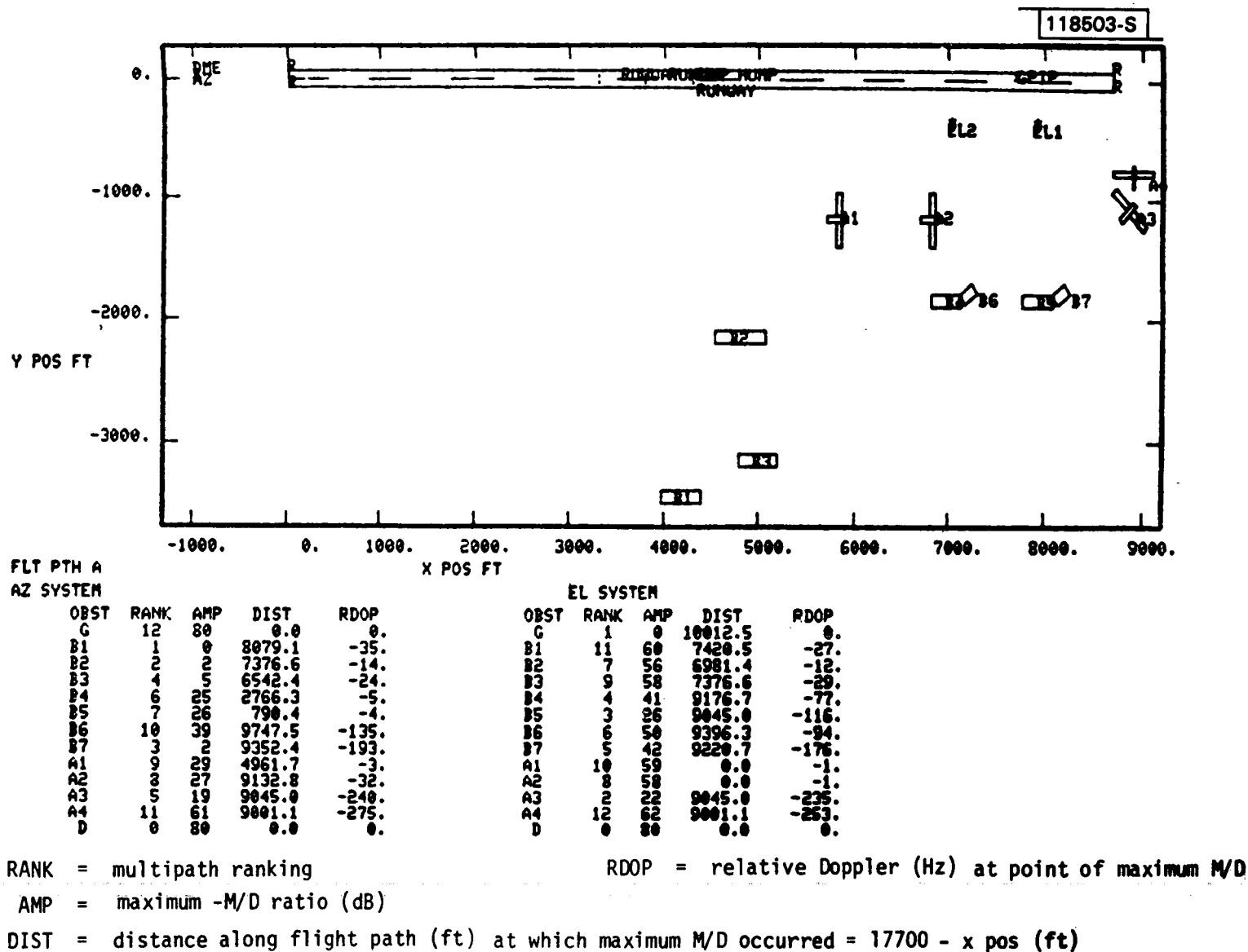
Fig.4-25. Airport map for WG-A scenario 2 for L-band carrier.
