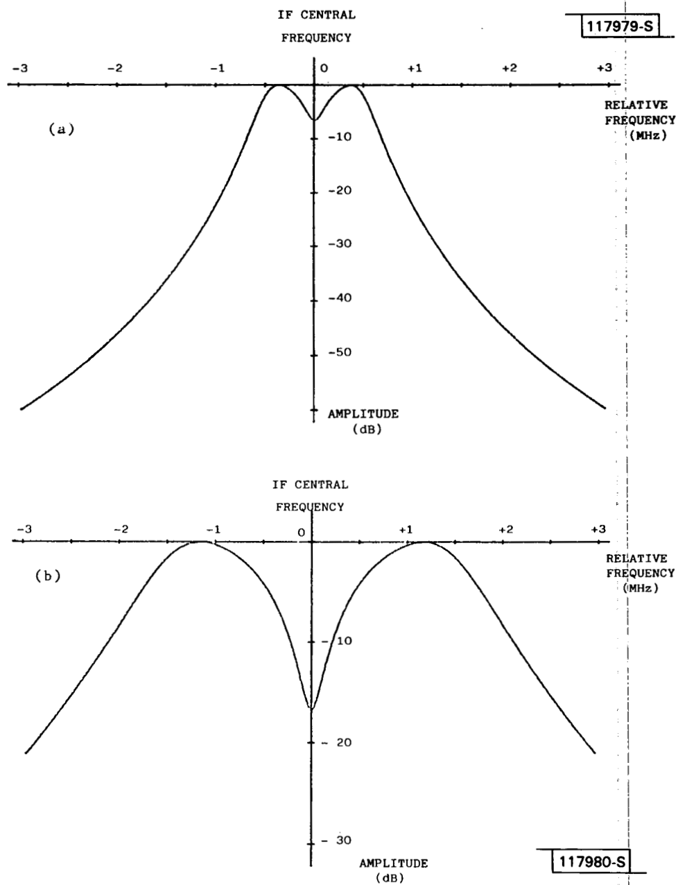
Fig.2-16. (a) Characteristic of the CTOL/STOL system receiver filter and (b) characteristic of the VTOL system receiver filter.
