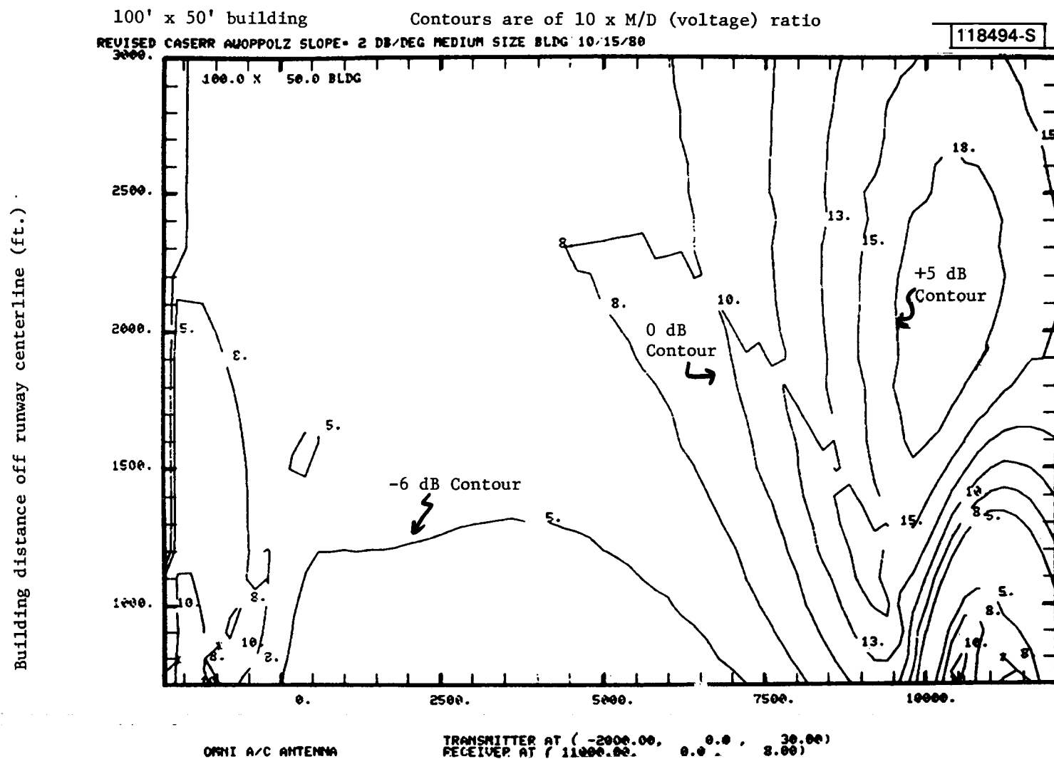
Fig.4-18. Effective M/D levels from medium size building with receiver near touchdown.
