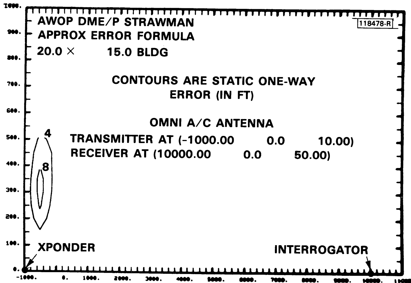
Fig.4-4. AWOP WG-M DME/P Strawman: "surface vehicle" reflections at threshold.
