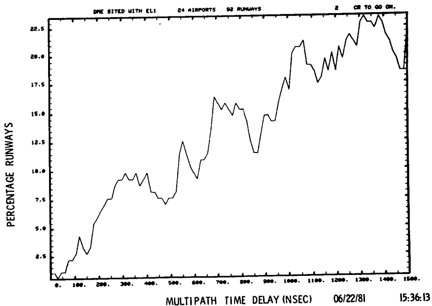
Fig.6-8. Multipath time delay distributions when DME/P is sited with MLS elevation antenna. Only buildings near runway threshold.
