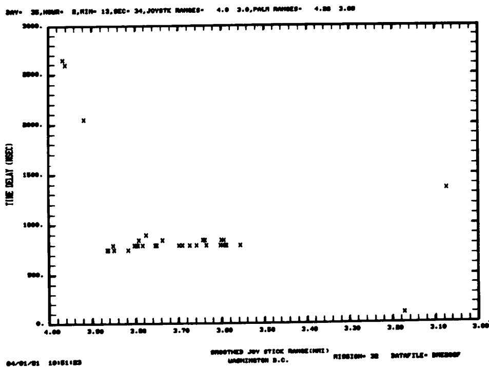
Fig.5-5(a). Summary results for 3° approach to DCA before threshold.
