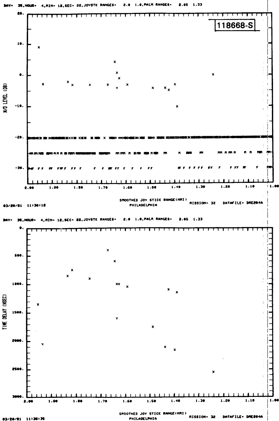
Fig.5-18(c). Summary results for flight profile 1 at Philadelphia.
