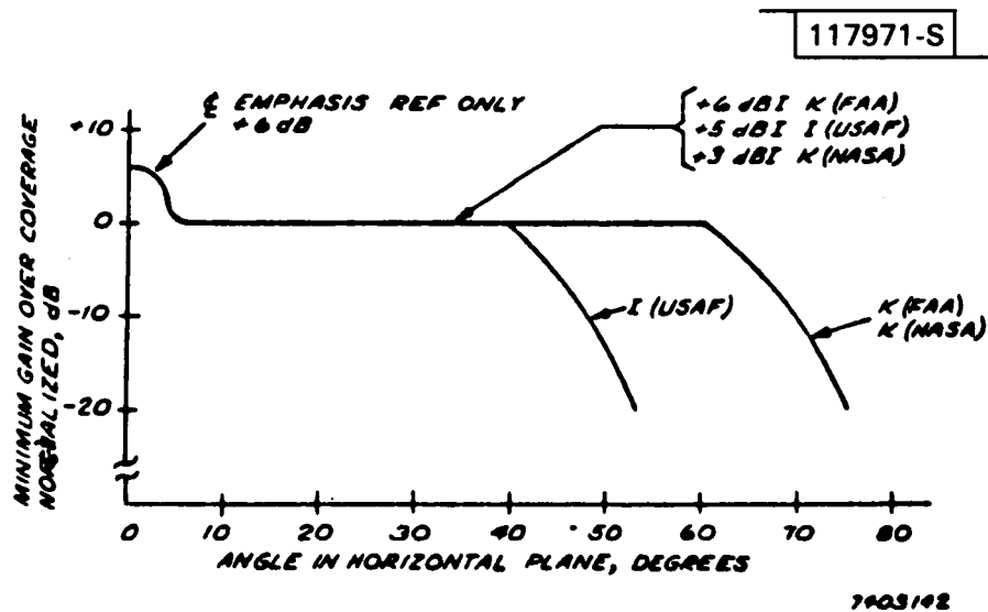
Fig.2-9. Hazeltine AZ antenna azimuth pattern showing centerline emphasis.
