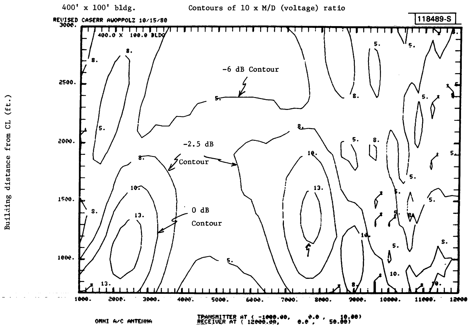
Fig.4-13. Effective M/D levels from large building with receiver at runway threshold.
