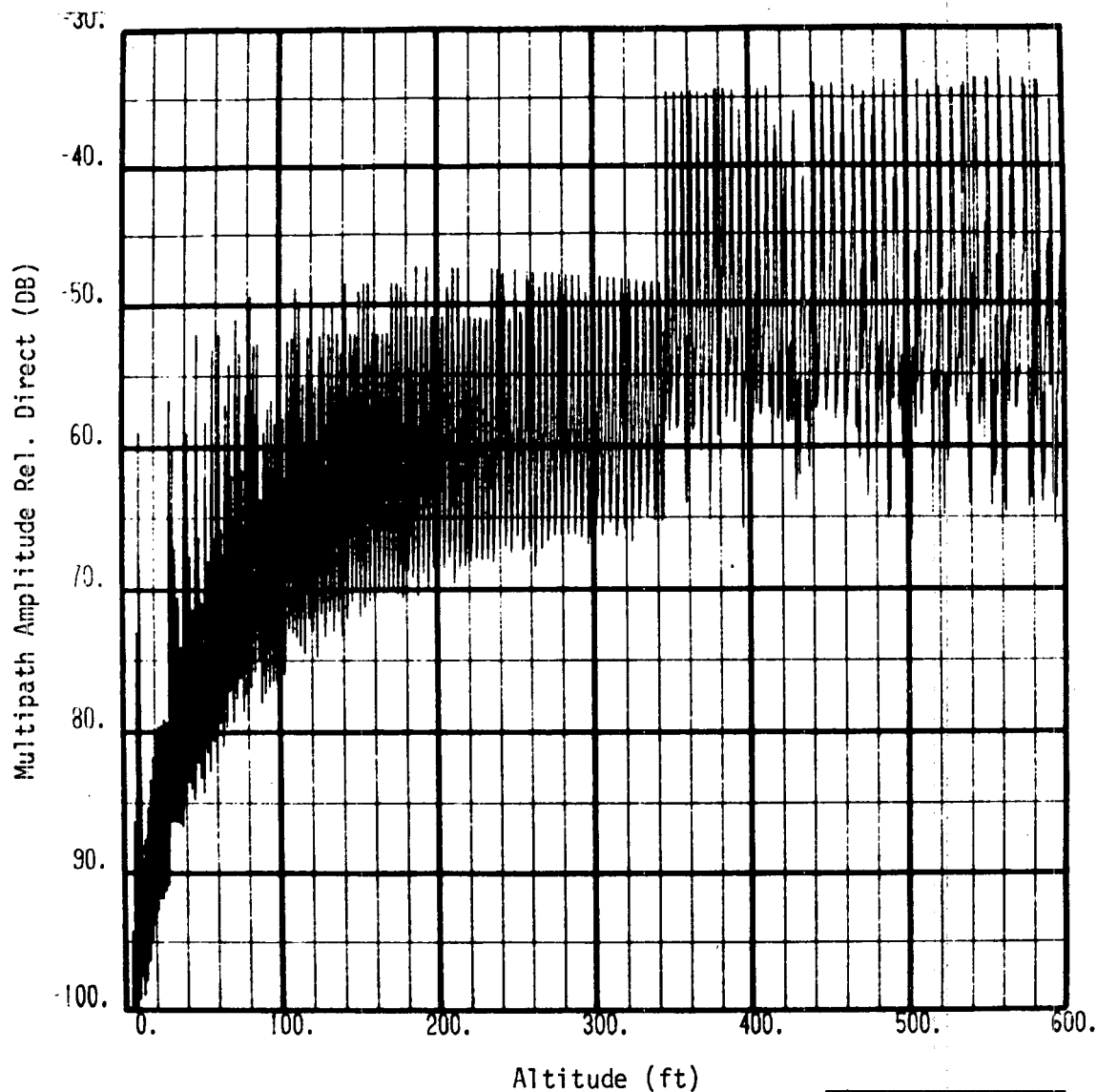
Fig. 2-9. Plot of amplitude, in dB, of diffuse ground scattering multipath component, with largest amplitude, vs altitude, for transmitter at (-500, 0, 8) , receiver on linear 3^\circ flight path between (9000, 0, 0) and (21000, 0, 600) , \sigma_h = 0.5' , \sigma_\ell = 1.0' .
