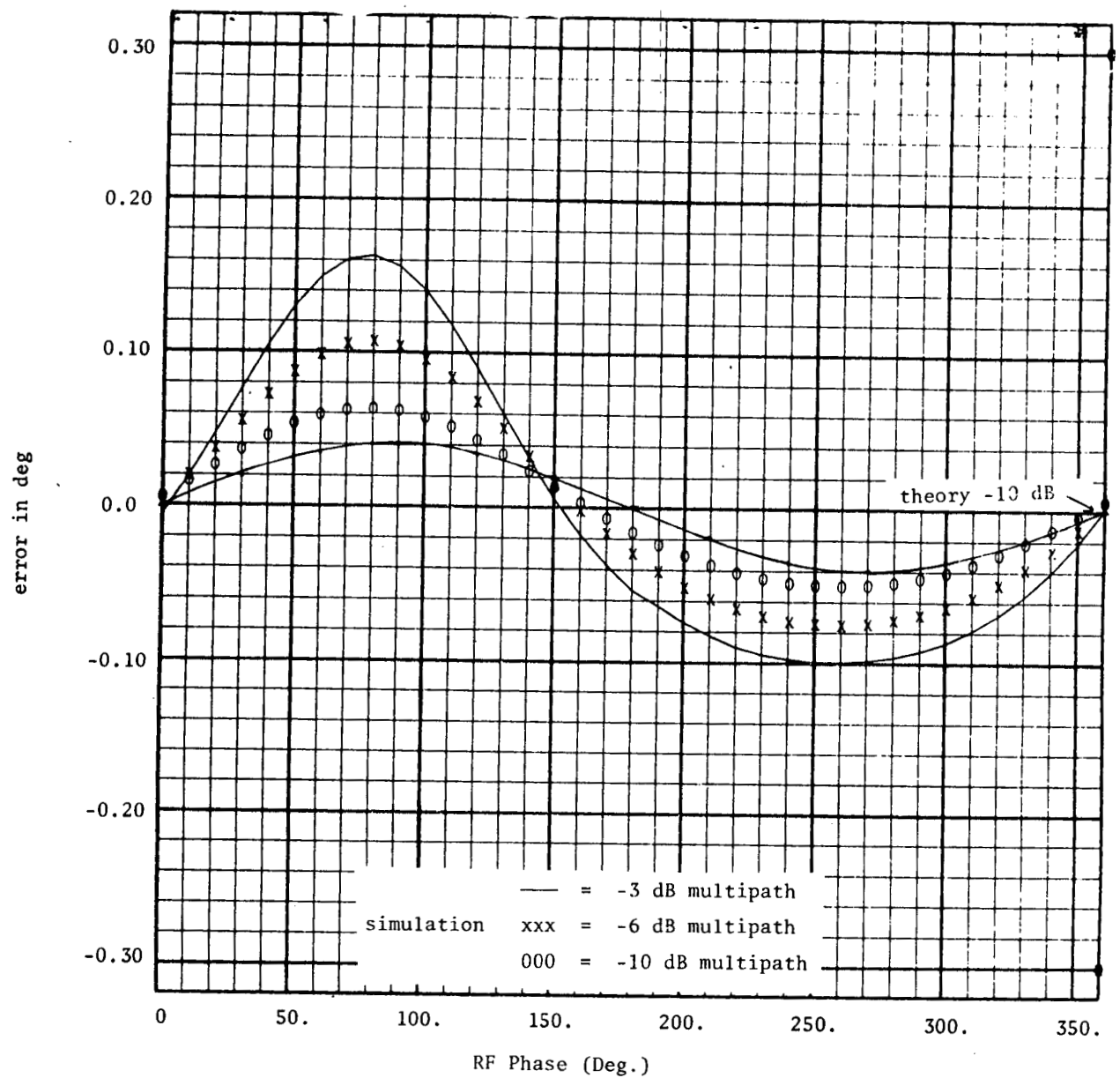
Fig. 6-10. Error vs RF phase, Doppler system with elevation filter, separation angle = 1.5^\circ .
