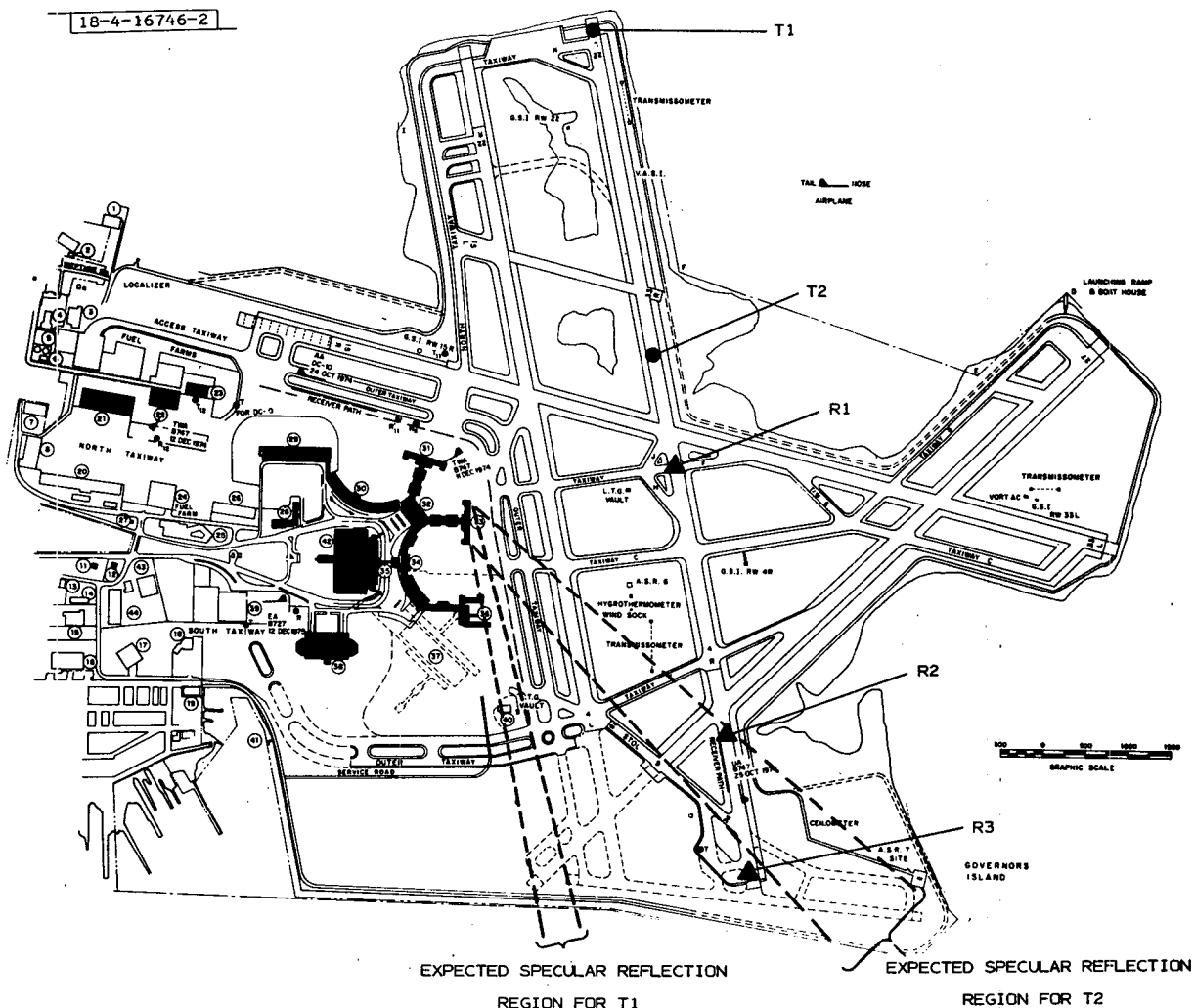
Fig. 3-2. Location of aircraft, transmitters, and receivers for airplane and terminal building multipath experiments at Logan International Airport.
