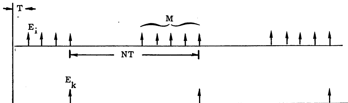
Fig. 5-1. Time sequence of measurement samples.
