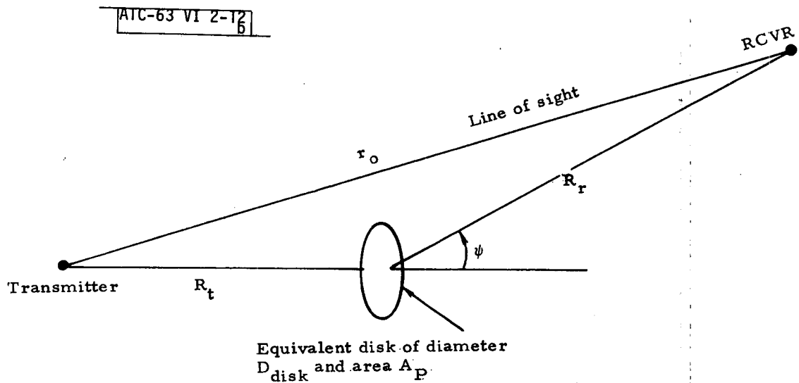
Fig. 2-12b. Disk model for obtaining shadowing effect due to aircraft approaching the line of sight.
