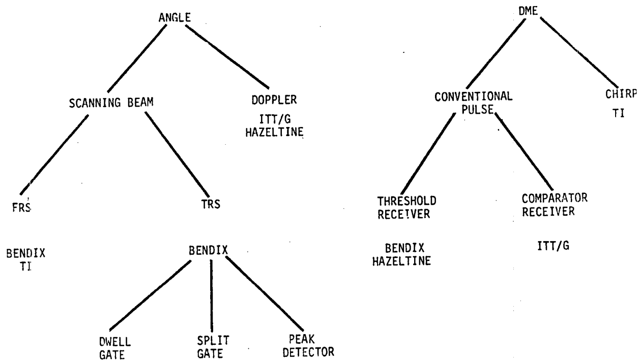
Fig. 4-1. MLS receiver models developed during first phase of Lincoln MLS program.
