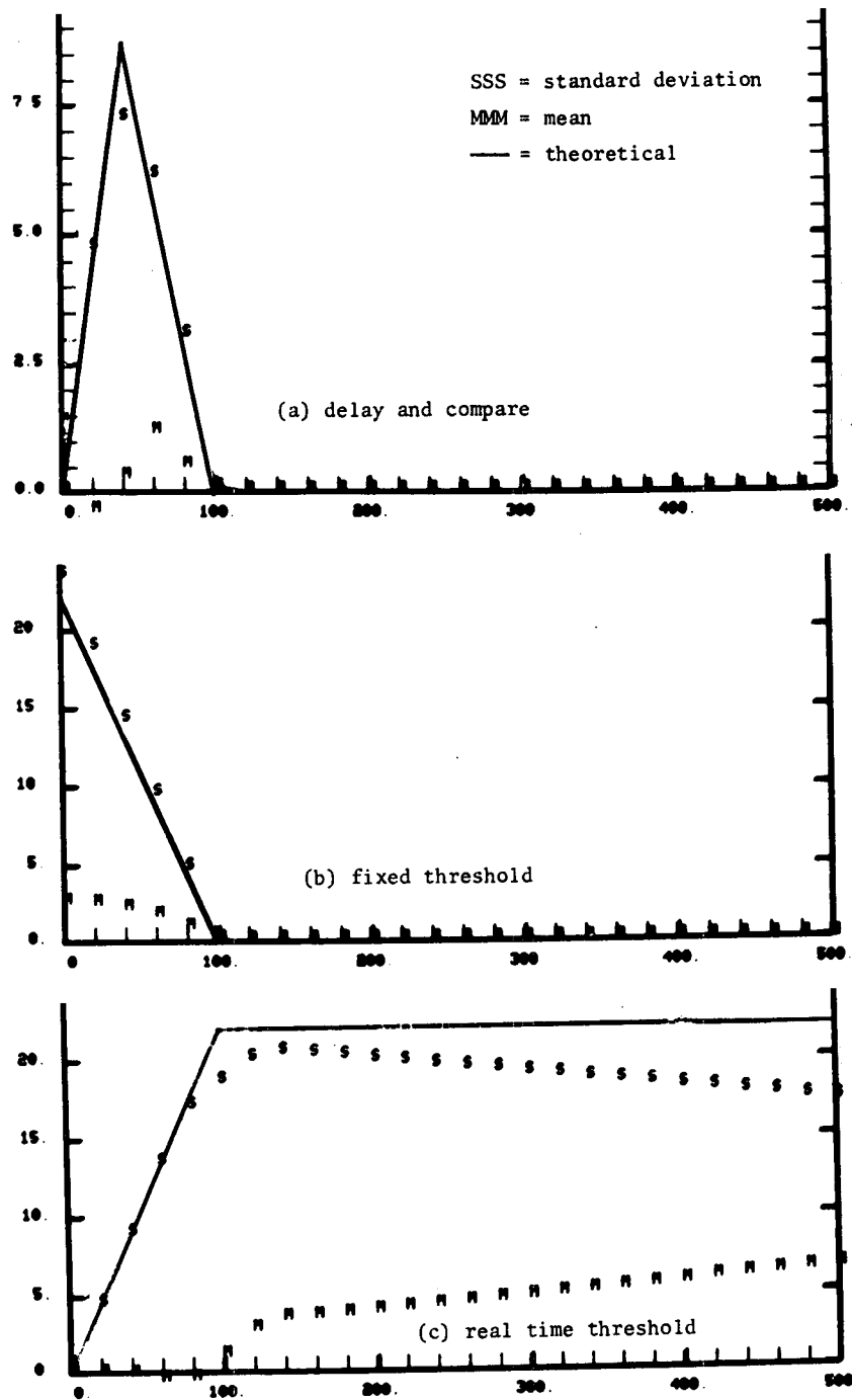
Fig. 6-27. DME error vs multipath time delay: comparison of simulation and theory for trapezoidal pulse.
