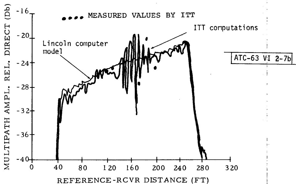
Fig. 2-7b. Comparison of computer simulation results with ITT computations and field data.
