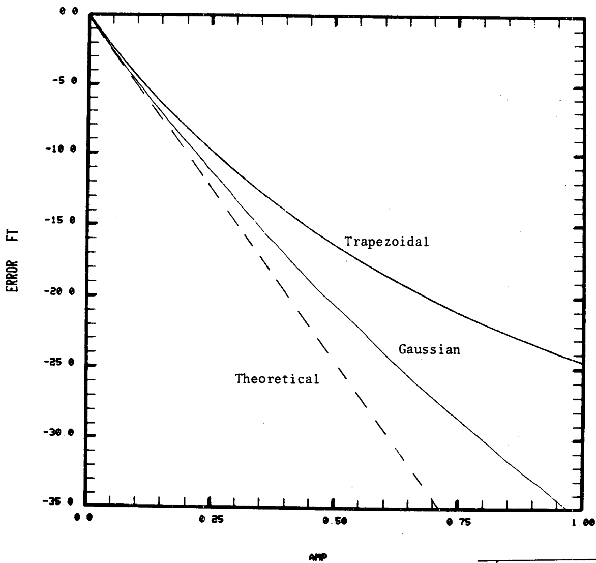
Fig. 6-20. DME error vs multipath amplitude-fixed thresholding.
