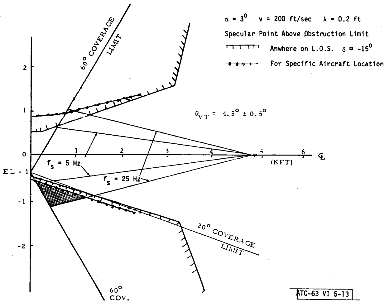
Fig. 5-13. Reflector location diagram.
