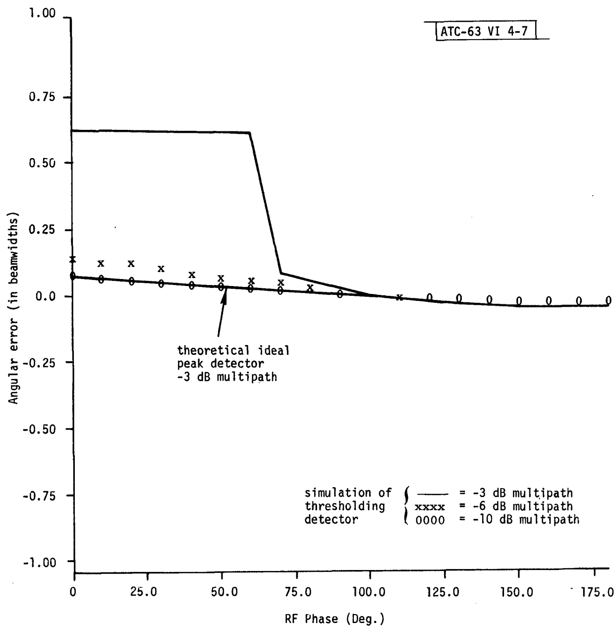
Fig. 4-7. Error vs RF phase, time-reference scanning beam system, separation angle = 1.5^\circ .
