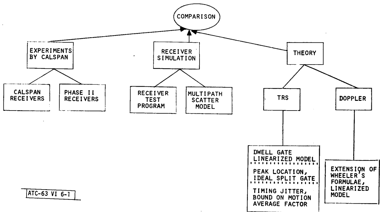
Fig. 6-1. Elements of angle receiver validation process.
