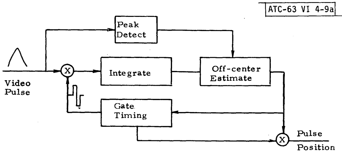
Fig. 4-9a. Split-gate multiply and integrate
