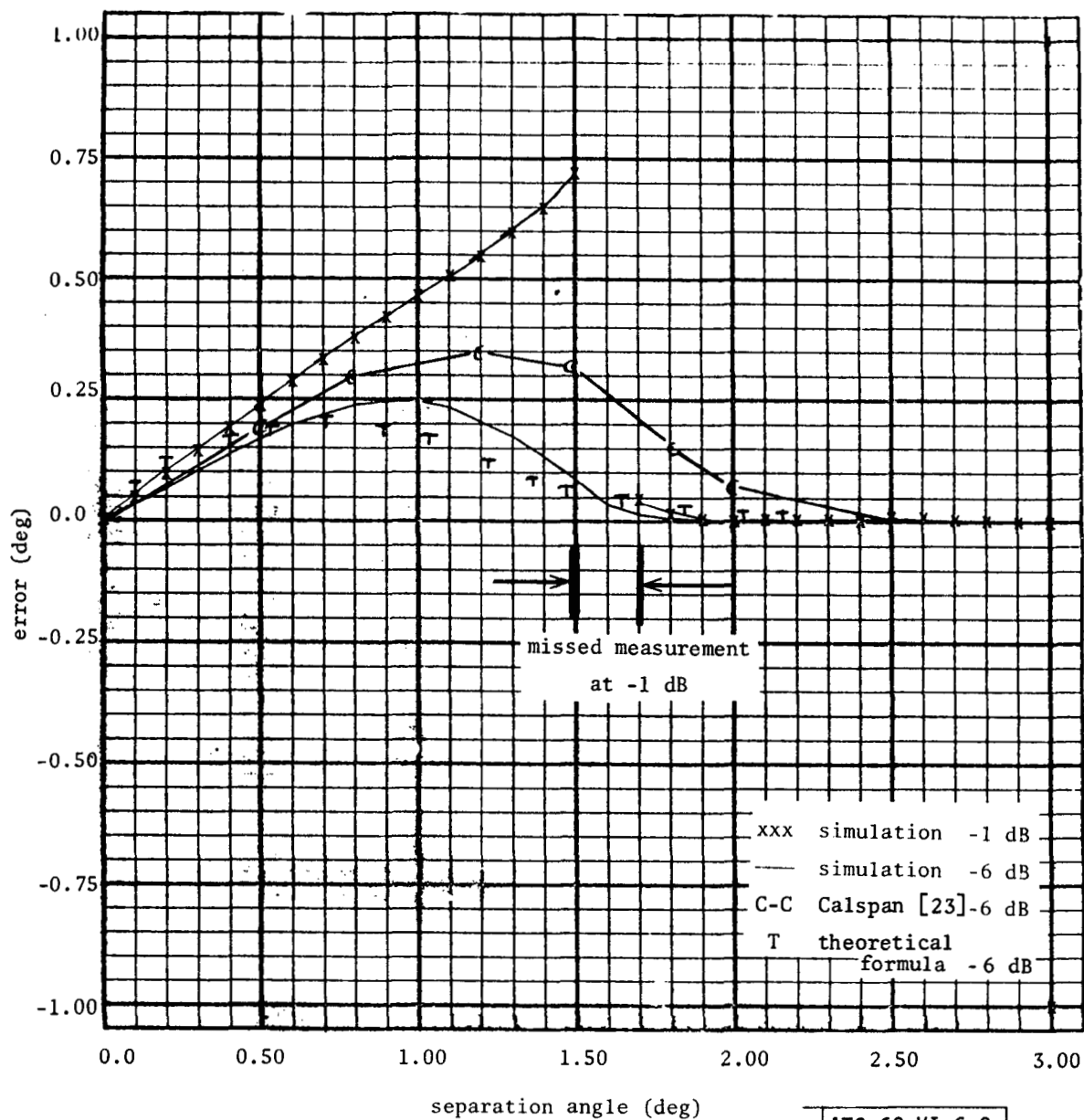
Fig. 6-3. Error vs separation angle, Bendix scanning beam system, multipath phase 0^\circ .
