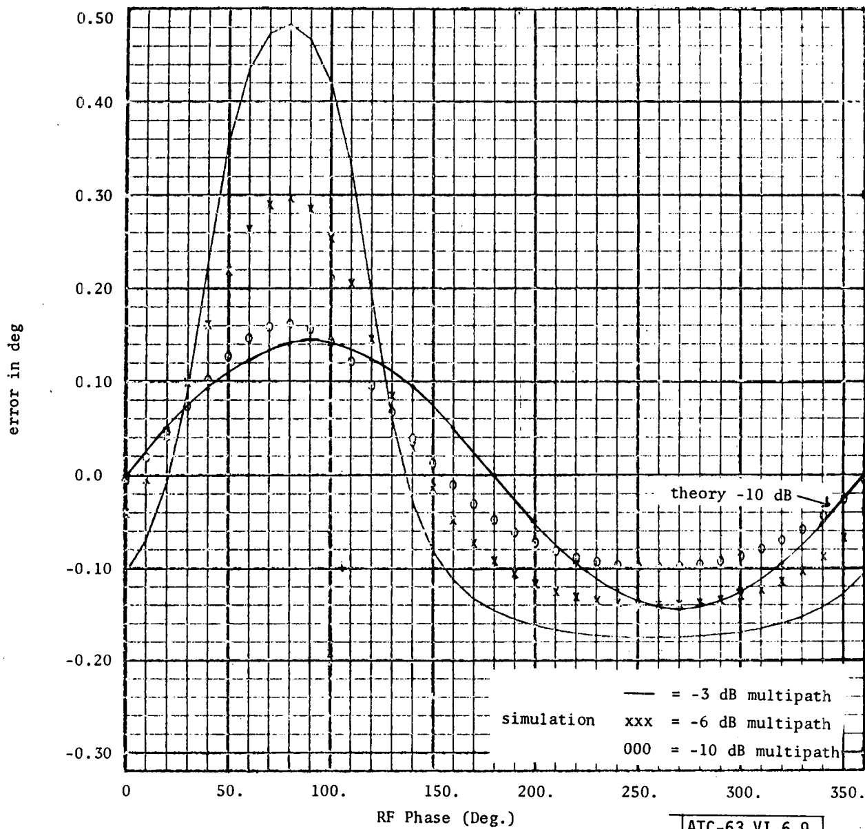
Fig. 6-9. Error vs RF phase, Doppler system without filter, separation angle = 1.5^\circ .
