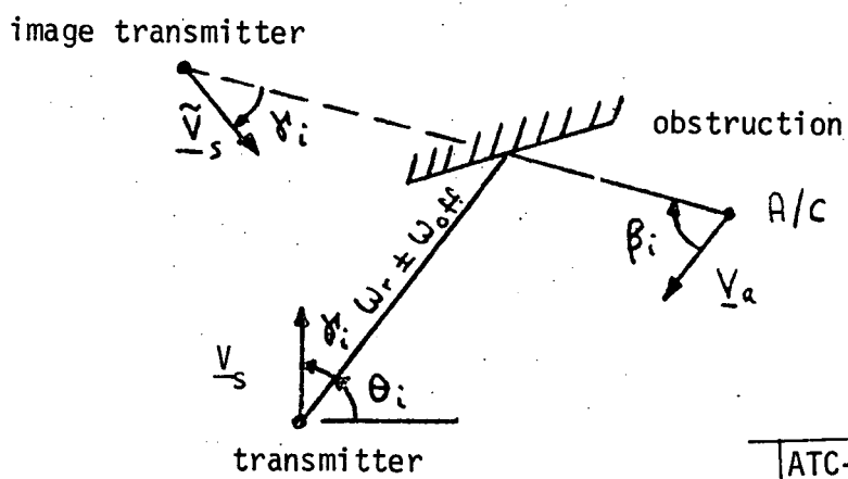
Fig. 4-11. Geometry for received angle frequency calculation.
