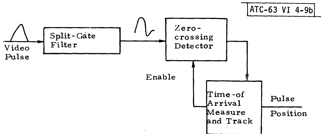
Fig. 4-9b. Split-gate convolution.
