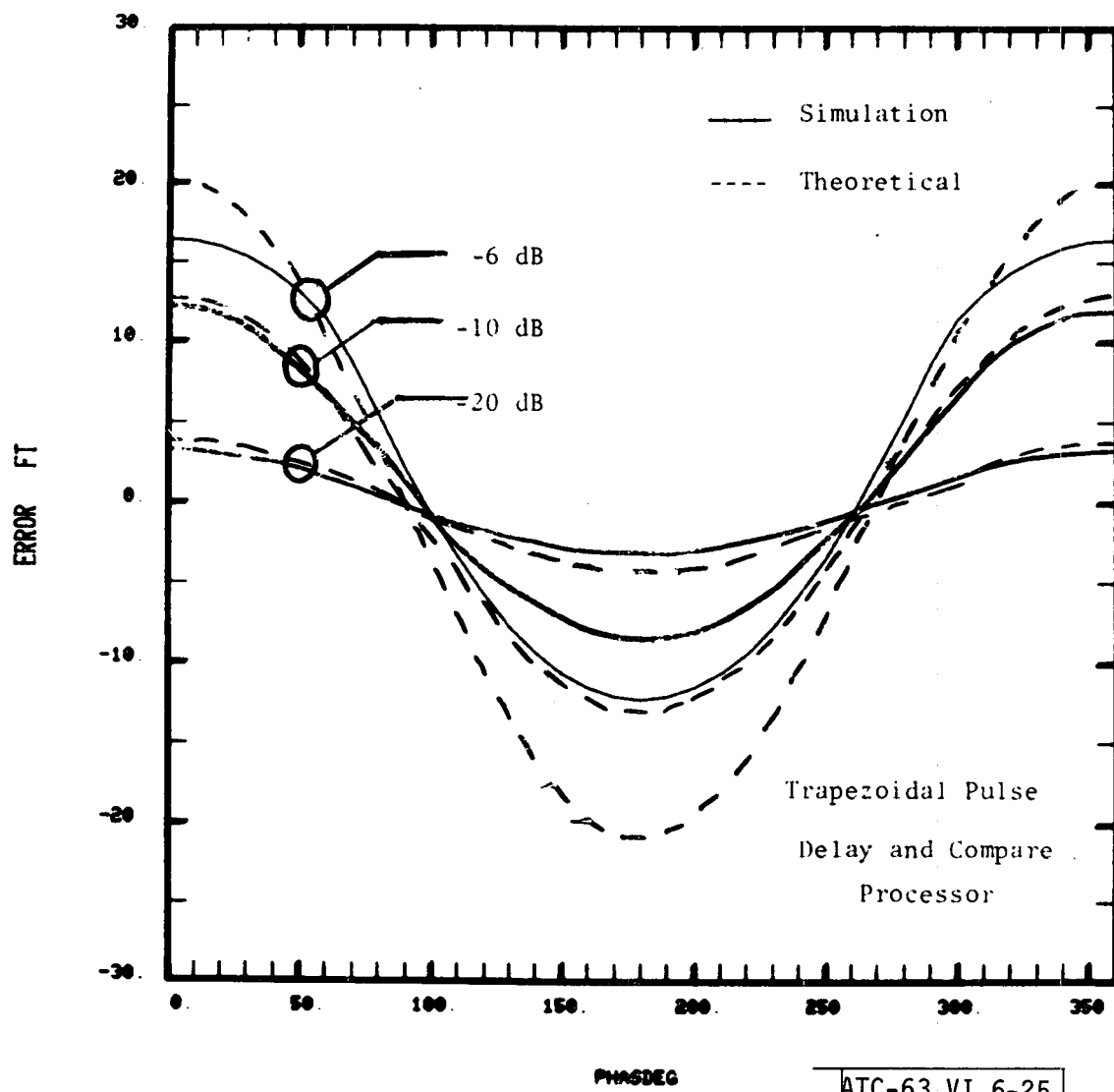
Fig. 6-25. DME error vs multipath phase.
