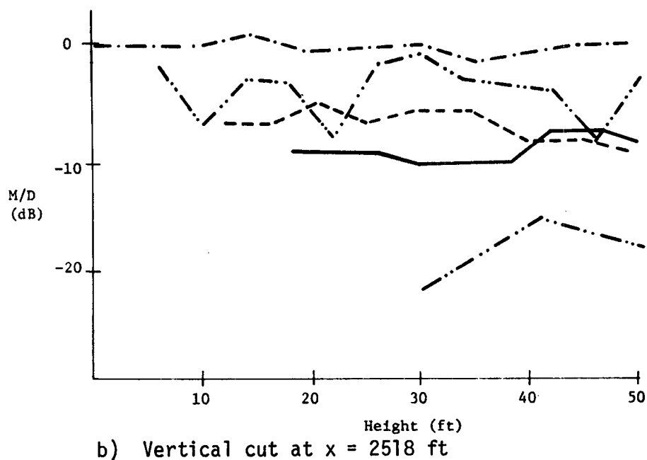
Fig. 3-17. Test 7. Elevation -2 at threshold; horizontal and vertical cuts.
