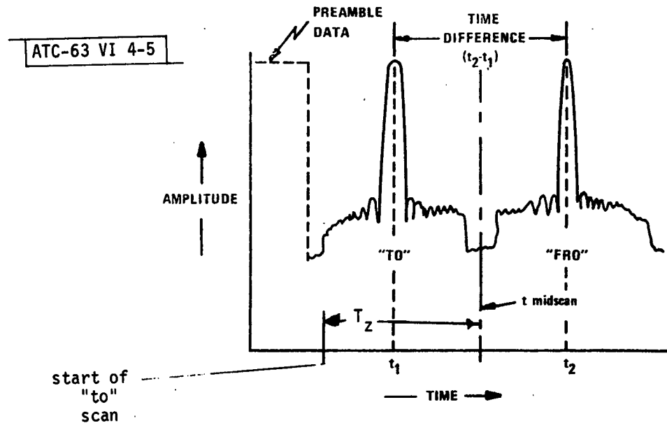
(a) Typical Pulses Received by TRS3 Receiver as Beam Scans TO and FRO
