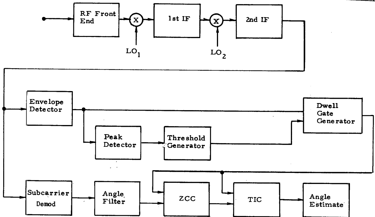
Fig. 4-3. Bendix/Bell FRS angle processing receiver.
