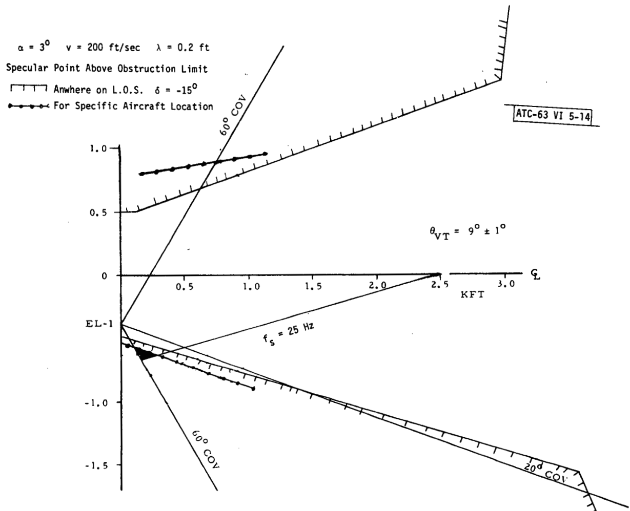
Fig. 5-14. Reflector rotation diagram.
