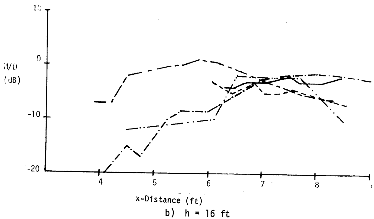
Fig. 3-13. Test 2. Azimuth at threshold; horizontal cuts.
