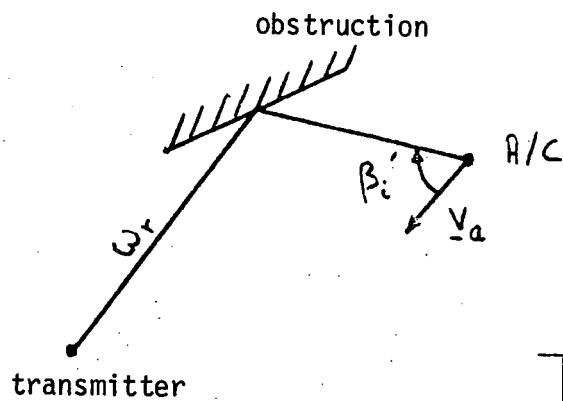
Fig. 4-10. Geometry for received reference frequency calculation.
